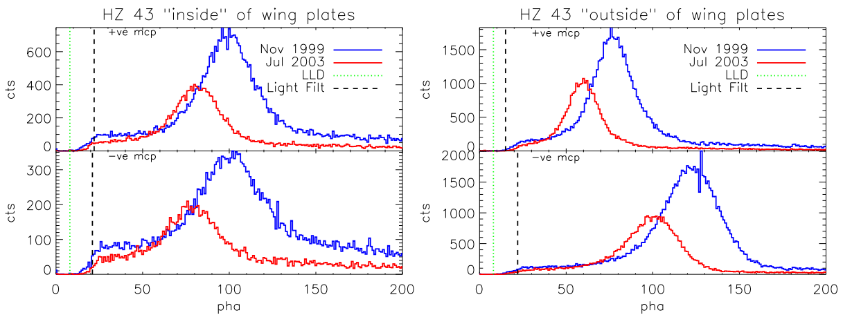
Figure 16. HZ 43 wing plate PHA distributions for November 1999 and July 2003 observations, and the \ll 1\% impact of the LLD and light PI filter cut-offs. Note: total counts vary in accordance with differing exposure times per observation.
