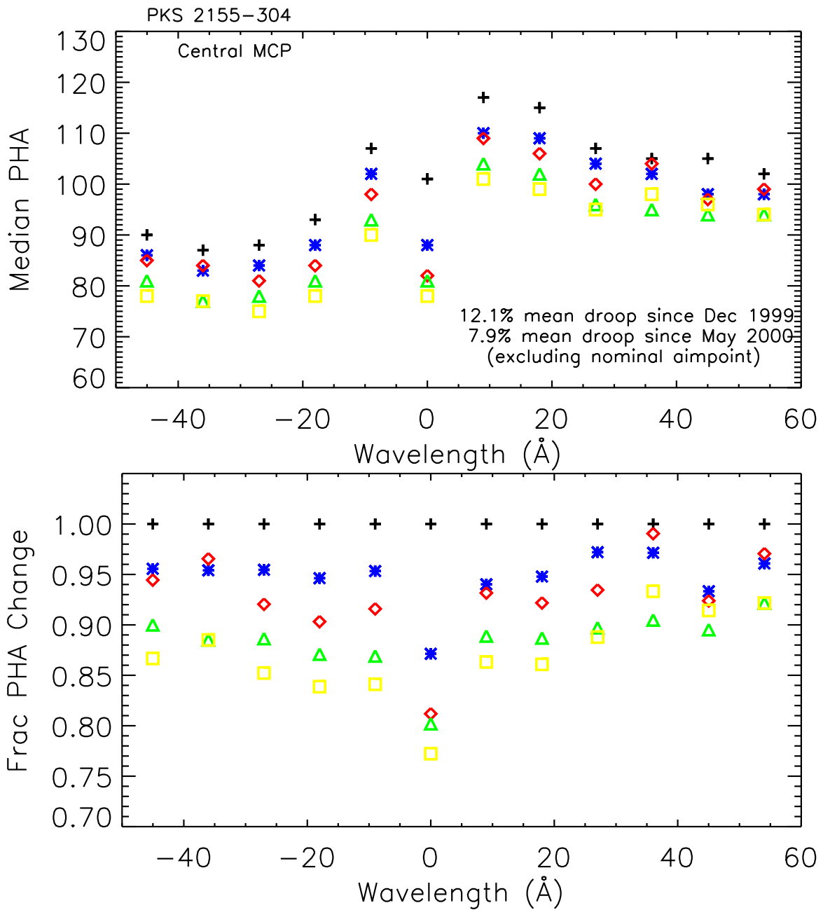
Figure 11. PKS 2155-304 median PHA evolution for the 11 dispersion bins (5 negative, 6 positive) on the central MCP. Aimpoint data plotted for comparison. Note the depression at 0th order (aimpoint). Bottom plot normalized to ObsID 331.
