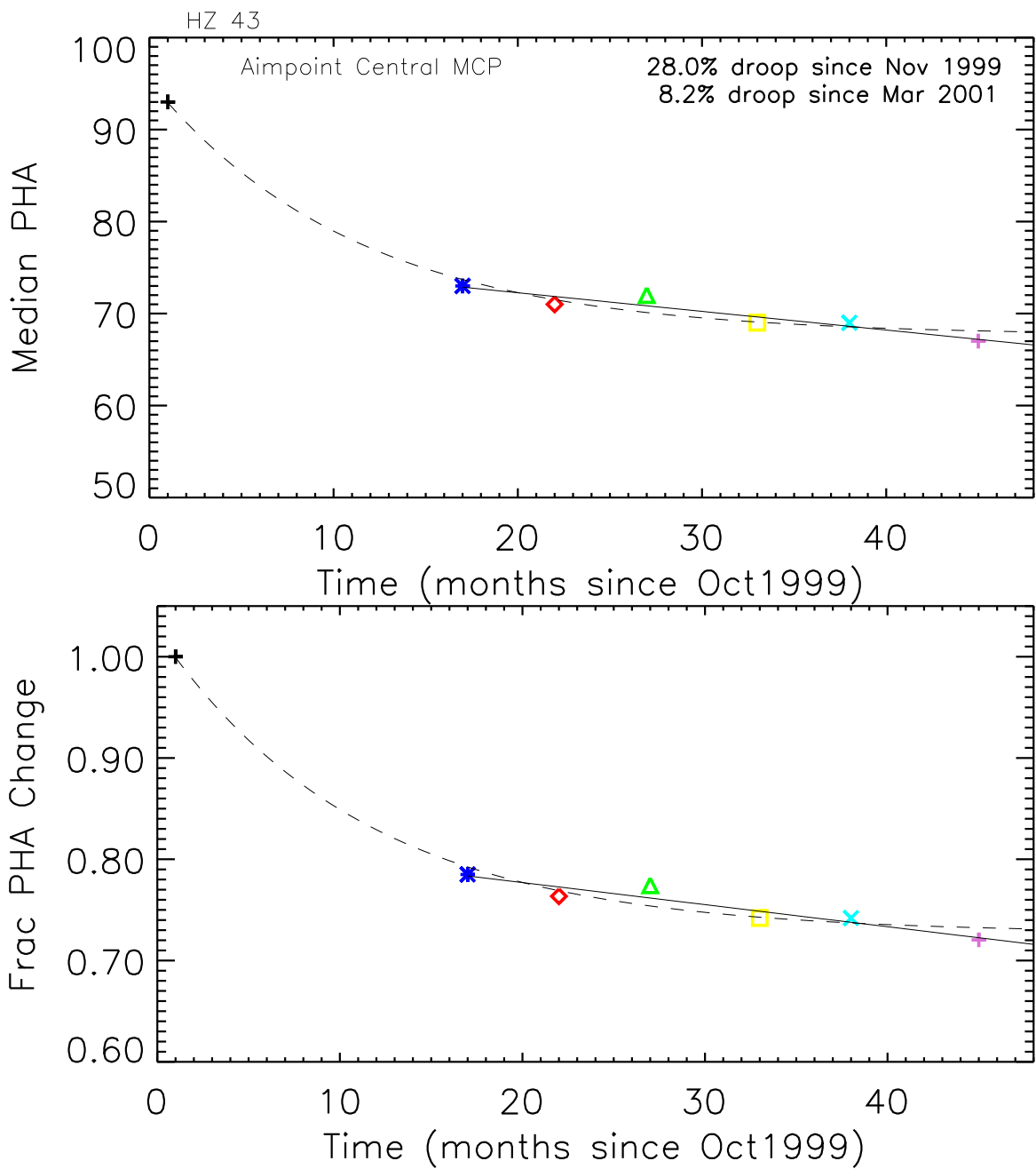
Figure 3. HZ 43 aimpoint median PHA evolution, with exponential (dashed curve) and linear (solid line) fits (see text). Bottom plot normalized to the first observation, ObsID 59.
