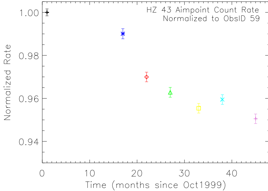
Figure 14. Evidence for QE degradation? HZ 43 aimpoint count rate evolution shows downward trend. Normalized to first observation, ObsID 59. Error bars represent statistical error of each observation only.
