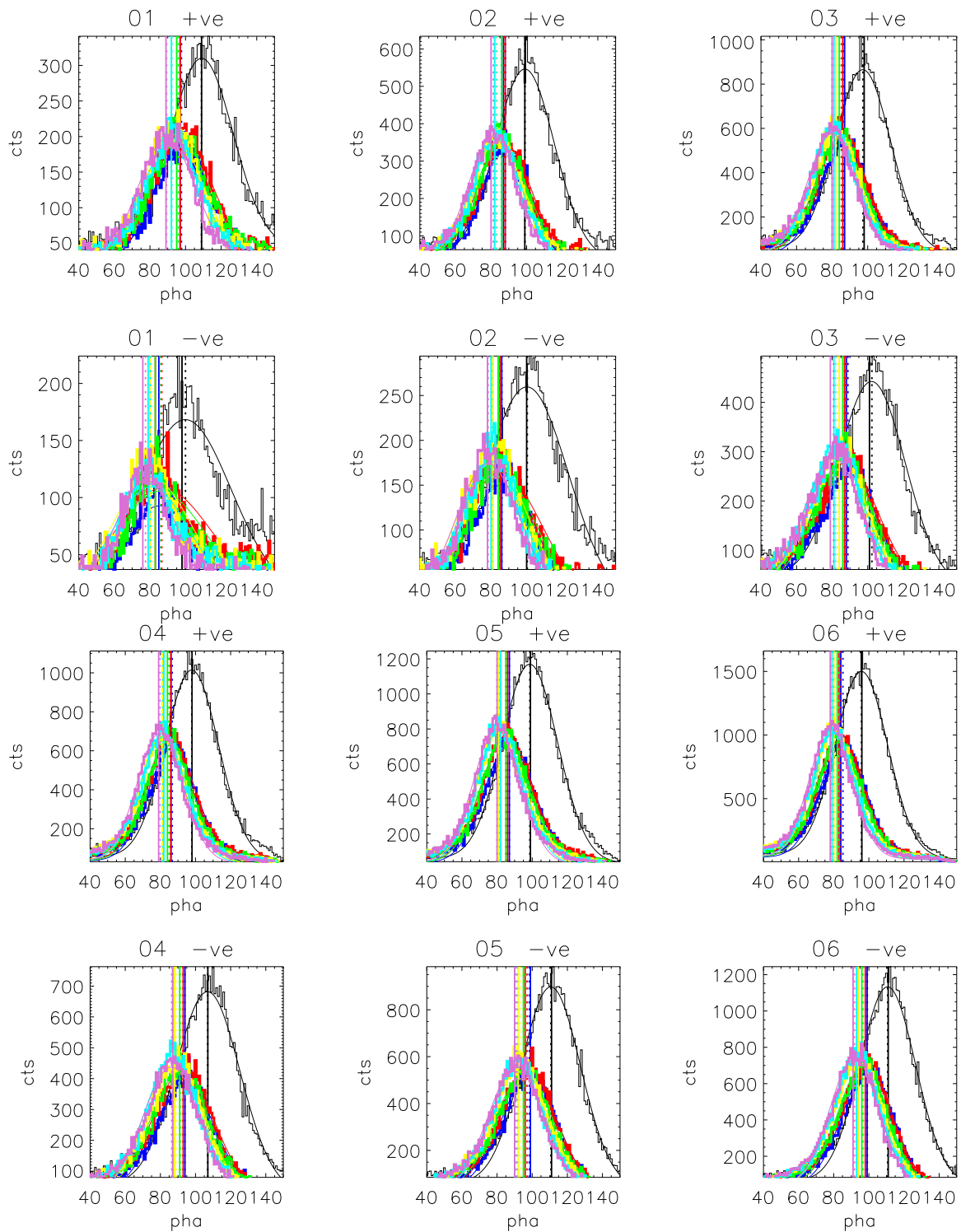
Figure 7. HZ 43 wing MCP PHA distributions. Solid vertical lines mark the median PHA. Gaussian fits overplotted. Bin numbers increase from center outward on MCPs. Positive and negative MCP bins plotted on alternating rows to facilitate comparison. Bins 01–06.
