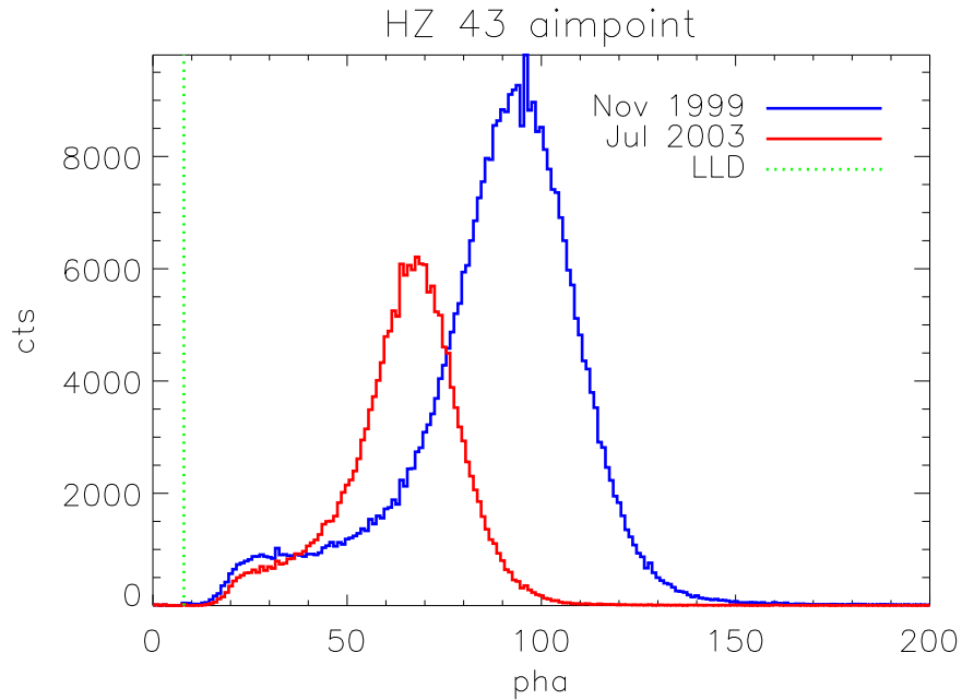
Figure 15. HZ 43 aimpoint PHA distribution for November 1999 (first) and July 2003 (most recent) observations, and the \ll 1\% impact of the LLD.
