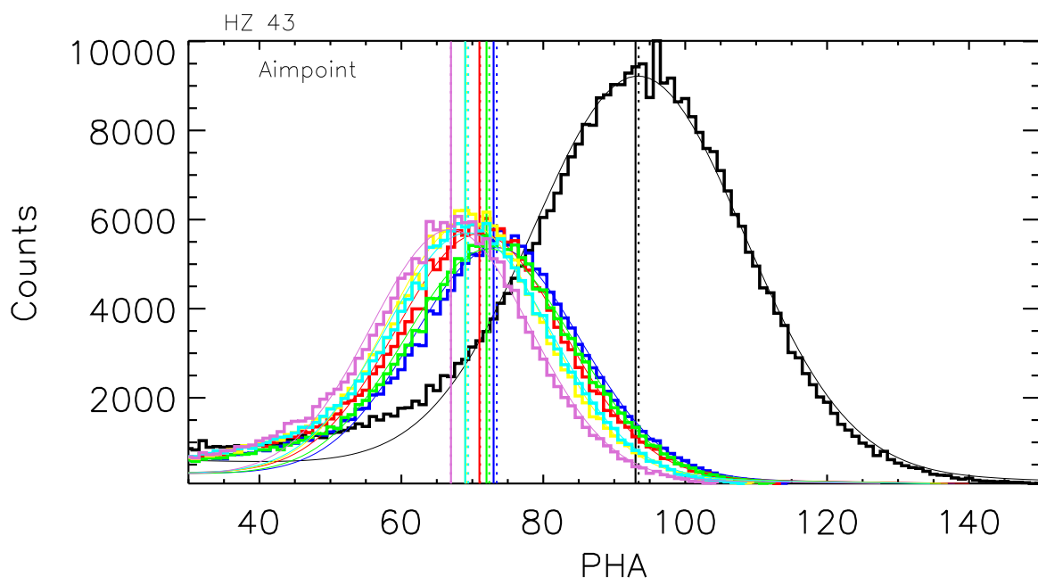
Figure 4. HZ 43 aimpoint PHA distribution. Solid vertical lines mark the median PHA. Gaussian fits over-plotted. Note: total counts vary in accordance with differing exposure times per observation.
