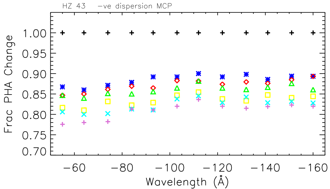
Figure 6. HZ 43 median PHA evolution (data as in Figure 5), normalized to ObsID 59. Top plot: positive dispersion MCP. Bottom plot: negative dispersion MCP.
