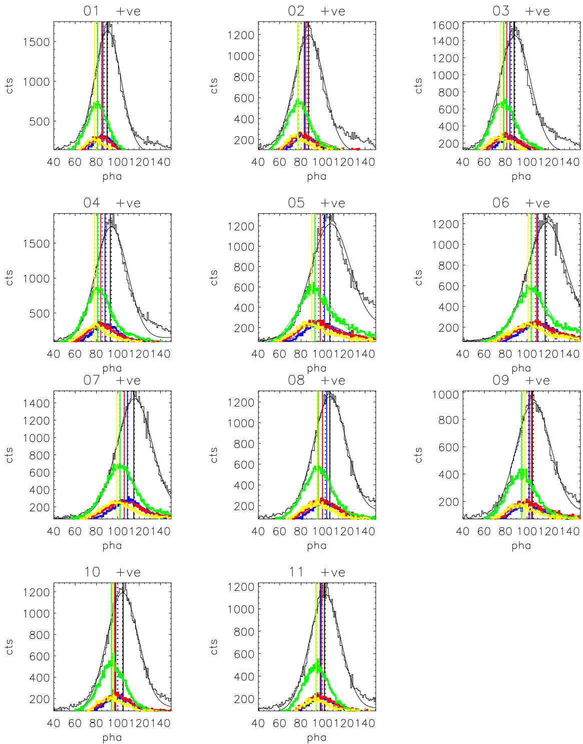
Figure 12. PKS 2155-304 central MCP PHA distributions. Solid vertical lines mark the median PHA. Gaussian fits overplotted. Bin numbers increase across central MCP from negative to positive, skipping over aimpoint.
