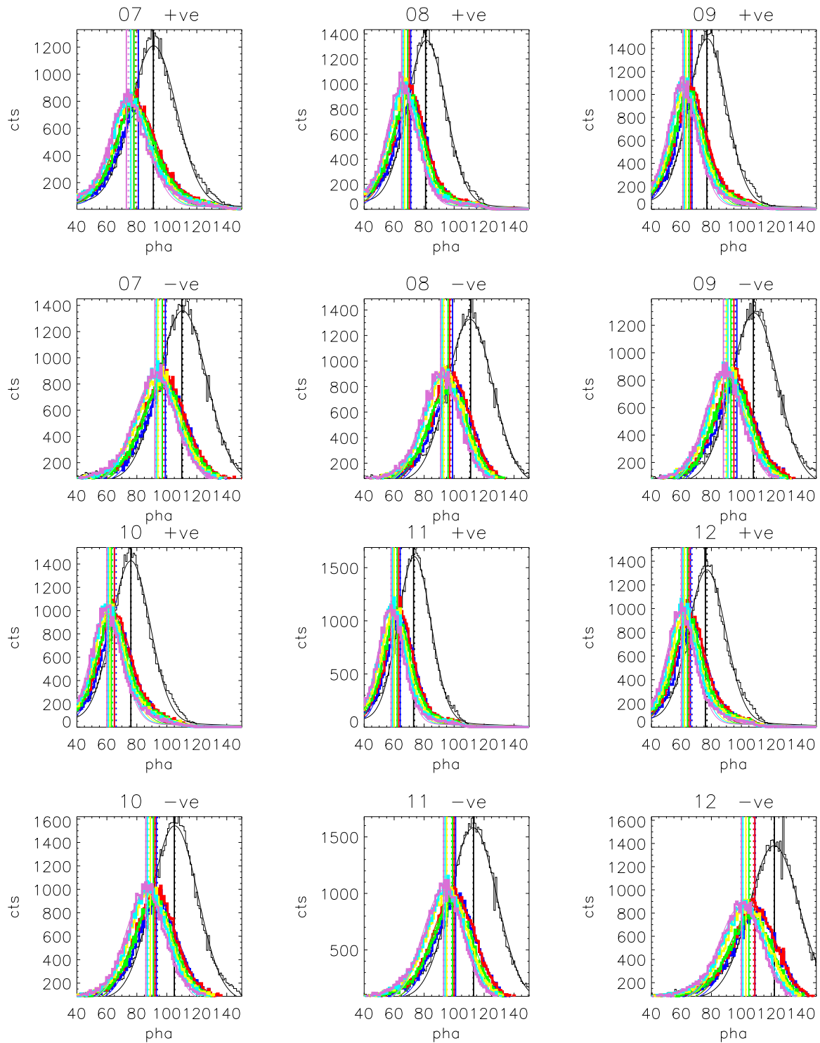
Figure 8. As in Figure 7. Bins 07–12.
