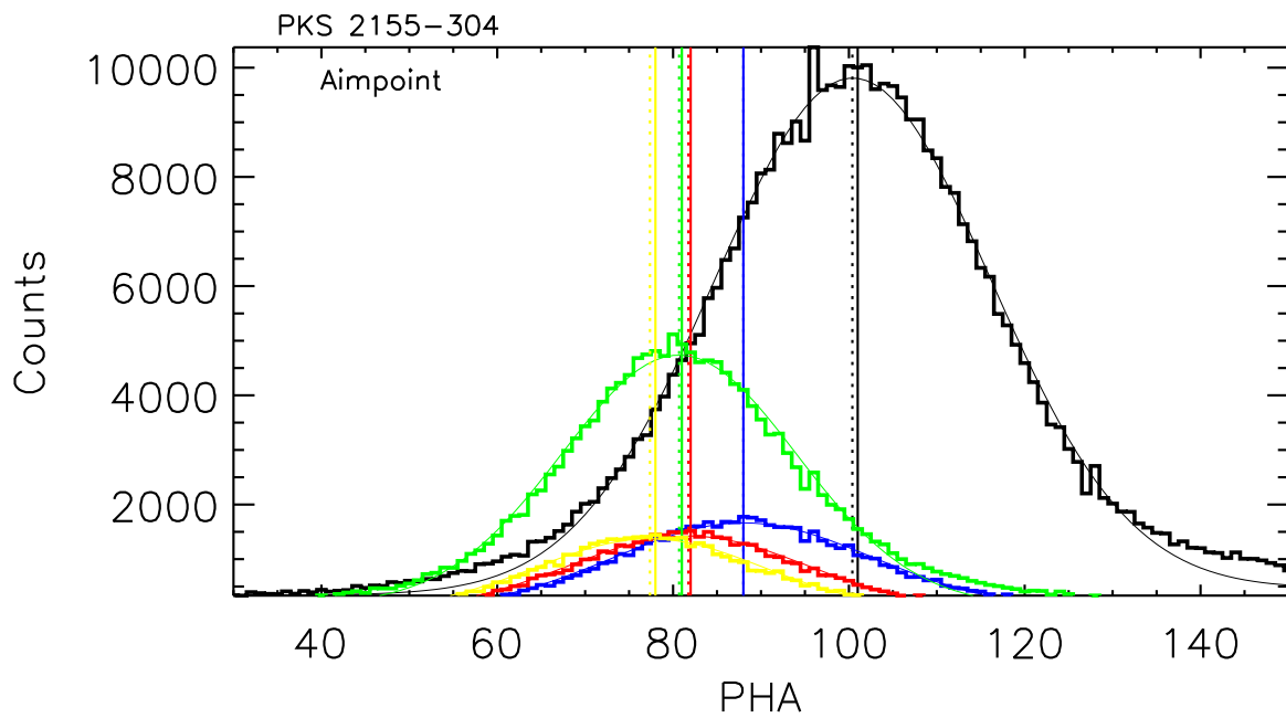
Figure 10. PKS 2155-304 aimpoint PHA distribution. Solid vertical lines mark the median PHA. Gaussian fits overplotted. Note: total counts vary in accordance with intrinsic source variability and differing exposure times per observation.
