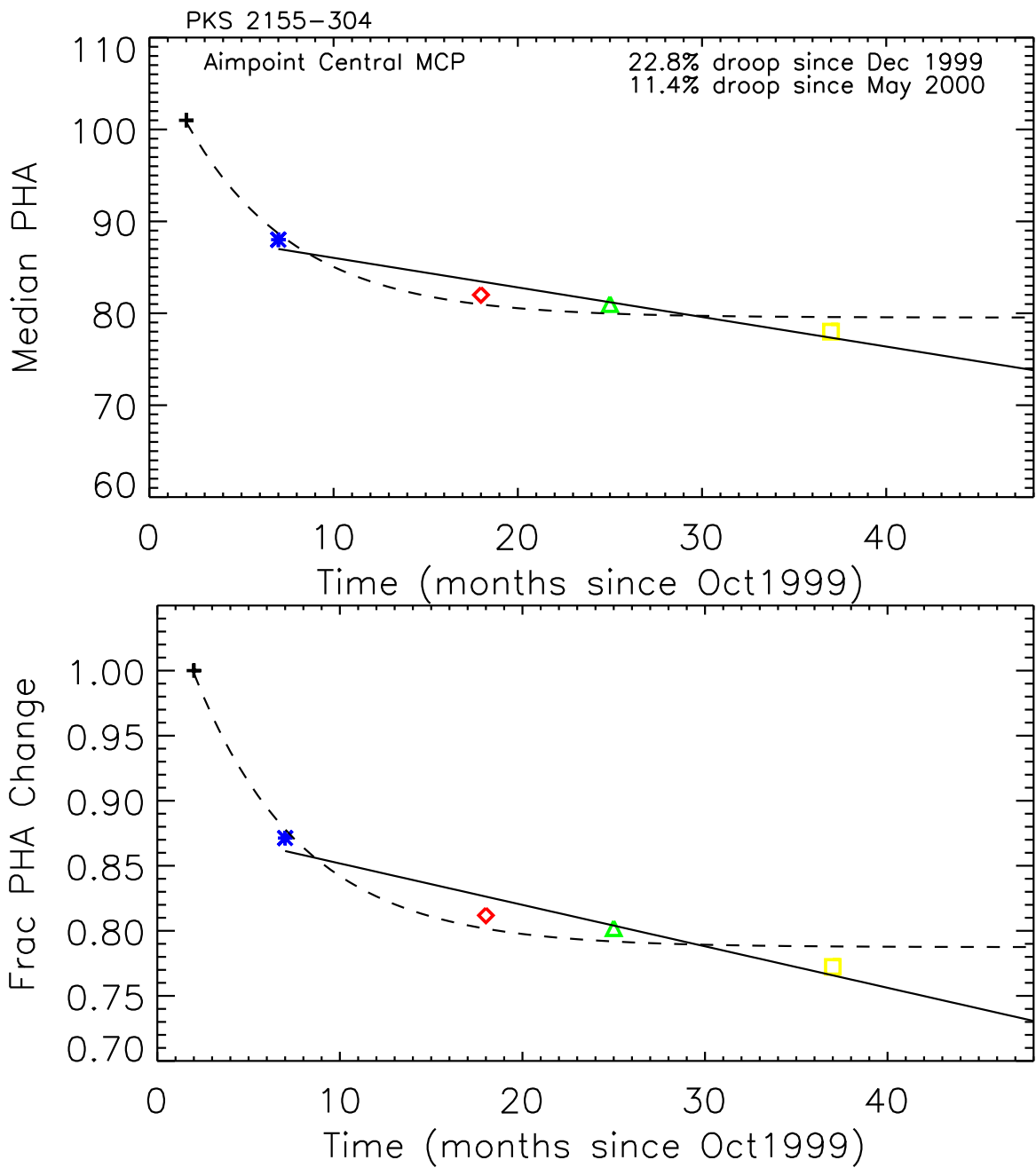
Figure 9. PKS 2155-304 aimpoint median PHA evolution, with exponential (dashed curve) and linear (solid line) fits (see text). Bottom plot normalized to first observation, ObsID 331.
