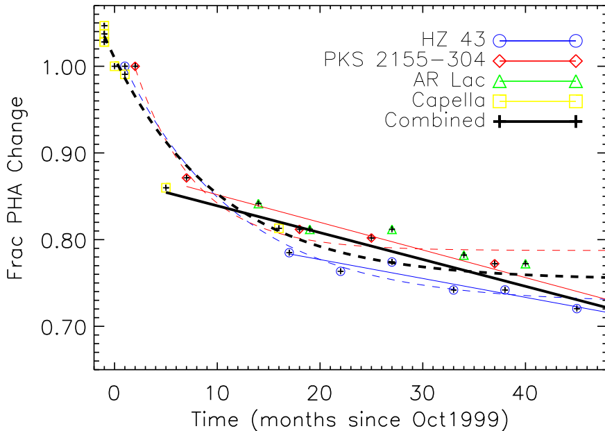
Figure 13. Aimpoint data for HZ 43 (blue), PKS 2155-304 (red), and Combined (HZ 43, PKS 2155-304, AR Lac and Capella – black), with exponential (dashed curve) and linear (solid line) fits to model PHA evolution. All observations are normalized to November/December 1999.
