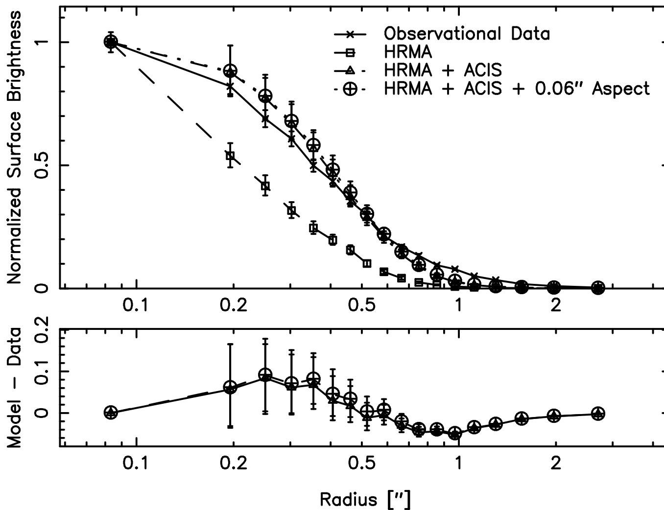
Merged off-axis ACIS Data: 35", 12° 2.0 keV < E < 3.0 keV
