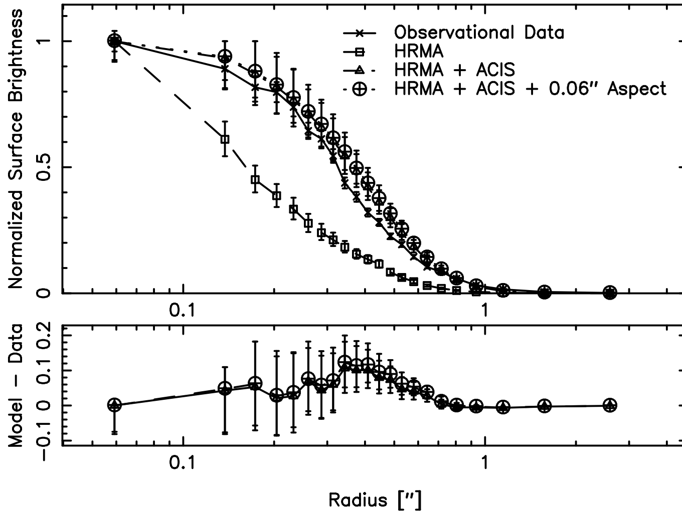
Merged off-axis ACIS Data: 35", 12° 0.0 keV < E < 1.0 keV
