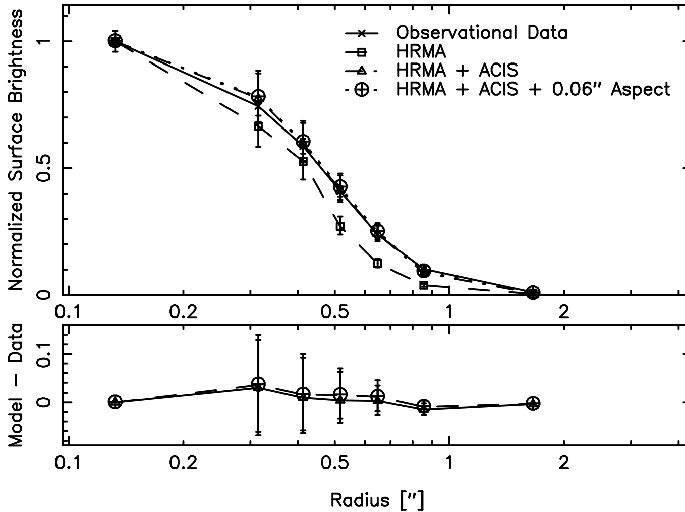
Merged off-axis ACIS Data: 7.7", 132° 6.0 keV < E < 9.0 keV
