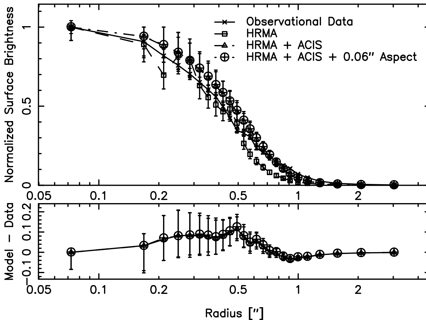
Merged off-axis ACIS Data: 35", 12° 6.0 keV < E < 9.0 keV
