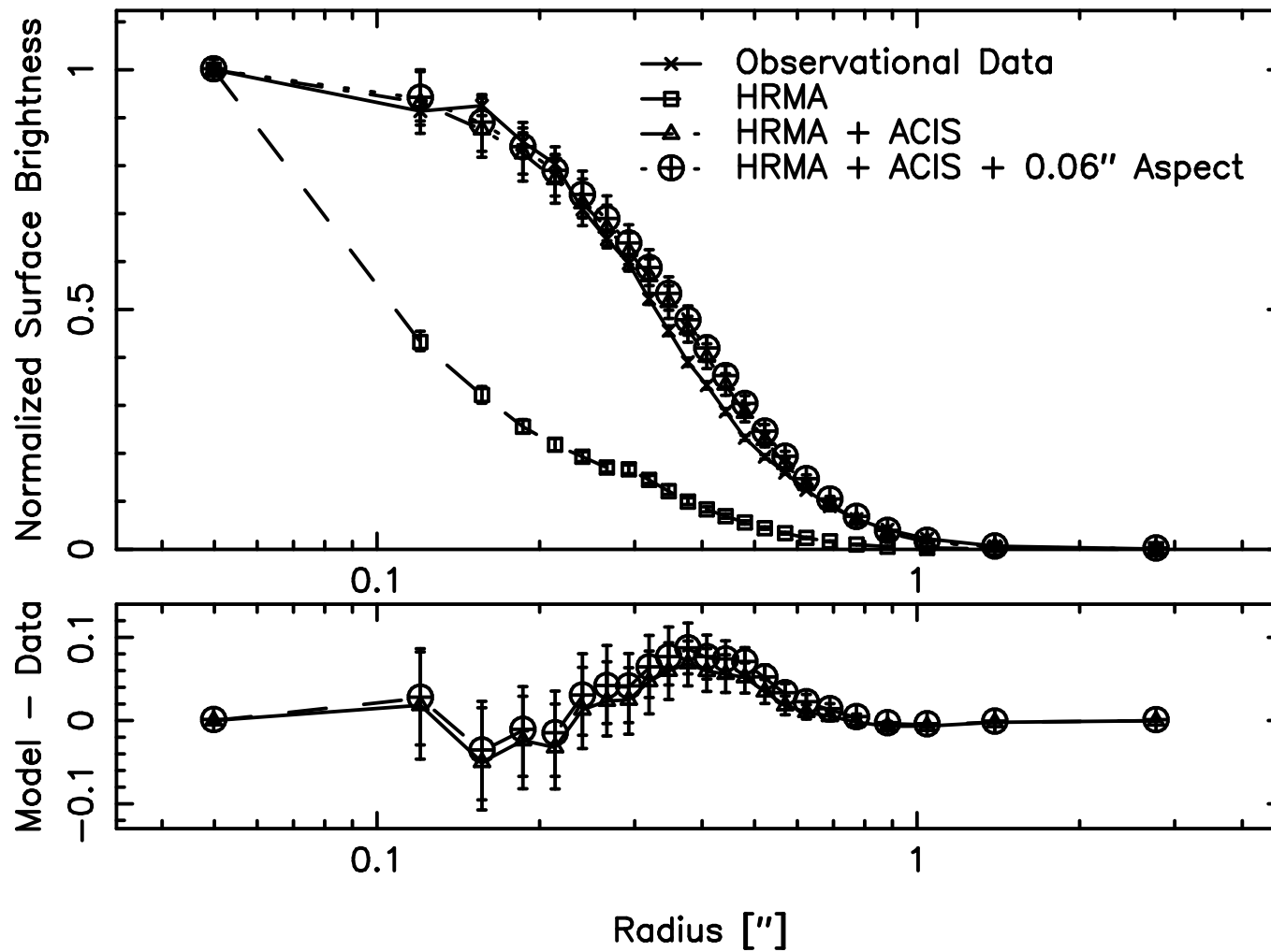
Merged off-axis ACIS Data: 7.7", 132°
