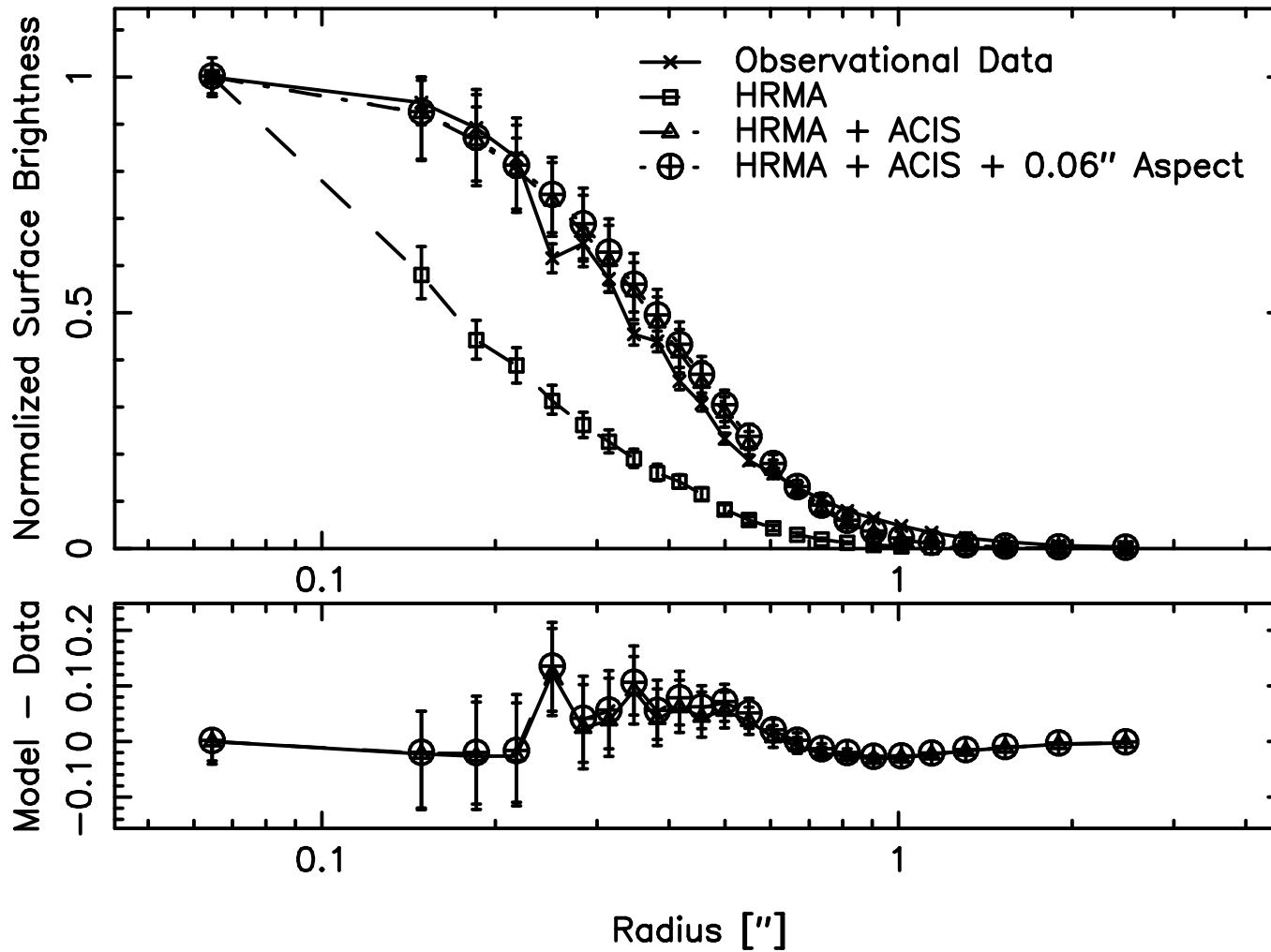
Merged off-axis ACIS Data: 35", 12° 1.0 keV < E < 2.0 keV
