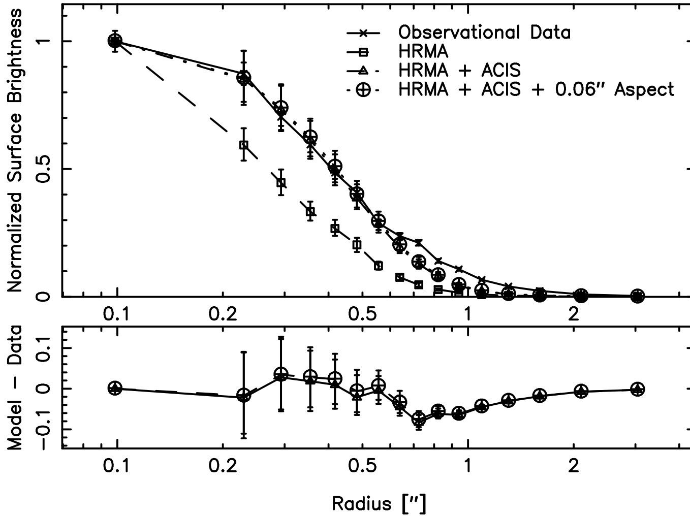
Merged off-axis ACIS Data: 35", 12° 5.0 keV < E < 6.0 keV
