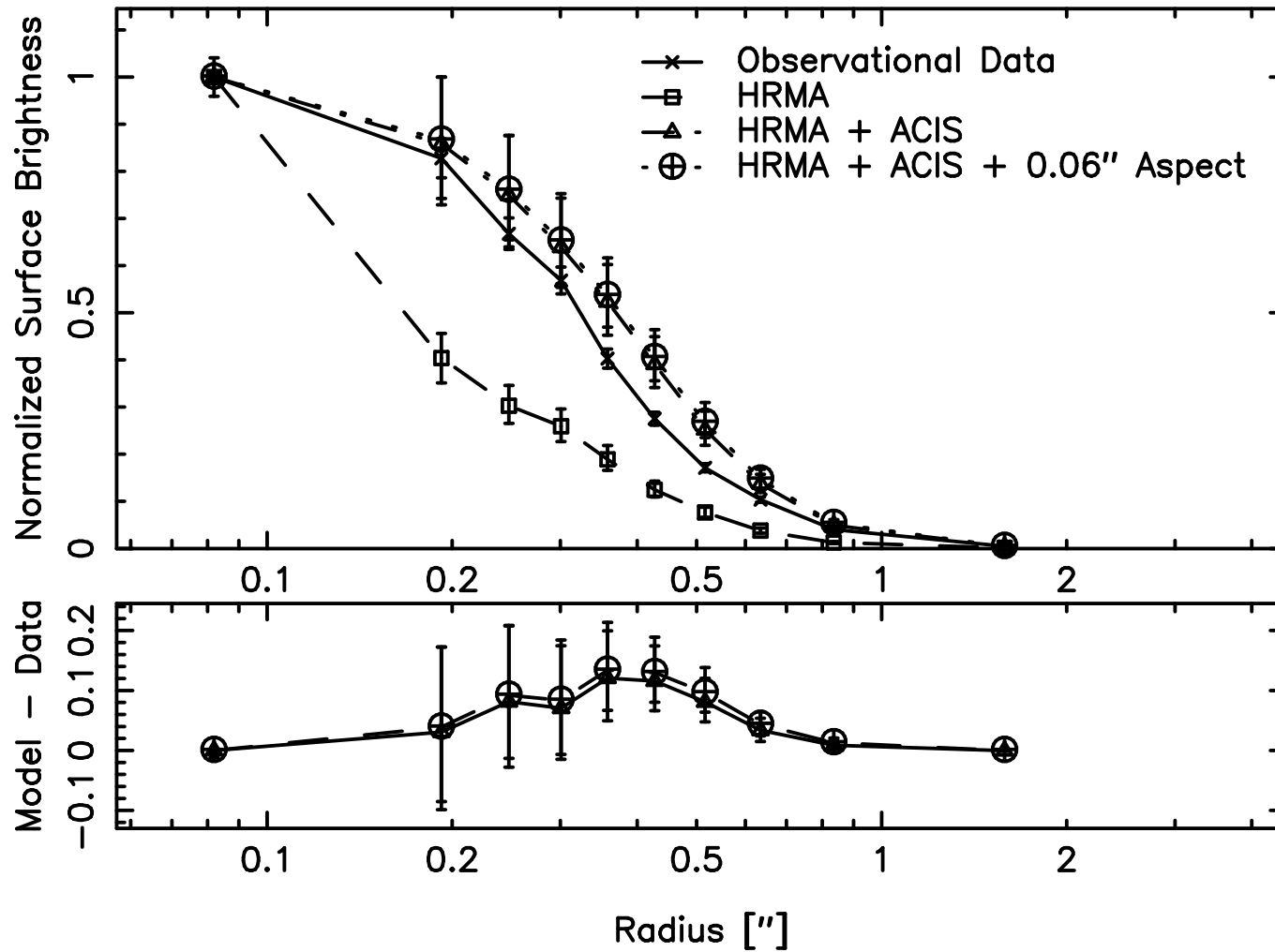
Merged off-axis ACIS Data: 7.7", 132° 2.0 keV < E < 3.0 keV
