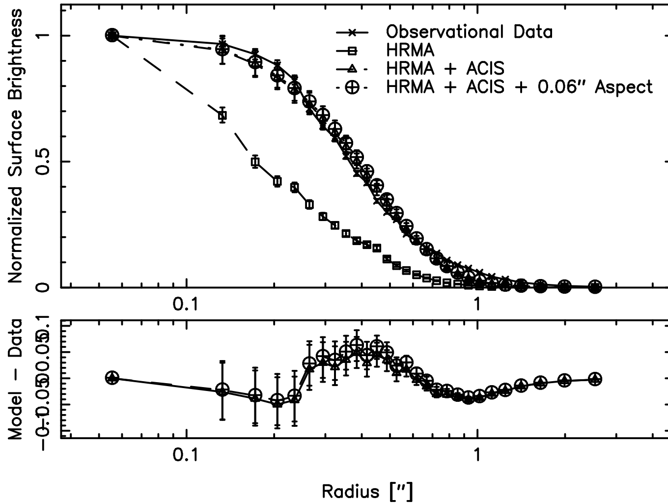
Merged off-axis ACIS Data: 35", 12°
