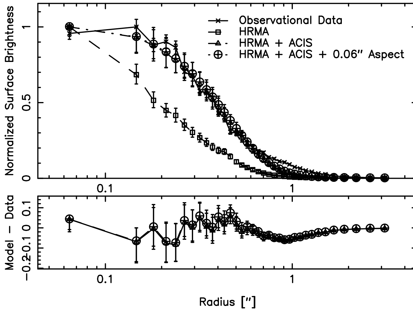
Merged off-axis ACIS Data: 35", 12° 3.0 keV < E < 5.0 keV
