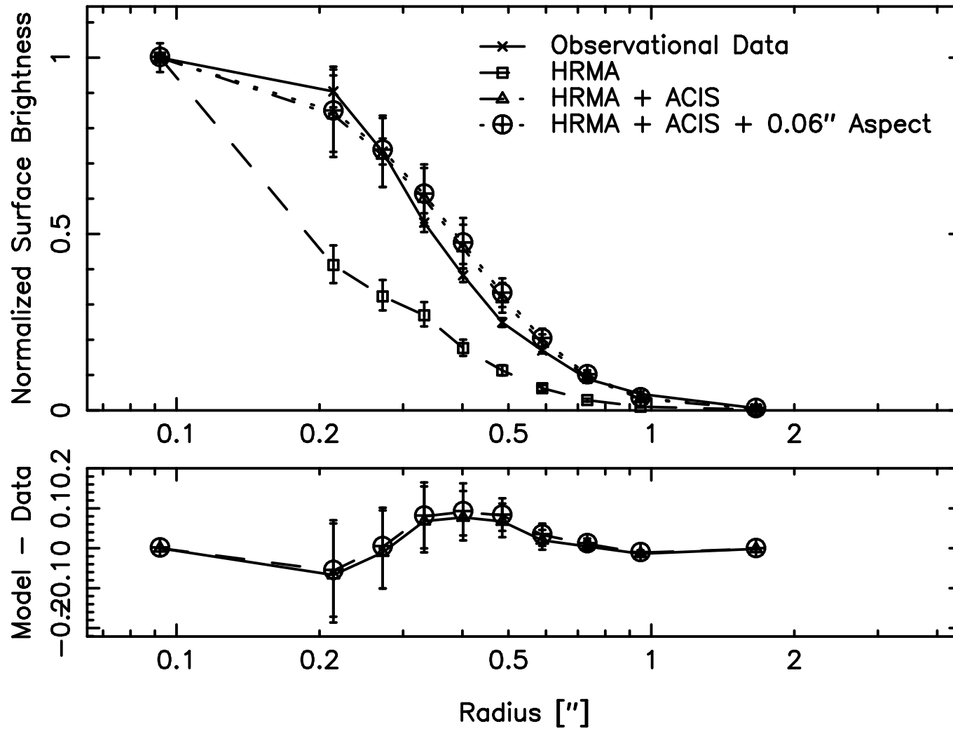
Merged off-axis ACIS Data: 7.7", 132° 3.0 keV < E < 5.0 keV
