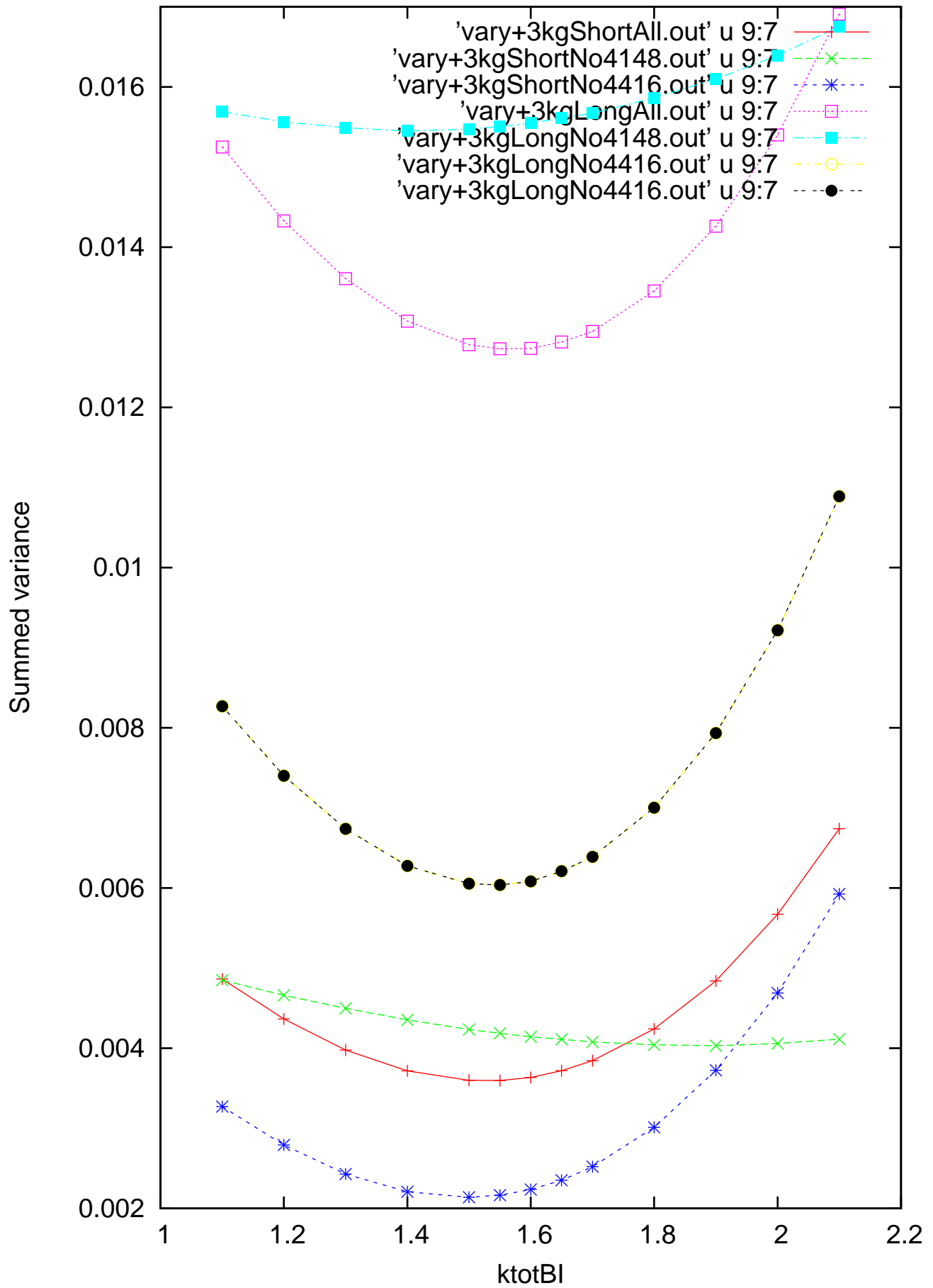
Varying ktotBI for m=+3 with kpBI(ED)=0.41; 5.6-6.4/6.6-8.45 Ang
