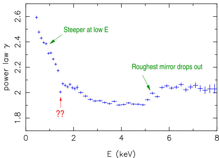
Figure F.1: Powerlaw index for fits to the narrow band obsid 3662 data.
