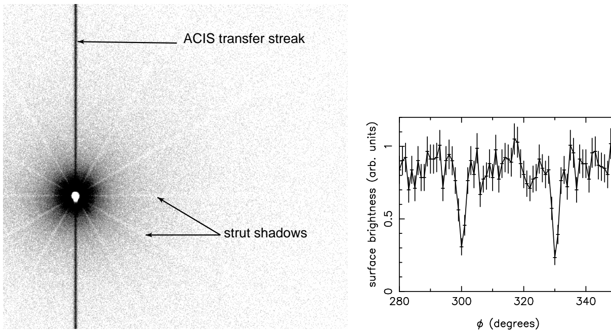
Figure 3: Left: Closeup of the deep Her X-1 wings observation. The ACIS transfer streak results from photons hitting the detector during the frame transfer to the frame store. The observation is notable for showing the shadows produced by the mirror support struts. Right: azimuthal variation of the 0.5–2.0 keV diffuse emission 1–2' from the source; 1° bins in \phi .
