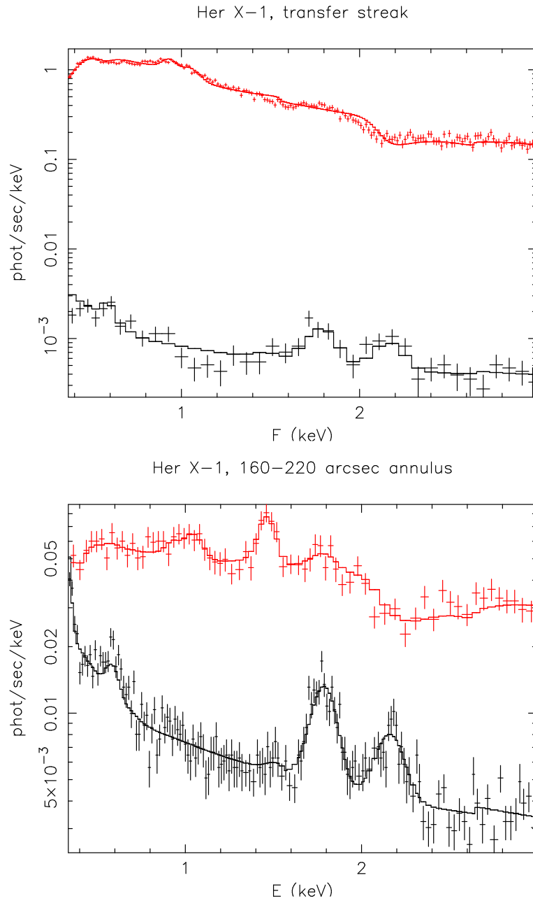
Figure F.2: Top: Spectrum for the transfer streak of Her X-1 (obsid 3662). Frame transfer is effectively a different ACIS mode, and it has not been calibrated. There is a shift in the slope of the gain of at least a few percent; this can be seen clearly at the Ir M edge just above 2 keV. (The rate has not been corrected for the effective transfer streak duty cycle.) Bottom: Spectrum for Her X-1 (obsid 3662) for an annular region 160–220'' from the source. In both panels, the upper curve is the Her X-1 obsid 3662 data. The lower curve shows the spectra for the corresponding blank sky data.
