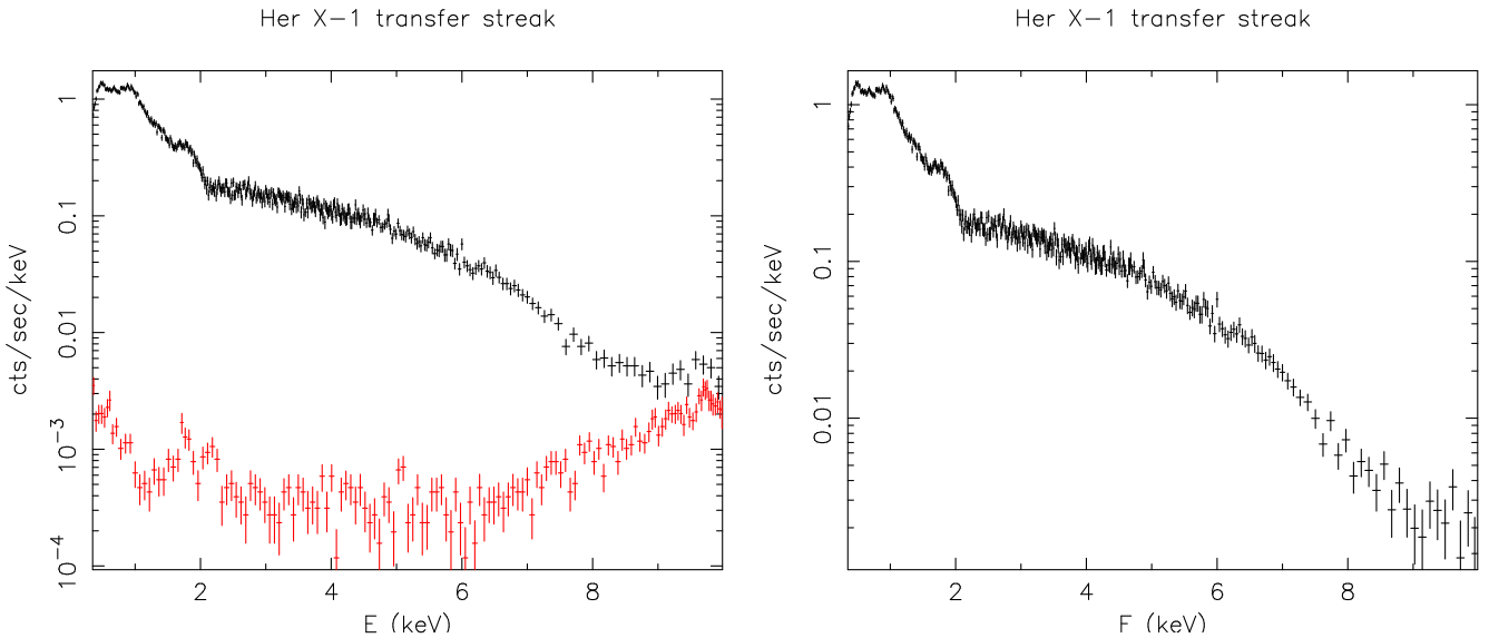
Figure E.1: Spectrum for the bright core of the Her X-1 transfer streak. Left: top curve: streak spectrum; bottom curve: spectrum extracted from the corresponding region of the blank sky data. Right: background-subtracted transfer streak spectrum. .
