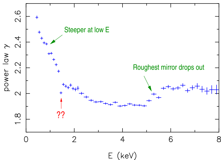
Figure 4: Powerlaw index for fits to the narrow band ObsID 3662 data. See text and Appendix F for further discussion of the “glitch” near 1.5 keV.
