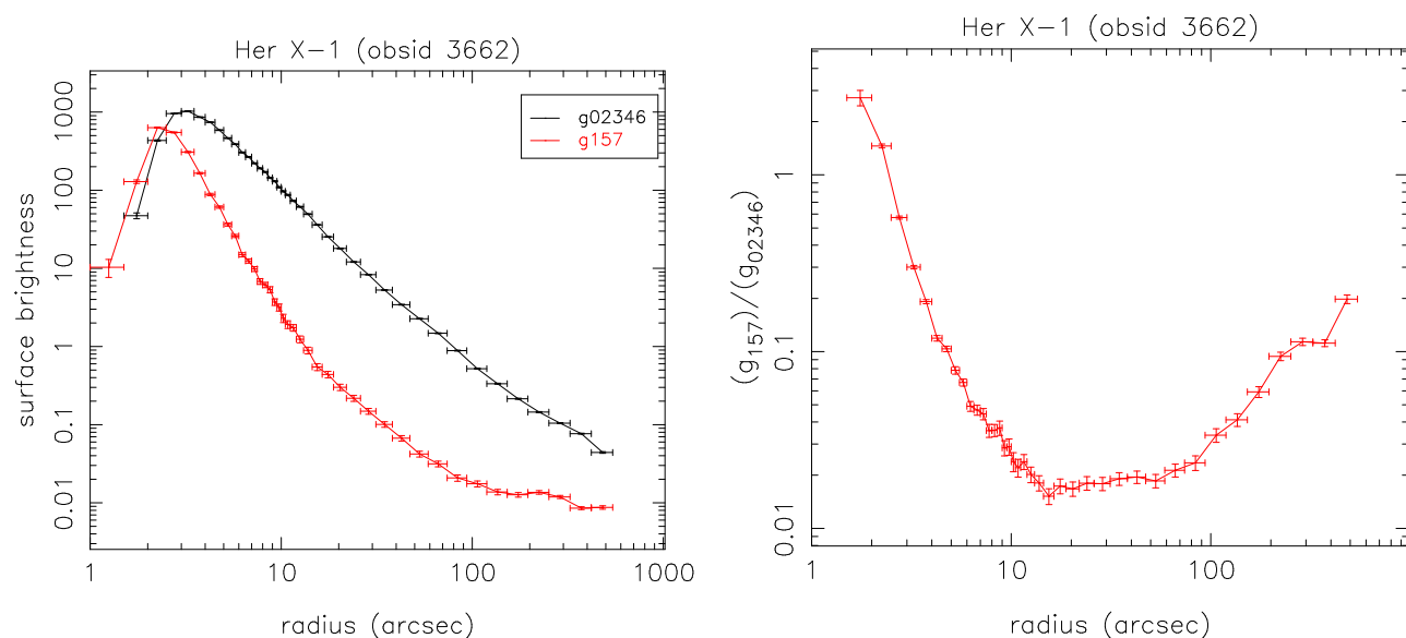
Figure A.2: Left: Her X-1 data. Surface brightness profiles for ASCA good grades and ASCA bad grades. Status filtered and energy filtered 0.5 - 2.0 keV. No exposure correction applied. Right: Her X-1 data: as in bottom left figure, but showing the ratio of ASCA bad grades to ASCA good grades.
