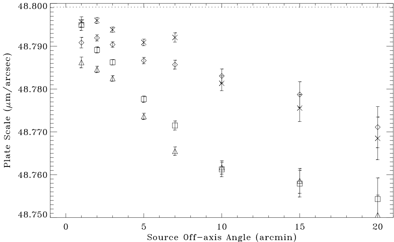
HRMA Plate Scale E = 8.638 keV
