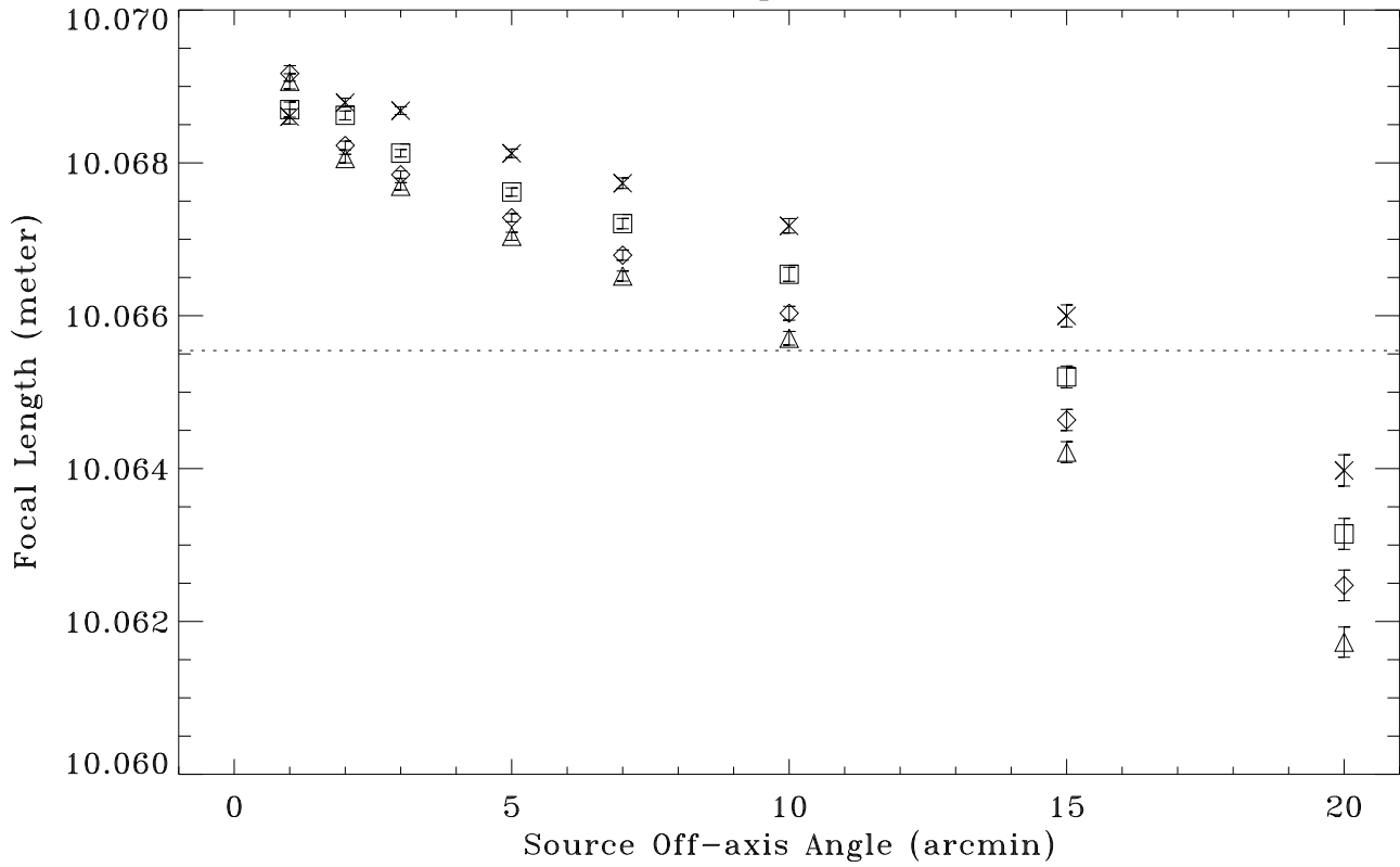
HRMA Plate Scale E = 4.510 keV
