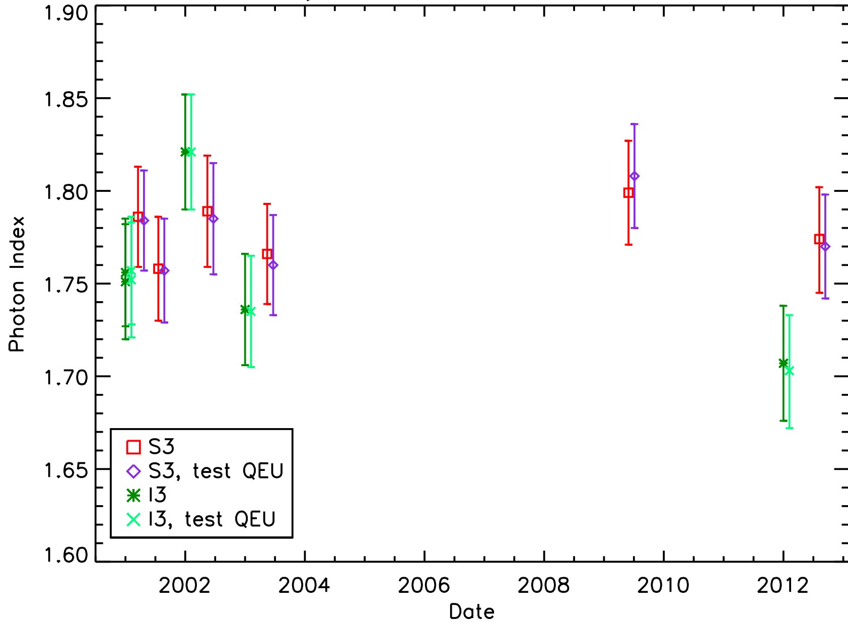
ACIS subarray G21.5-0.9 fit results: Photon Index
