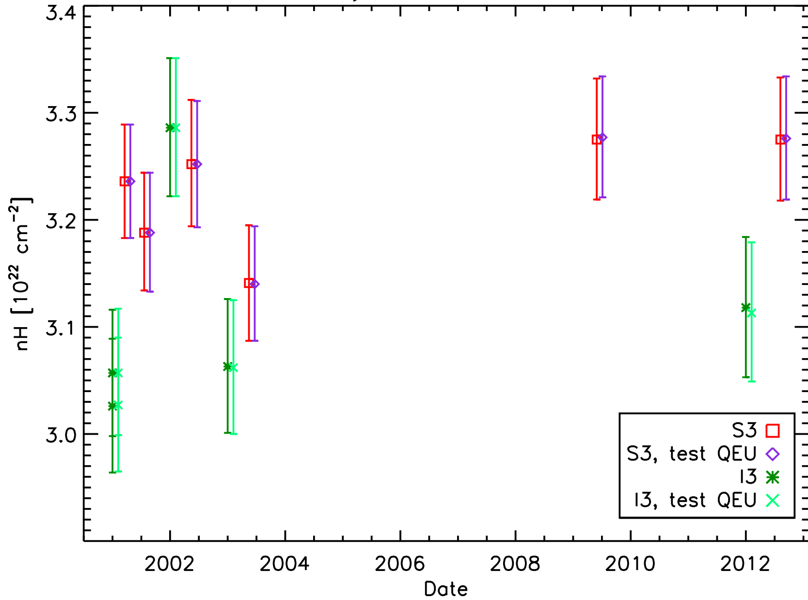
ACIS subarray G21.5-0.9 fit results: nH
