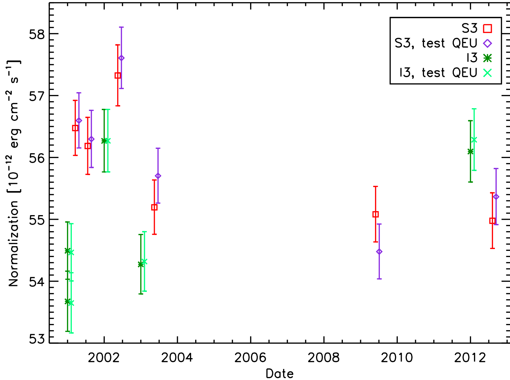
ACIS subarray G21.5–0.9 fit results: Flux in 2–8 keV
