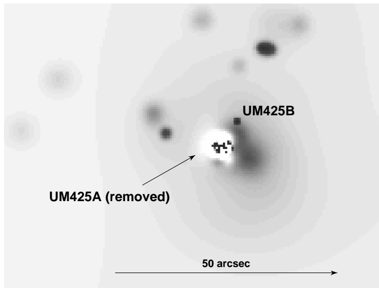
FIG. 5.— Adaptively smoothed soft-band (0.3-3 keV) image of the UM 425 field with the central UM 425A point source subtracted. North is up, East to the left. An elliptical component of diffuse emission centered about 5'' west of UM 425A is seen. The central 15'' core of the emission contains \sim 50 photons, giving an integrated count rate of 4.6 \times 10^{-4} cts s^{-1} . The bright source \sim 25'' N-NW of UM 425A corresponds to a bright foreground galaxy.
