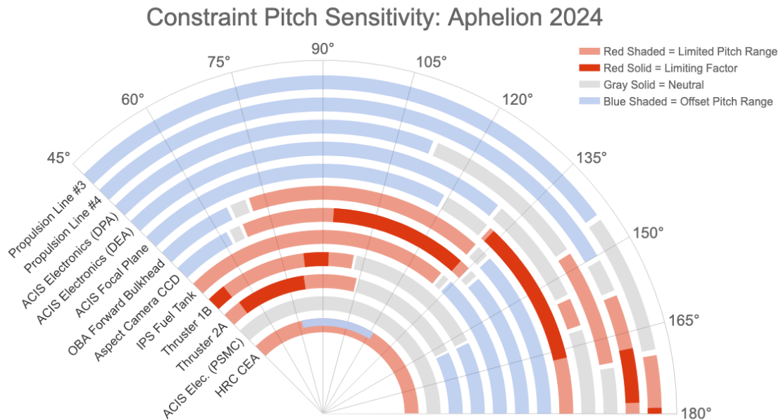
Figure 3.5: Illustration of the thermal impact of solar pitch angle on various spacecraft components with ACIS at the focus. Pale red arcs indicate pitch ranges in which it is more difficult to maintain the component within its thermal restrictions, gray arcs show where components are thermally neutral, and pale blue arcs indicate pitch ranges in which components can recover from time spent in thermally limited pitch regions. Dark red arcs indicate where a component represents the most limiting dwell time restriction at a given pitch angle; the MUPS at low pitch angles, ACA at mid-pitch, ACIS at high pitch, and the propulsion lines at the highest pitch angles. The HRC heats at all pitches while switched on, and only cools efficiently in a limited range of pitches while switched off. Note that the diagram represents the predicted status during 2024 with ACIS at the focus; thermal constraints will change over time so it should not be used as a guide for planning specific observations. For detailed inquiries regarding pitch sensitivity, please contact the CXC HelpDesk ( https://cxc.harvard.edu/helpdesk/ ).
