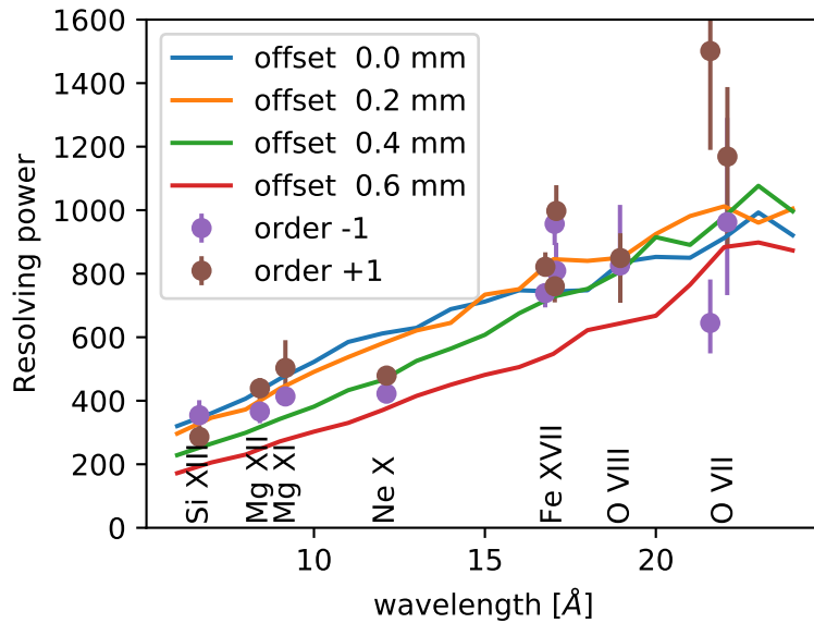
Figure 8.26: Expected spectral resolving power for HETG with the HRC-I detector for different focus offsets, based on ray-trace simulations using MARX (see § 8.6). Offsets between 0.0 and 0.4 mm provide the best spectral resolution for this configuration, and depend on the wavelength of interest. This figure is from Günther (2018).
