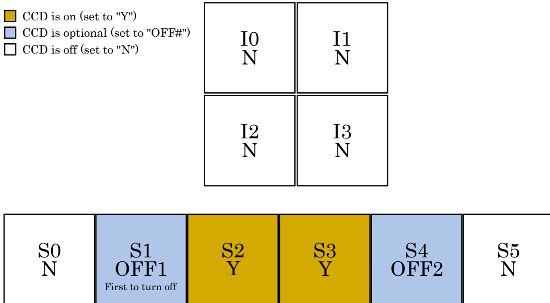
Figure 6.42: ACIS-S imaging, nominal S3 aimpoint (2 Required CCDs, 2 optional CCDs)
