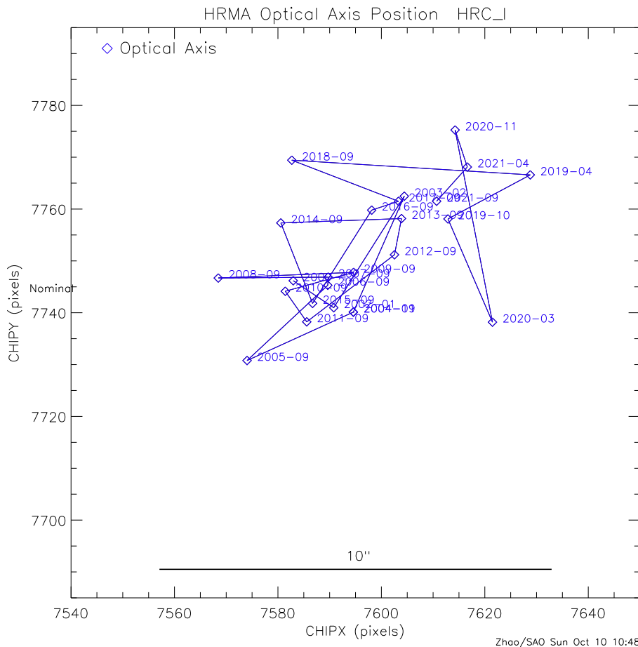
Figure 4.26: Chandra optical axis positions on HRC-I since launch. Each position is labeled by the year-month. The optical axis position is very stable and well within a 10 arcsec region.
