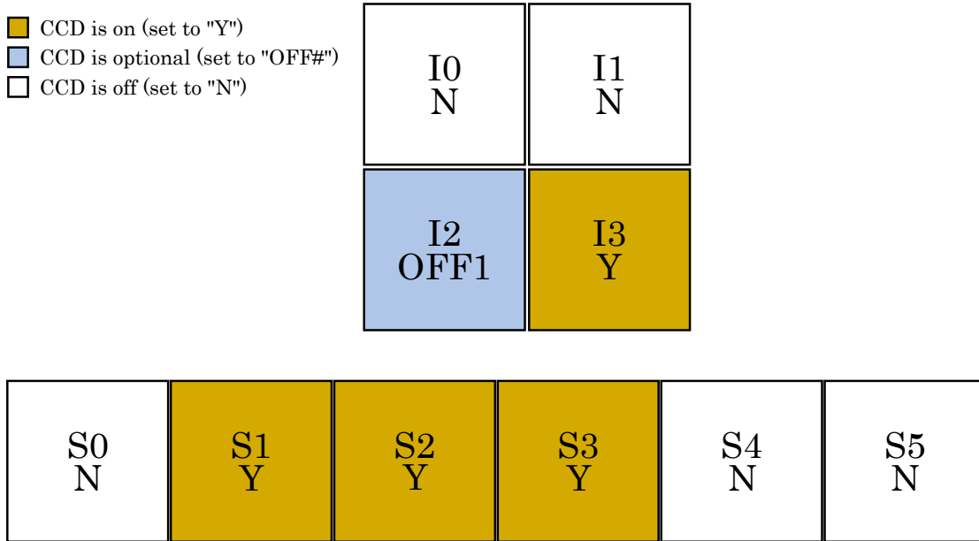
Figure 6.45: ACIS-S imaging, nominal aimpoint (4 Required CCDs, 1 Optional CCD)
