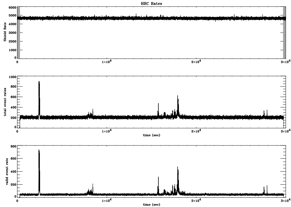
Figure 7.12: An example of the background variability during a \sim 30 ks HRC-I observation of the supernova remnant (SNR) SNR G21.5-09 taken on 1999-Oct-25. The total event rate (middle) and valid event rate (bottom) show correlated bursts up to \sim 800 \text{cts s}^{-1} . The bursts are uniformly distributed over the detector. The anti-coincidence shield (top) exhibits no correlated enhancements. The total and valid rates differ by \sim 200 \text{cts s}^{-1} due primarily to cosmic ray events that are vetoed and don't appear as valid events in the telemetry.
