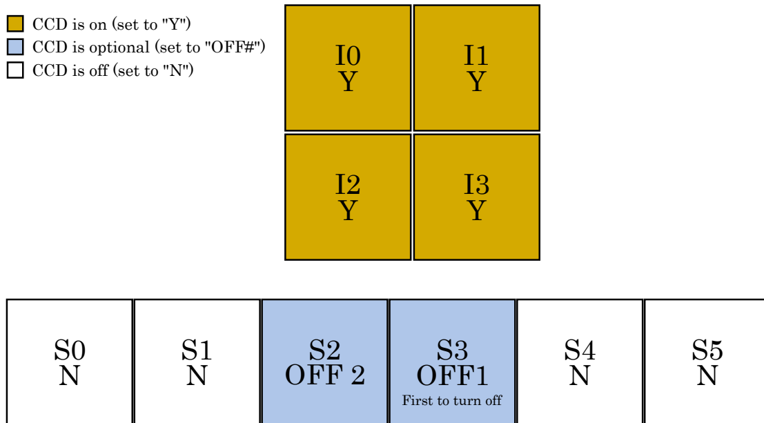
Figure 6.40: ACIS-I imaging, nominal I3 aimpoint (4 Required CCDs, 2 Optional CCDs)
