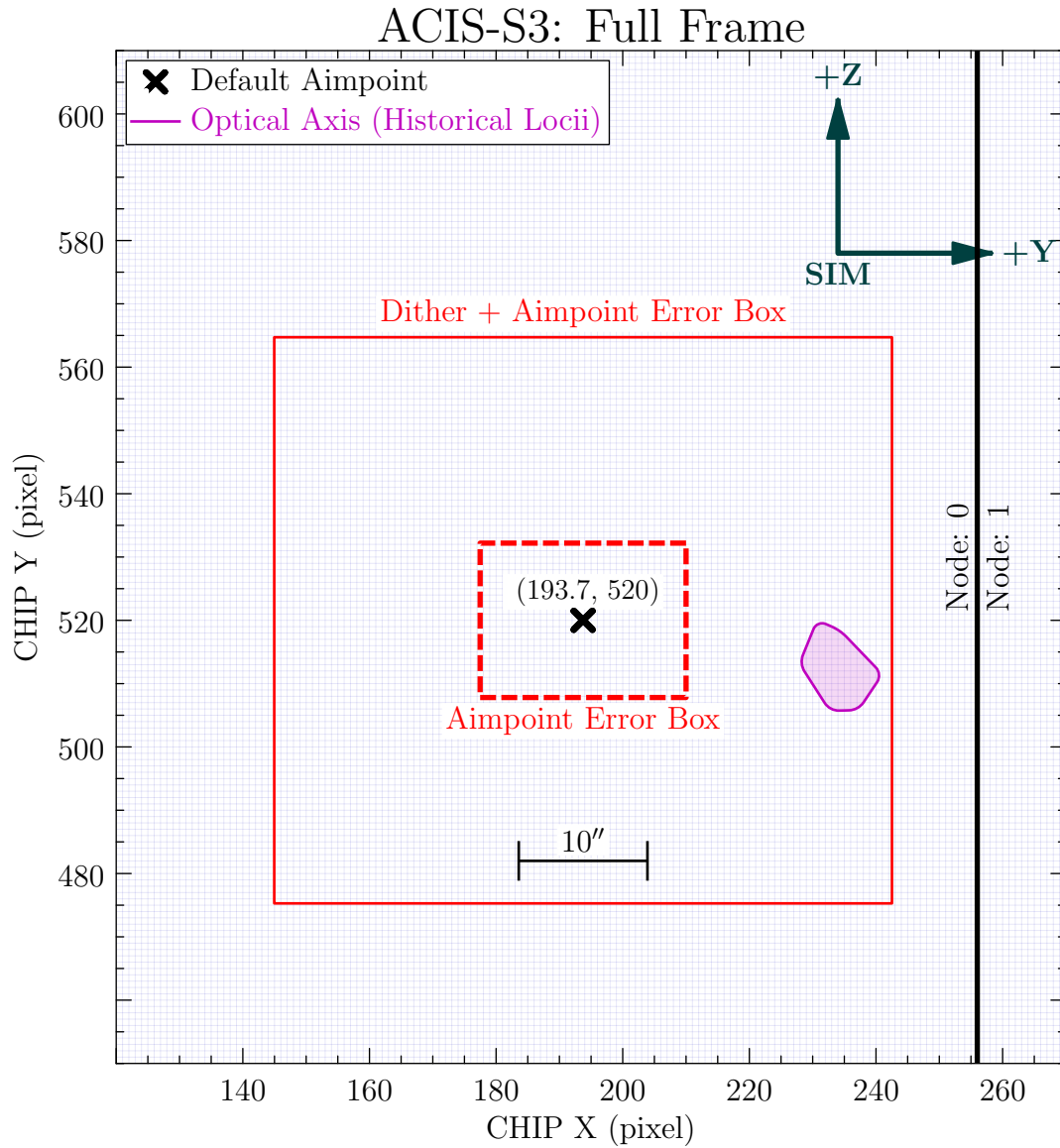
Figure 4.29: ACIS-S3 Full-Frame PDA & Dither Box. The Chandra historical optical axis locii are represented by the purple blob; the Permanent Default Aimpoint (PDA) by the black cross. The smaller red dashed-line box centered at the PDA is the error box of the effective aimpoint center—an on-axis target can be anywhere inside this box. The larger red solid-line box contains the dither pattern convolved with the error box. The PDA is shifted \sim 12 arcsec from the optical axis to avoid the node boundary 0|1.
