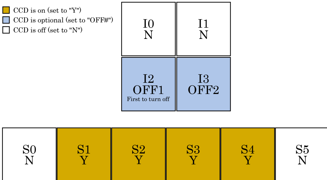
Figure 6.46: ACIS-S imaging, nominal aimpoint (4 Required CCDs, 2 Optional CCDs)
