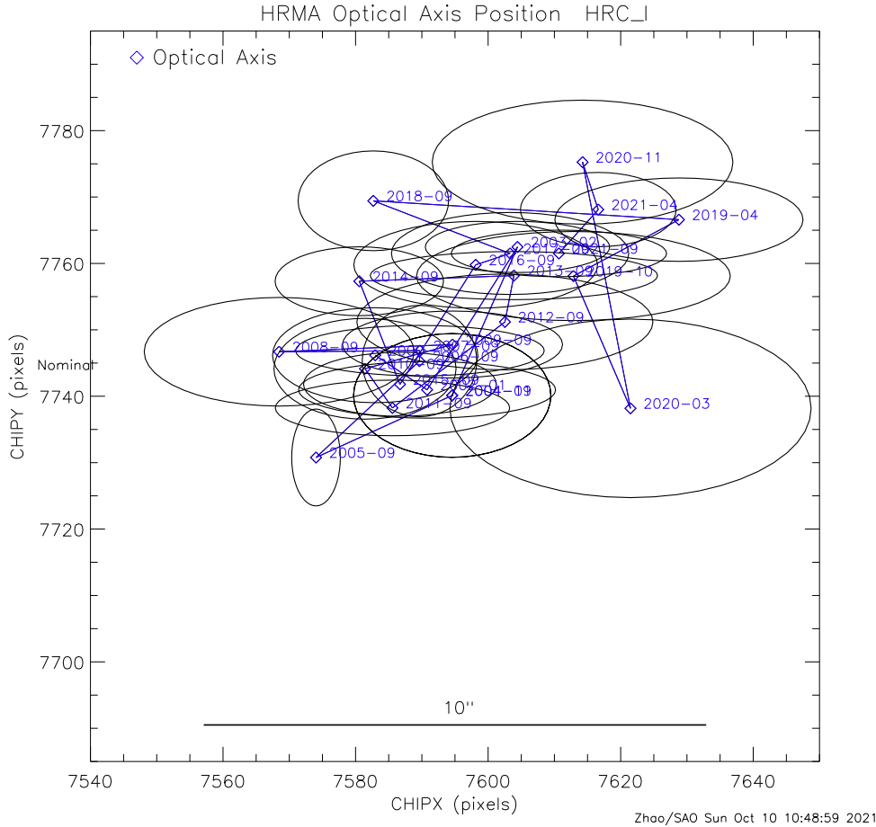
Figure 4.27: The same as Figure 4.26, with the 1\text{-}\sigma measurement error ellipse around each position for that given year. The drift of optical axis position is consistent with the measurement errors.
