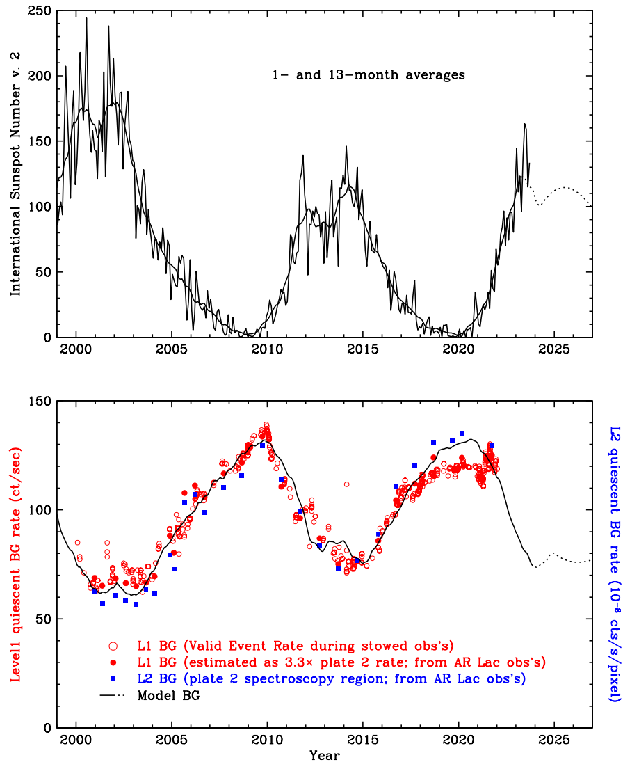
Figure 9.21: Solar cycle and HRC-S background. Top: Monthly sunspot numbers and with 13-month smoothing; dotted curve is predicted. Bottom: Level 1 background rate is for the LETGS standard spectroscopy region, derived from AR Lac monitoring data (without a grating) and from NIL-mode observations when the HRC-S is in the stowed position. The “typical” Level 2 (L2) rate is 1.0 \times 10^{-6} cts s^{-1} pixel ^{-1} , but this varies with the solar cycle. L1 and L2 background rates are not exactly correlated because of changes in the effects of L1-to-L2 filtering over time, particularly during the period of increasingly low gain prior to the May 2021 high voltage increase. The continuous black curve represents a simple model of the HRC-S background rate based on sunspot number with a 1-year lag (or 0.7 years after the 2009 solar minimum) corresponding to the approximate time for the solar wind to reach the heliopause, where its magnetic field helps deflect cosmic rays from entering the solar system. Rates in Figure 9.22 correspond to a Level 2 rate of 1.1 \times 10^{-6} cts s^{-1} pixel ^{-1} .
