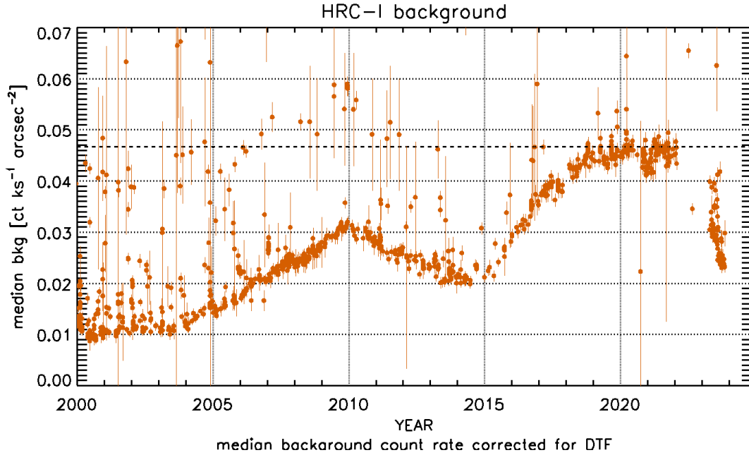
Figure 7.13: The change in HRC-I background rate with time. The deadtime corrected count rate per square arcsec is shown with error bars for each HRC-I observation. The lower envelope represents the quiescent rate, and the fluctuations are due to the occasional background flaring. The HRC-S data are similar.
