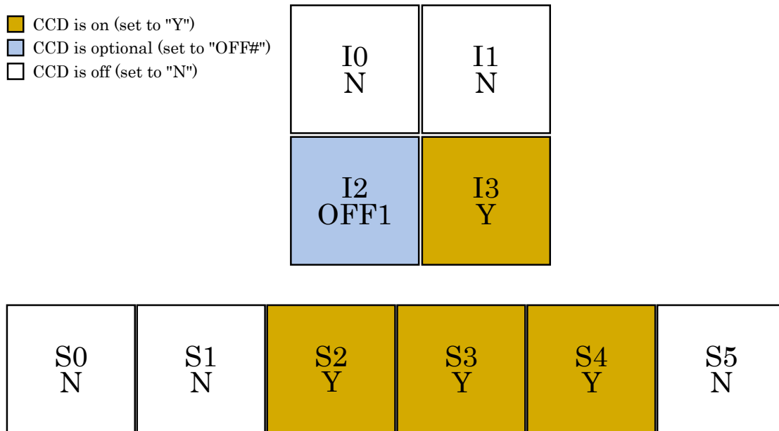
Figure 6.44: ACIS-S imaging, nominal S3 aimpoint (4 Required CCDs, 1 Optional CCD)
