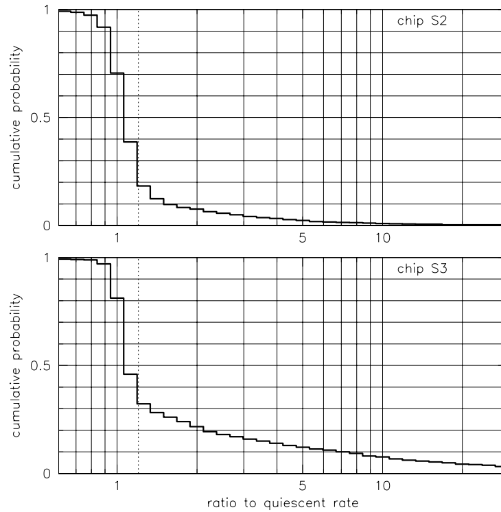
Figure 6.32: An estimate of the cumulative probability that the ratio of the background counting rate to the quiescent background counting rate is larger than a given value. The upper plot is for a representative FI chip (S2) and the lower plot is for a representative BI chip (S3). The vertical dotted line is a limiting factor 1.2 used in creating the background data sets. These probabilities are relevant for the archival data from the first 2–3 years of the mission. After declining with time to almost zero for a number of years, the amount of flaring has increased with solar maxima, but there has been less flaring than was seen in the first few years of the mission.
