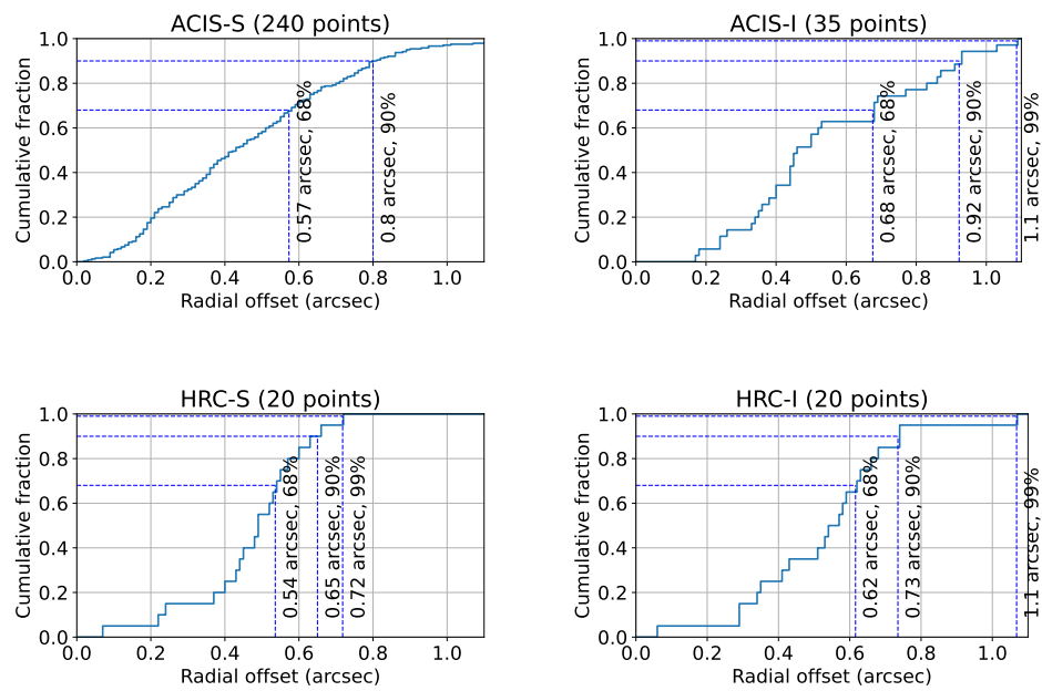
Figure 5.4: Cumulative histogram of celestial accuracy for Chandra X-ray source locations for each SI using observations since 2018-Oct. Radial offset is the distance in arcsec between the optical coordinate, typically from the Tycho-2 catalog, and the Chandra position.
