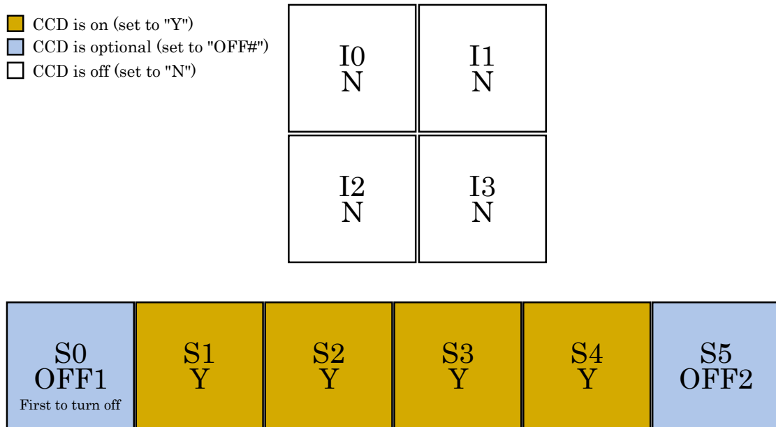
Figure 6.47: ACIS-S spectroscopy, nominal aimpoint (4 Required CCDs, 2 Optional CCDs)
