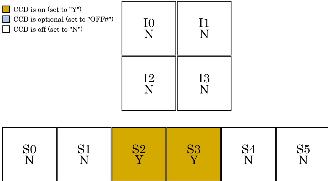
Figure 6.41: ACIS-S imaging, nominal S3 aimpoint (2 Required CCDs)
