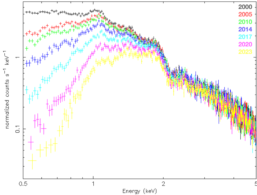
Figure 6.8: ACIS-S spectrum of the galaxy cluster Abell 1795 at seven different epochs ranging from 2000 to 2023. The decreasing count rates in the spectrum of a stable calibration source demonstrate the loss of effective area due to the build-up of the contaminant on the ACIS OBF.
