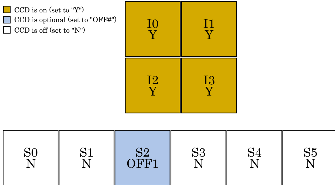
Figure 6.38: ACIS-I imaging, nominal I3 aimpoint (4 Required CCDs, 1 Optional CCD)
