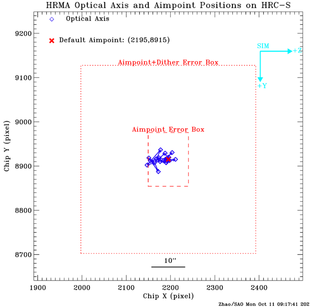
Figure 4.33: Chandra optical axis (blue diamonds) positions for each year and permanent default aimpoint (red cross) on HRC-S at [2195,8915]. The small box (red dashed line, 12 arcsec \times 16 arcsec, or 91.1 \times 121.4 pixels) centered at the permanent default aimpoint is the error box of the effective aimpoint center, i.e. an on-axis target can be anywhere inside this box. The large box (red dotted line, 52 arcsec \times 56 arcsec, or 394.7 \times 425.0 pixels) is the error box of effective aimpoint with dither.
