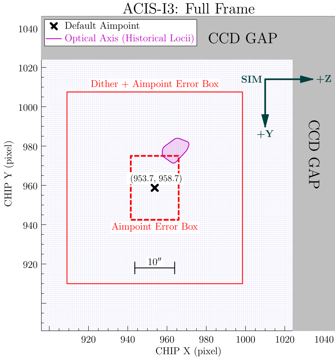
Figure 4.28: ACIS-I3 Full-Frame PDA & Dither Box. The Chandra historical optical axis locii are represented by the purple blob; the Permanent Default Aimpoint (PDA) by the black cross. The smaller red dashed-line box centered at the PDA is the error box of the effective aimpoint center—an on-axis target can be anywhere inside this box. The larger red solid-line box contains the dither pattern convolved with the error box.
