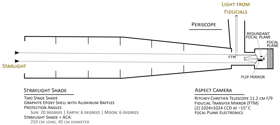
Figure 5.1: Aspect camera assembly
