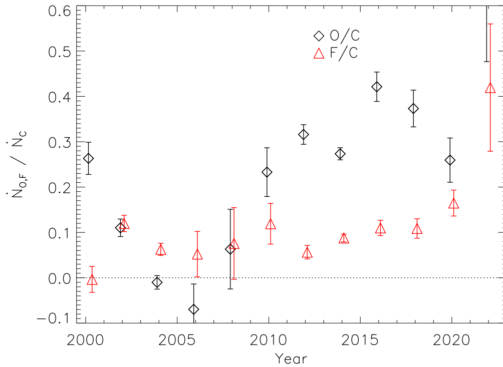
Figure 6.11: The ratio of the deposition rate in oxygen atoms and fluorine atoms per year to that for carbon over the Chandra mission as measured by LETG/ACIS-S observations of blazars.
