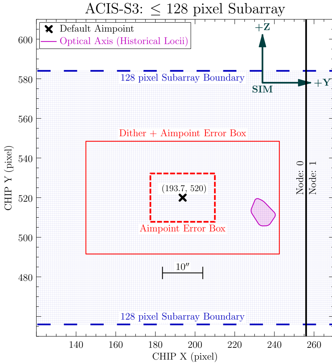
Figure 4.31: ACIS-S3 Dither Box on a subarray \leq 128 pixels. The Chandra historical optical axis locii are represented by the purple blob; the Permanent Default Aimpoint (PDA) by the black cross. The smaller red dashed-line box centered at the PDA is the error box of the effective aimpoint center—an on-axis target can be anywhere inside this box. The larger red solid-line box contains the dither pattern convolved with the error box.
