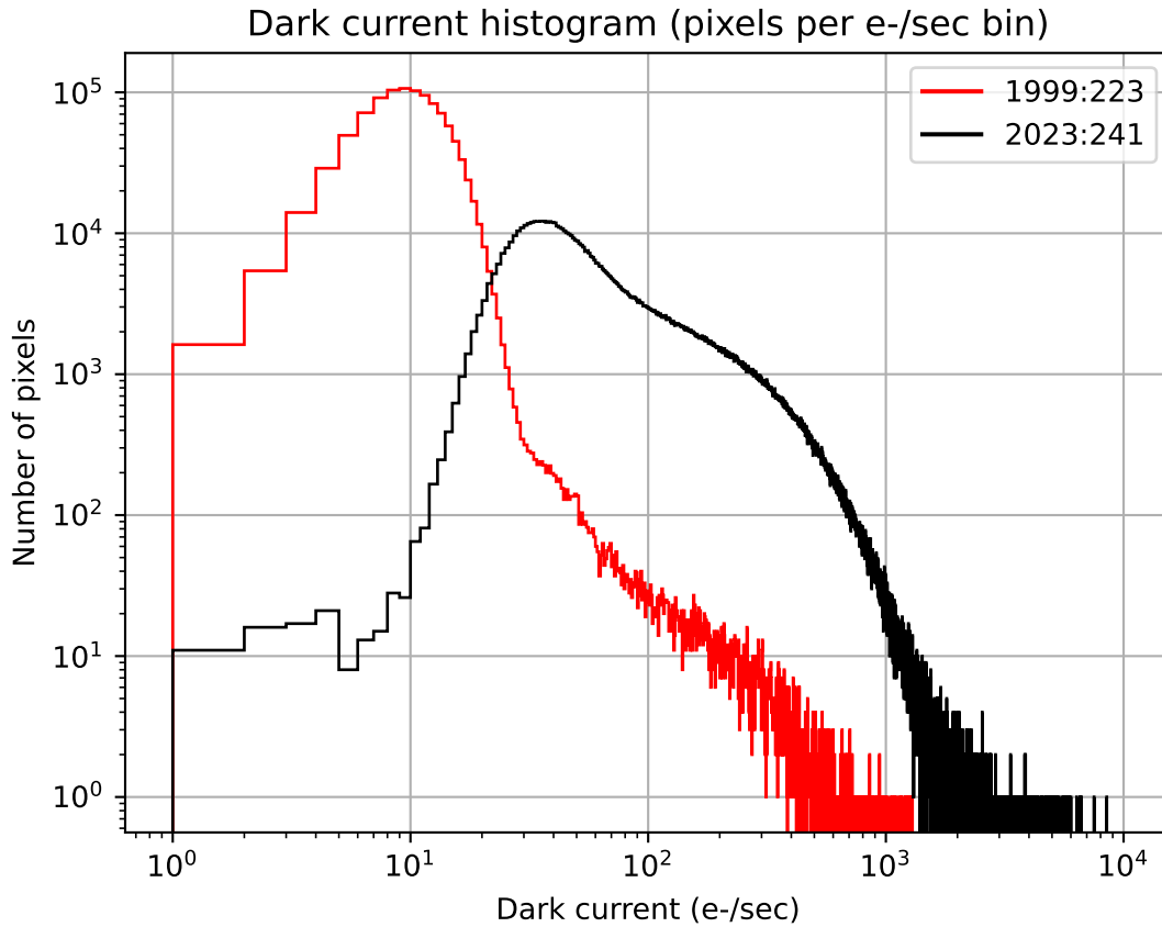
Figure 5.8: Differential histogram of dark current distribution for the ACA CCD on 1999-Aug-11 and 2023-Aug-29.
