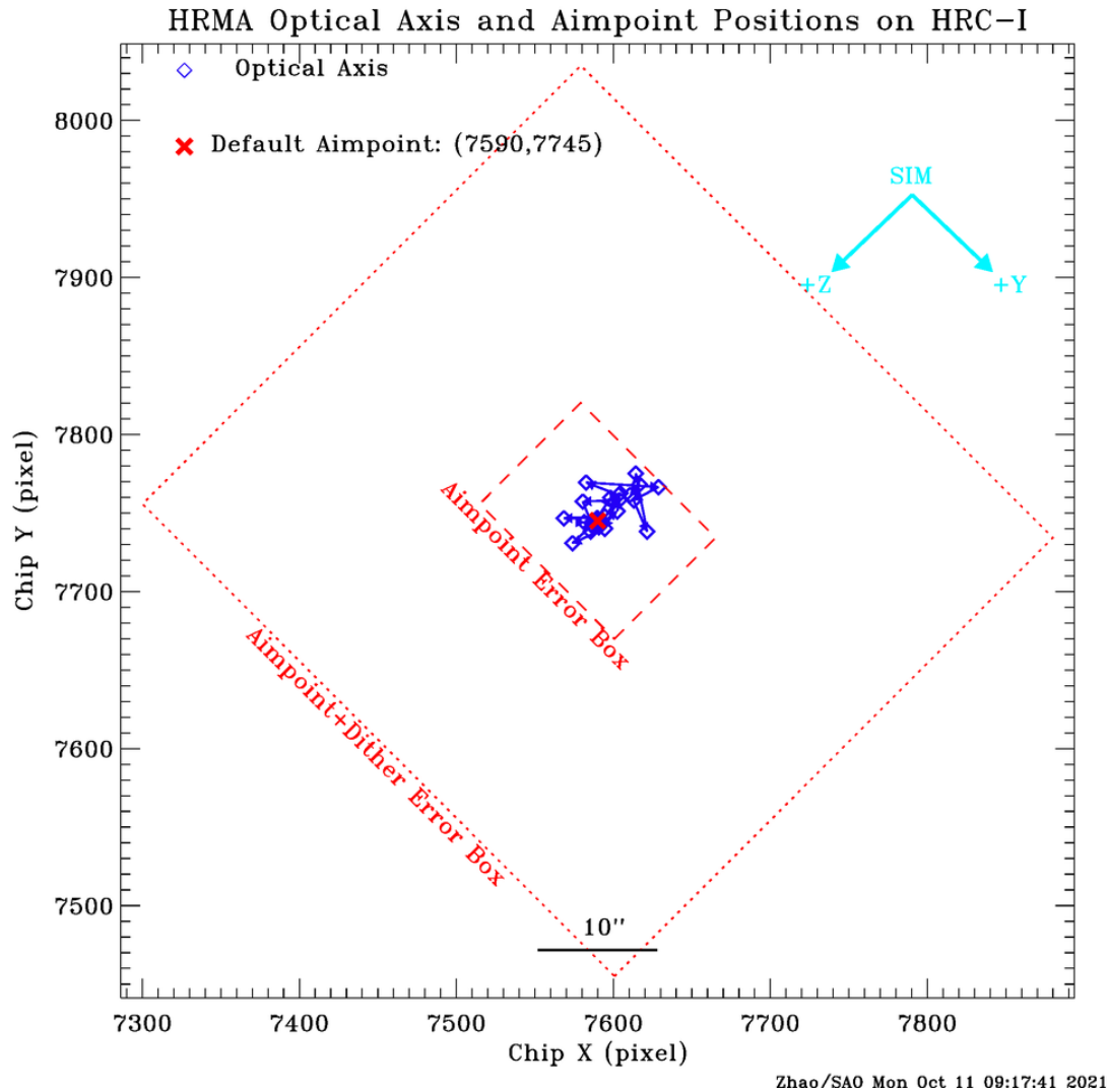
Figure 4.32: Chandra optical axis (blue diamonds) positions for each year and permanent default aimpoint (red cross) on HRC-I at [7590,7745]. The small box (red dashed line, 16 \text{ arcsec} \times 12 \text{ arcsec} , or 121.4 \times 91.1 pixels in SIM [Y, Z]) centered at the permanent default aimpoint is the error box of the effective aimpoint center, i.e. an on-axis target can be anywhere inside this box. The large box (red dotted line, 56 \text{ arcsec} \times 52 \text{ arcsec} , or 425.0 \times 394.7 pixels in SIM [Y, Z]) is the error box of effective aimpoint with dither.
