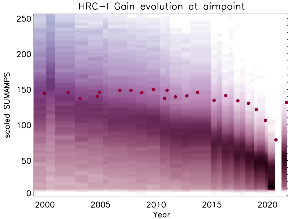
Figure 7.8: Gain decline on the HRC-I. The distribution of the scaled sum of the amplifier signals (scaled SUMAMPS) at each year, obtained from AR Lac observations at the aimpoint, is shown as vertical shaded stripes using square-root scaling. Higher values are shown as darker. Note the steady decline in the mode of the scaled SUMAMPS distribution with time; the distribution narrows and shrinks towards zero, until the voltage increase in early 2021 that causes the distribution to rebound to c.2015 levels. The red points mark the gain-corrected average PI. Notice that the multiplicative gain correction is not as effective at correcting for the gain decline as during earlier in the mission; efforts are underway to implement a more complex correction function. The gain maps available in the CALDB renormalize the scaled SUMAMPS distributions across the detector and over time to match that obtained in 1999-Oct.
