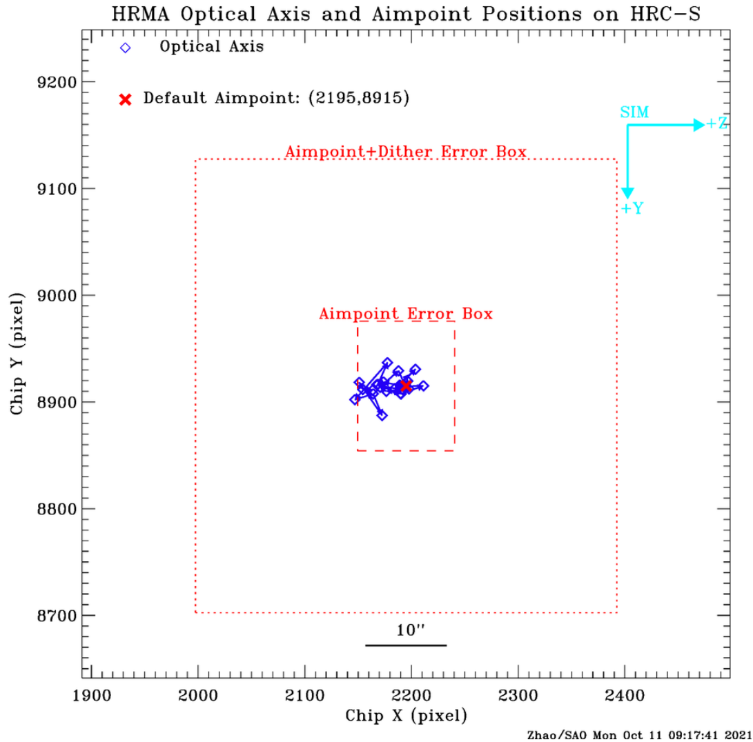
Figure 4.32: Chandra optical axis (blue diamonds) positions for each year and permanent default aimpoint (red cross) on HRC-S at [2195,8915]. The small box (red dashed line, 12 \text{ arcsec} \times 16 \text{ arcsec} , or 91.1 \times 121.4 pixels) centered at the permanent default aimpoint is the error box of the effective aimpoint center, i.e. an on-axis target can be anywhere inside this box. The large box (red dotted line, 52 \text{ arcsec} \times 56 \text{ arcsec} , or 394.7 \times 425.0 pixels) is the error box of effective aimpoint with dither.
