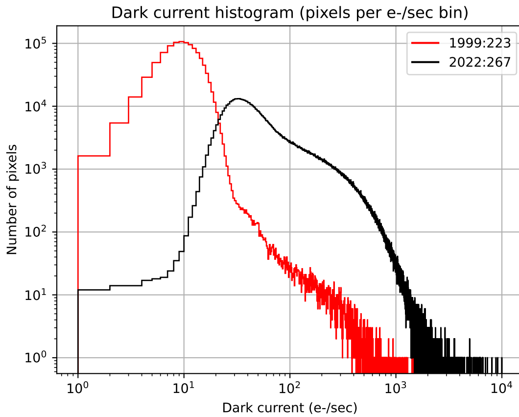
Figure 5.8: Differential histogram of dark current distribution for the ACA CCD in 1999-Aug and 2022-Oct
