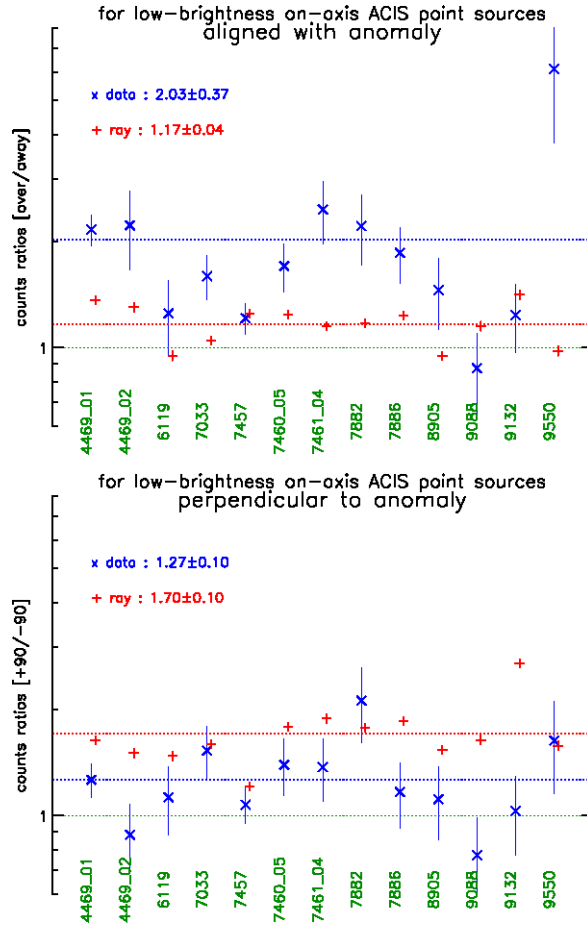
Figure 4.18: The ratio of counts collected from different segments around the PSF for a number of low-count-rate on-axis point sources (see Kashyap 2010). These are sources for which pile-up effects are minimal, and which have no previously known intrinsic features. The counts are collected in pie-shaped regions over and away from the anomaly (top; see Figure 4.17) and from similar regions rotated \pm 90^\circ from them (bottom). The ratios for counts are shown for both the data (‘x’; blue points) and raytrace (‘+’; red points). The error bars are shown as thin vertical lines. The average of the ratios computed for all the sources are also shown, along with the standard errors on the mean. There is a clear asymmetry in the PSF profile of the data along the nominal direction of the anomaly that is neither present in the perpendicular direction, nor accountable by raytraces. Comparison with the raytrace model PSFs is necessary to establish the reality of the anomaly, since the Chandra PSF is not azimuthally symmetrical and displays intrinsic asymmetries. See, for instance, the ratios along the perpendicular direction, in the lower figure, where they are higher for the raytrace model than for the data, signifying that there are as yet unexplained differences between the data and the raytrace model. The mechanism by which these discrepancies arise is under investigation.
