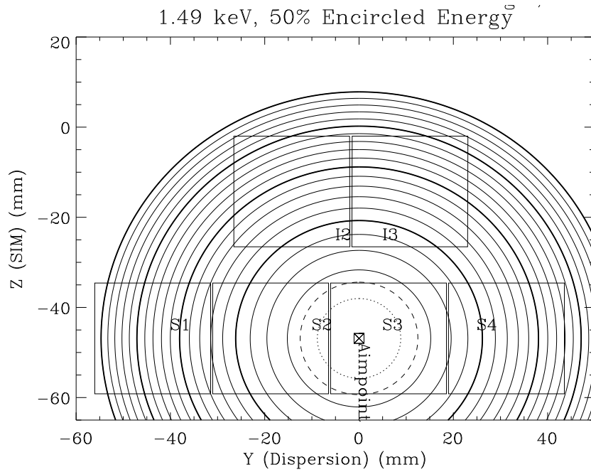
Figure 6.18: Approximate contours of constant 50% encircled energy at 1.49 keV when the ACIS-S aimpoint is selected. The dotted circle is 1 arcsec. That is, the 50% encircled energy at 1.49 keV at any point on the dotted circle is 1 arcsec. Similarly, the dashed circle is 1.5 arcsec. The remainder are at 1 arcsec intervals. The thicker solid circles highlight the 5, 10, 15, and 20 arcsec contours.
