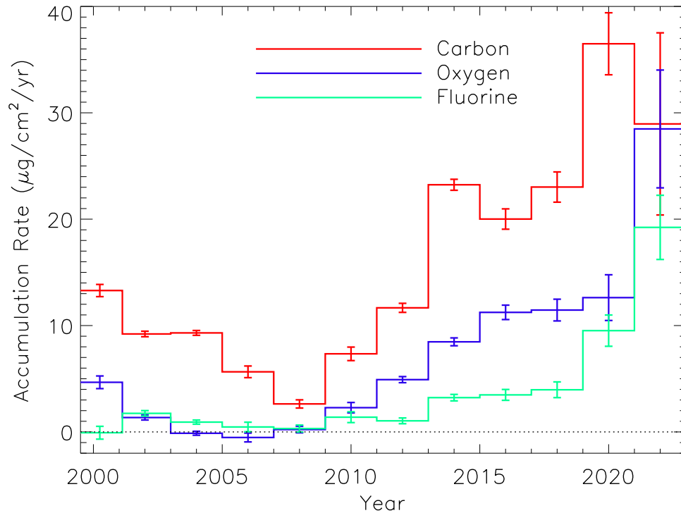
Figure 6.10: The accumulation rate for C, O, and F over the Chandra mission as measured by LETG/ACIS-S observations of blazars.
