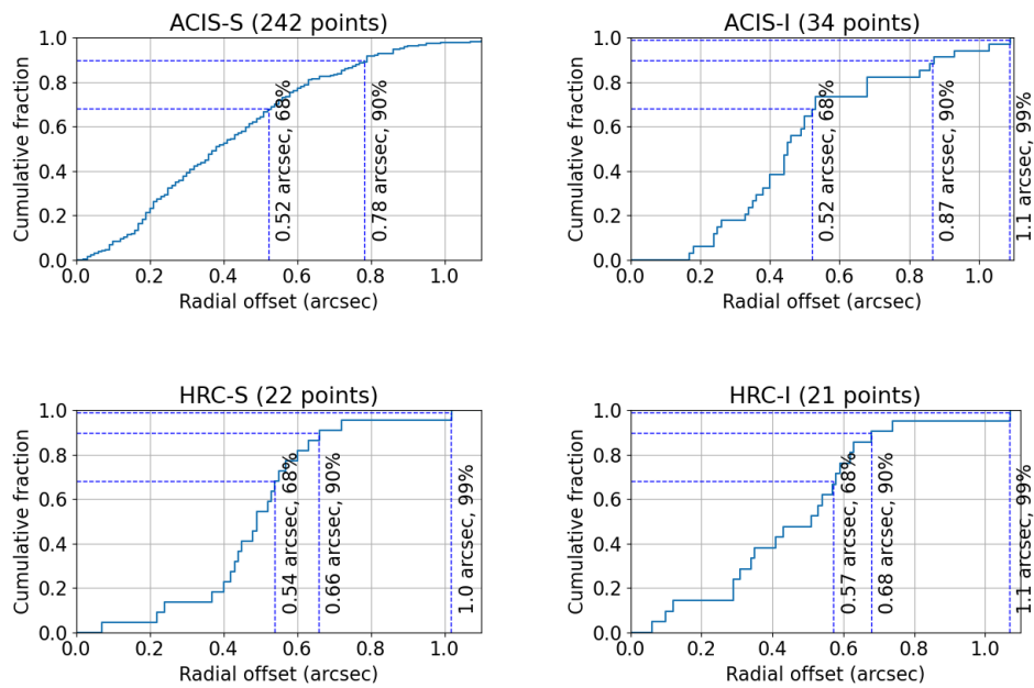
Figure 5.4: Cumulative histogram of celestial accuracy for Chandra X-ray source locations for each SI using observations since 2017-Oct. Radial offset is the distance in arcsec between the optical coordinate, typically from the Tycho-2 catalog, and the Chandra position.
