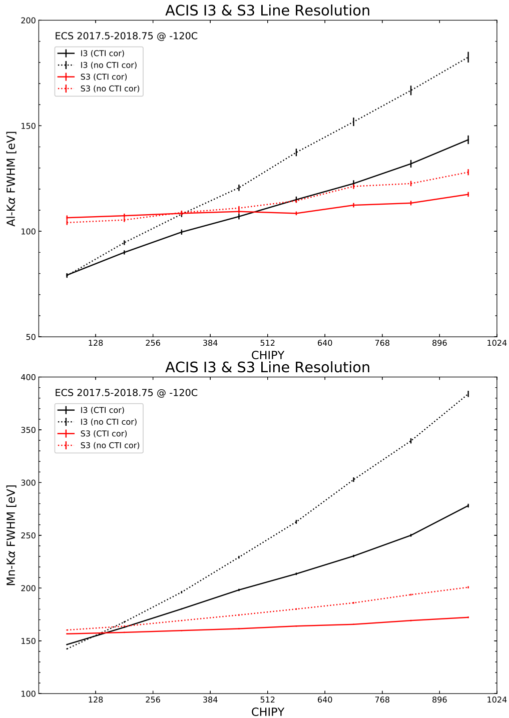
Figure 6.15: Energy resolution (FWHM in eV) versus row number (CHIPY) for several cases is plotted. The top plot shows Aluminum K\alpha (1.49 keV), while the bottom plot is for Manganese K\alpha (5.9 keV). The resolution of the I3 chip, with and without CTI correction) is shown by the black curves, and the S3 resolution is shown by the red curves.
