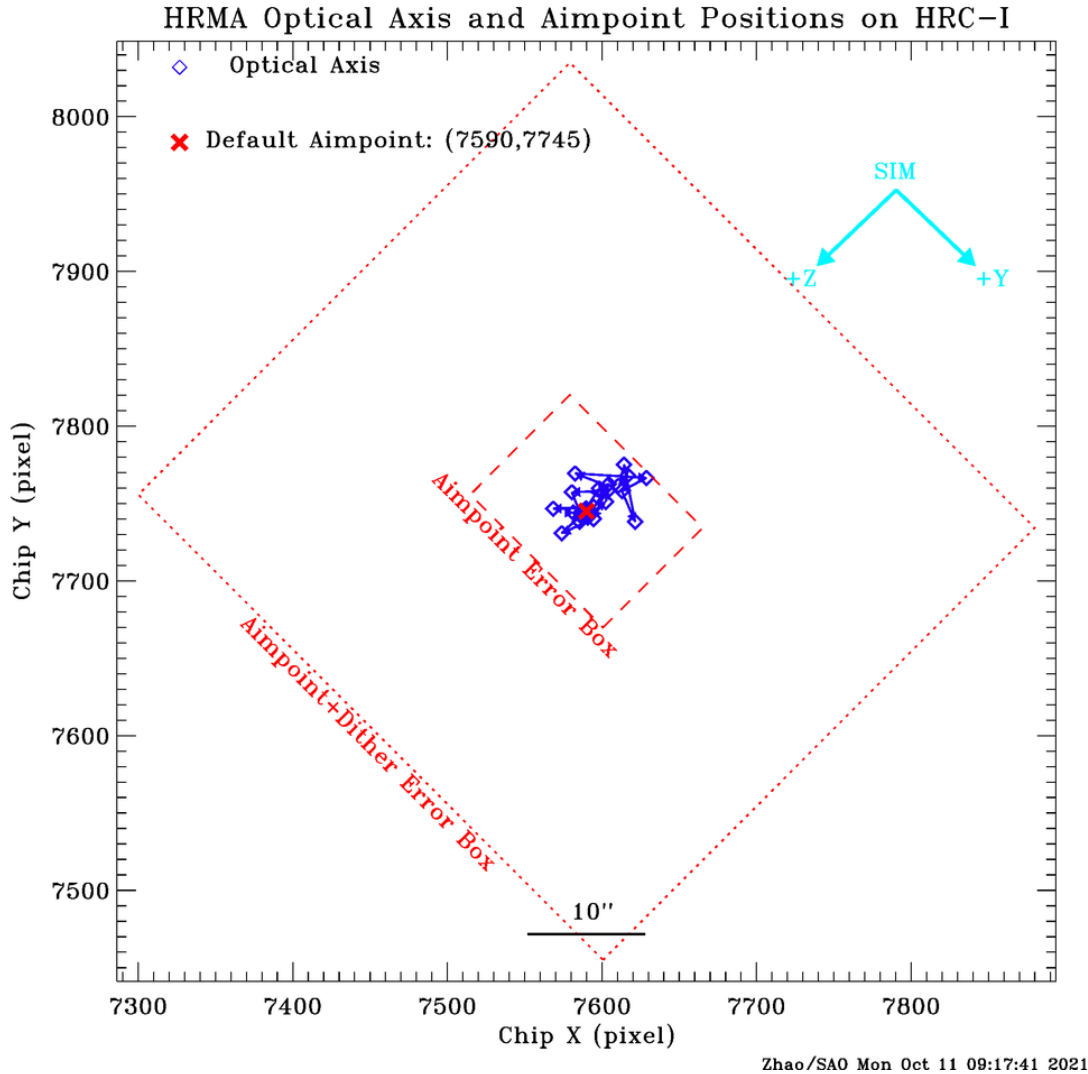
Figure 4.29: Chandra optical axis (blue diamonds) positions for each year and permanent default aimpoint (red cross) on HRC-I at [7590,7745]. The small box (red dashed line, 16 arcsec \times 12 arcsec, or 121.4 \times 91.1 pixels in SIM [Y, Z]) centered at the permanent default aimpoint is the error box of the effective aimpoint center, i.e. an on-axis target can be anywhere inside this box. The large box (red dotted line, 56 arcsec \times 52 arcsec, or 425.0 \times 394.7 pixels in SIM [Y, Z]) is the error box of effective aimpoint with dither.
