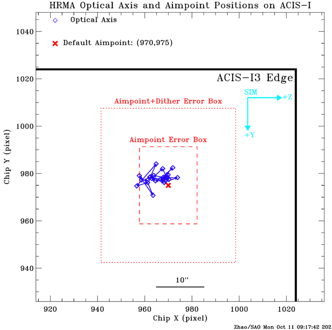
Figure 4.27: Chandra optical axis (blue diamonds) positions for each year and permanent default aimpoint (red cross) on ACIS-I at [970,975]. The small box (red dashed line, 12 arcsec \times 16 arcsec, or 24.4 \times 32.5 pixels) centered at the permanent default aimpoint is the error box of the effective aimpoint center, i.e. an on-axis target can be anywhere inside this box. The large box (red dotted line, 28 arcsec \times 32 arcsec, or 56.9 \times 65.0 pixels) is the error box of effective aimpoint with dither.
