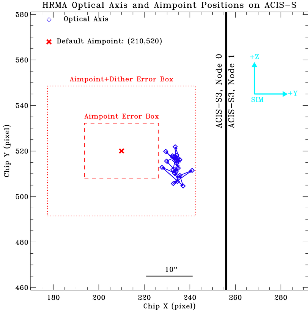
Figure 4.28: Chandra optical axis (blue diamonds) positions for each year and permanent default aimpoint (red cross) on ACIS-S at [210,520]. The small box (red dashed line, 16 arcsec \times 12 arcsec, or 32.5 \times 24.4 pixels) centered at the permanent default aimpoint is the error box of the effective aimpoint center, i.e. an on-axis target can be anywhere inside this box. The large box (red dotted line, 32 arcsec \times 28 arcsec, or 65.0 \times 56.9 pixels) is the error box of effective aimpoint with dither. Note the permanent default aimpoint is \sim 12 arcsec from the optical axis in order to avoid the node boundary 0|1.
