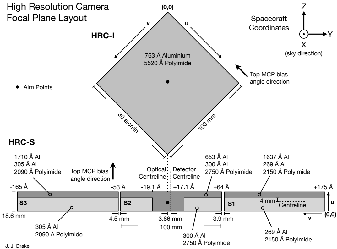
Figure 7.1: A schematic of the HRC focal-plane geometry as viewed along the optical axis from the telescope towards the focal plane. See http://hea-www.harvard.edu/HRC/calib/hrccalib_a_180998.ps
