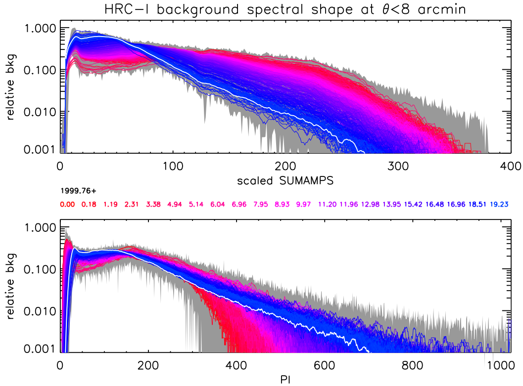
Figure 7.14: The shape of the background spectrum varies with time on both the HRC-I and HRC-S. This plot shows the spectra of both the scaled SUMAMPs (top panel) and Pulse Invariant channels (PI; bottom panel), color coded by years into the mission (red is early, blue is current). The spectral shapes are obtained from the central 8 arcmin region of the HRC-I during regular AR Lac calibration observations, with the source photons and observations affected by high background excluded. The grey shaded region represents the full envelope, and the individual curves are the smoothed spectra, normalized by total counts and rescaled to a sample maximum of 1. The white curves represent the latest observations prior to the voltage change.
