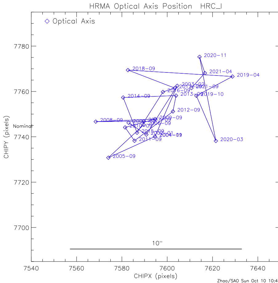
Figure 4.25: Chandra optical axis positions on HRC-I since launch. Each position is labeled by the year-month. The optical axis position is very stable and well within a 10 arcsec region.
