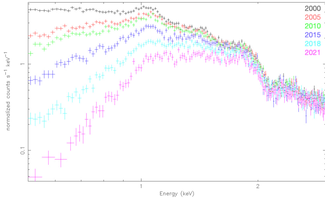
Figure 6.8: ACIS-S spectrum of the galaxy cluster Abell 1795 at six different epochs ranging from 2000 to 2021. The decreasing count rates in the spectrum of a stable calibration source demonstrate the loss of effective area due to the build-up of the contaminant on the ACIS OBF.
