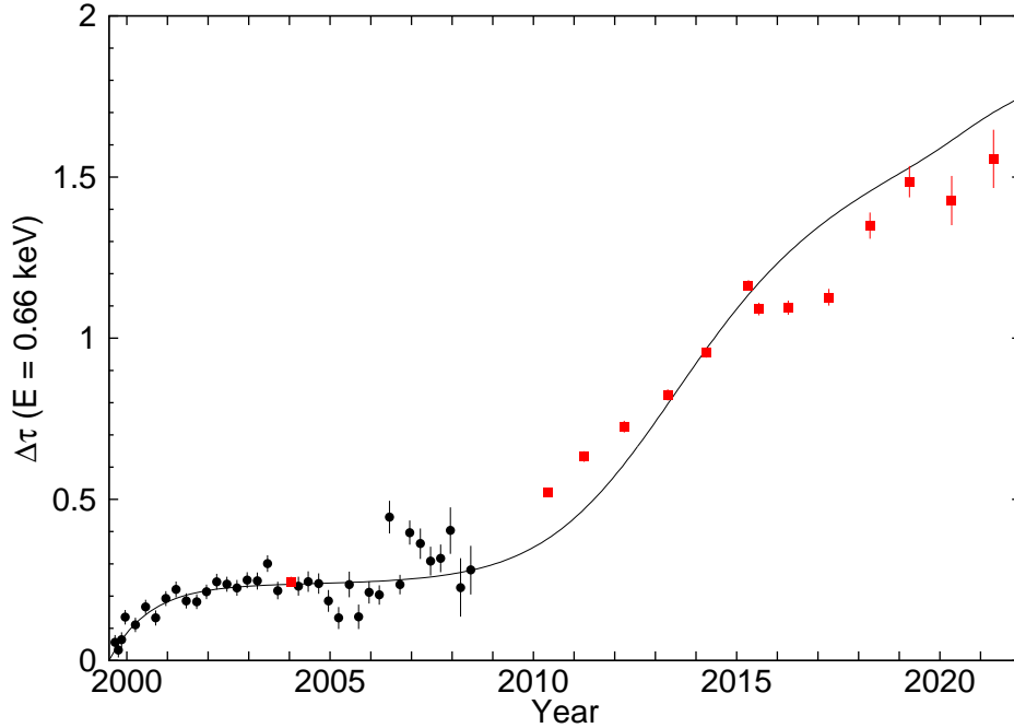
Figure 6.9: The difference between the optical depth at 0.66 keV measured near the center of the ACIS-S chip S3 and that measured near the readout at the edge of the same chip is shown against time. Black circles are measurements made using the ECS data and red squares are made from observations of the galaxy cluster Abell 1795. The solid curve shows the optical depth of the contaminant as modeled in the most recent contamination model.
