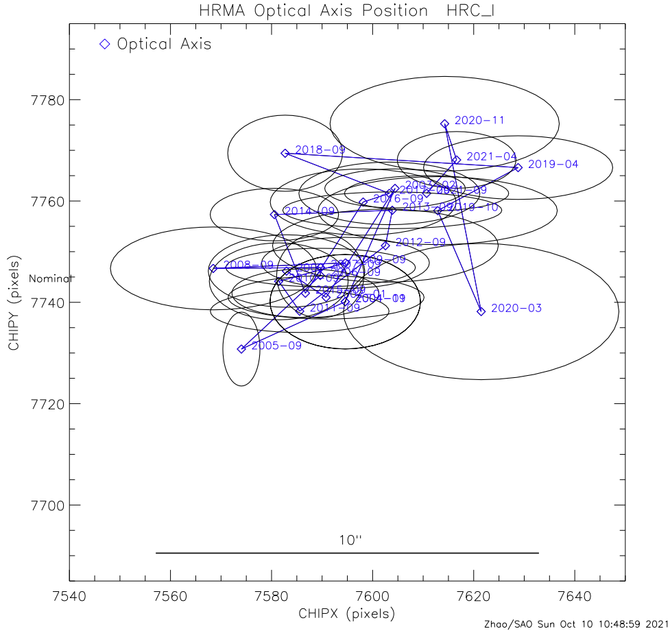
Figure 4.26: The same as Figure 4.25, with the 1\text{-}\sigma measurement error ellipse around each position for that given year. The drift of optical axis position is consistent with the measurement errors.
