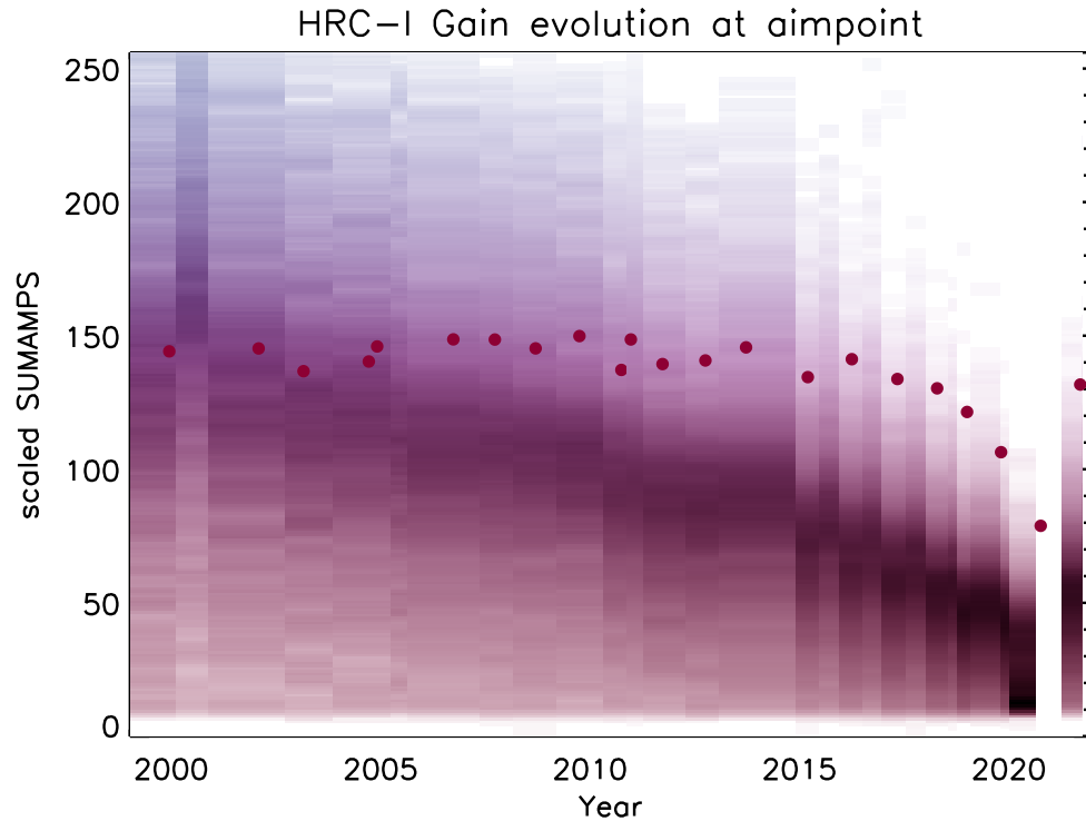
Figure 7.8: Gain decline on the HRC-I. The distribution of the scaled sum of the amplifier signals (scaled SUMAMPS) at each year, obtained from AR Lac observations at the aimpoint, is shown as vertical shaded stripes using square-root scaling. Higher values are shown as darker. Note the steady decline in the mode of the scaled SUMAMPS distribution with time; the distribution narrows and shrinks towards zero, until the voltage increase in early 2021 that causes the distribution to rebound to c.2015 levels. The red points mark the gain-corrected average PI. Notice that the multiplicative gain correction is not as effective at correcting for the gain decline as during earlier in the mission; efforts are underway to implement a more complex correction function. The gain maps available in the CALDB renormalize the scaled SUMAMPS distributions across the detector and over time to match that obtained in 1999-Oct.
