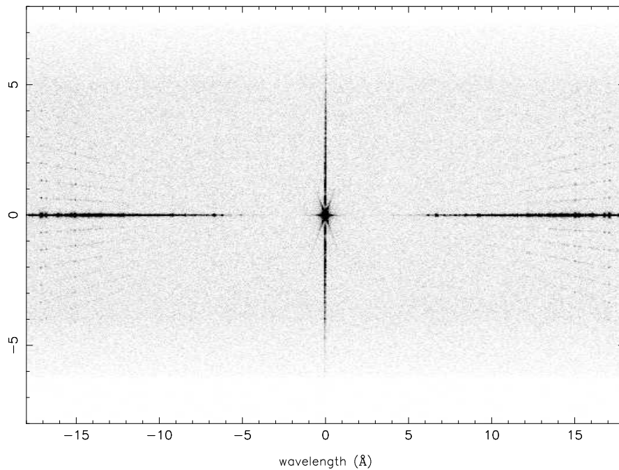
Figure 9.23: HRC-S detector image of LETGS observation of Capella. Vertical axis is stretched by a factor of 1.6 relative to horizontal; only the central 30 mm of the central plate is shown. The full extent of the telemetered six-tap cross-dispersion window is shown and measures 9.9 mm. The areas of reduced background at top and bottom are due to dither effects. Star-shaped coarse support structure diffraction is seen around zeroth order, and “cat’s whiskers” fine support structure diffraction is seen above and below the primary dispersion axis, as well as in the vertical line through zeroth order.
