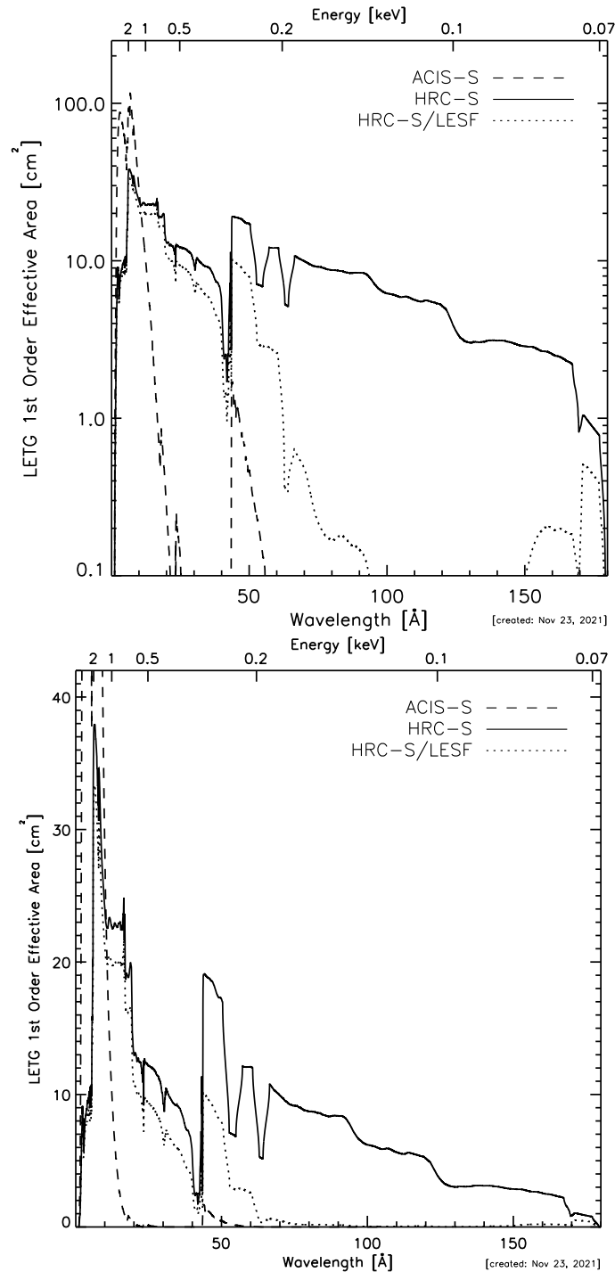
Figure 9.17: LETGS 1st-order effective area for an on-axis point source, with HRC-S, HRC-S/LESF, and ACIS-S detector configurations with log (top) and linear (bottom) scaling. Positive and negative orders are summed. LETG+ACIS-S areas include the effects of time-dependent contamination. Note that the vertical scale of the linear plot has been truncated.
