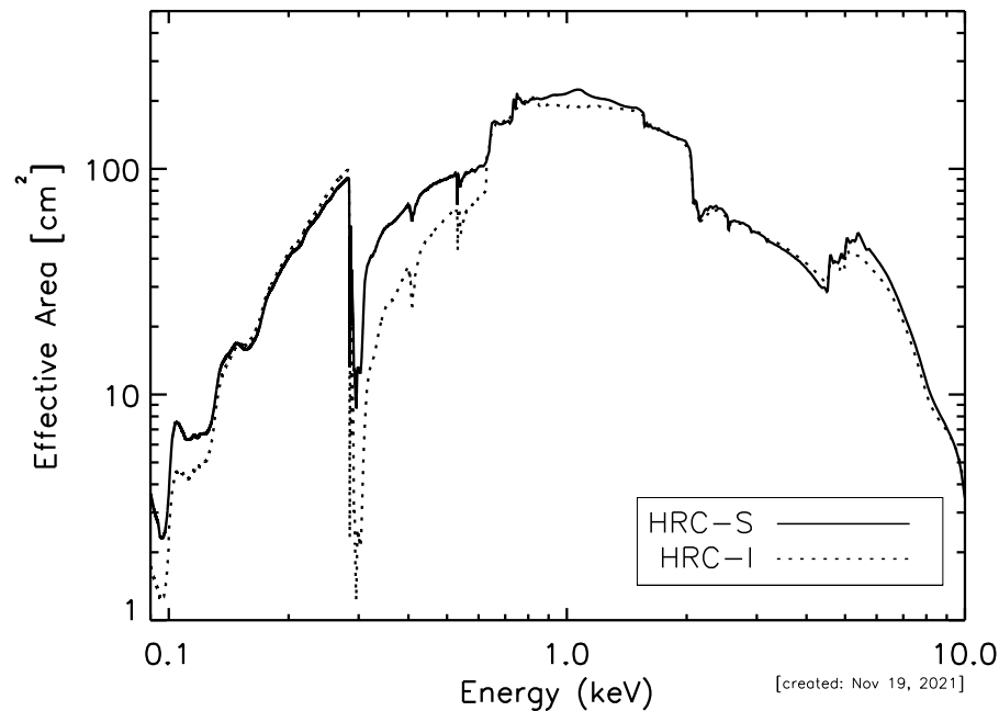
Figure 7.11: The effective area of the HRMA/HRC-I (dashed line) and the central segment of the HRMA/HRC-S in imaging mode (solid line) integrated over the full PSF. Absorption edges are due to the iridium coating on the mirrors, the CsI MCP coating, and the polyimide/Al of the UVIS.
