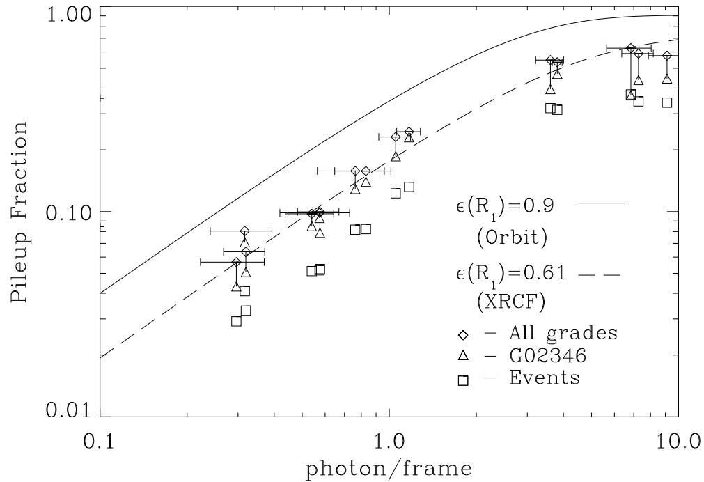
Figure 6.24: The pile-up fraction as a function of the the counting rate (in the absence of pile-up in units of photons/frame). The solid line is for on-orbit, the dashed line and the data points are for, and from, ground-based data respectively. The difference between the ground and flight functions are a consequence of the improved PSF on-orbit, where gravitational effects are negligible – see Chapter 4. Note that when pile-up occurs there are two or more photons for each event, so the fraction of events with pile-up is always less than the fraction of photons with pile-up.
