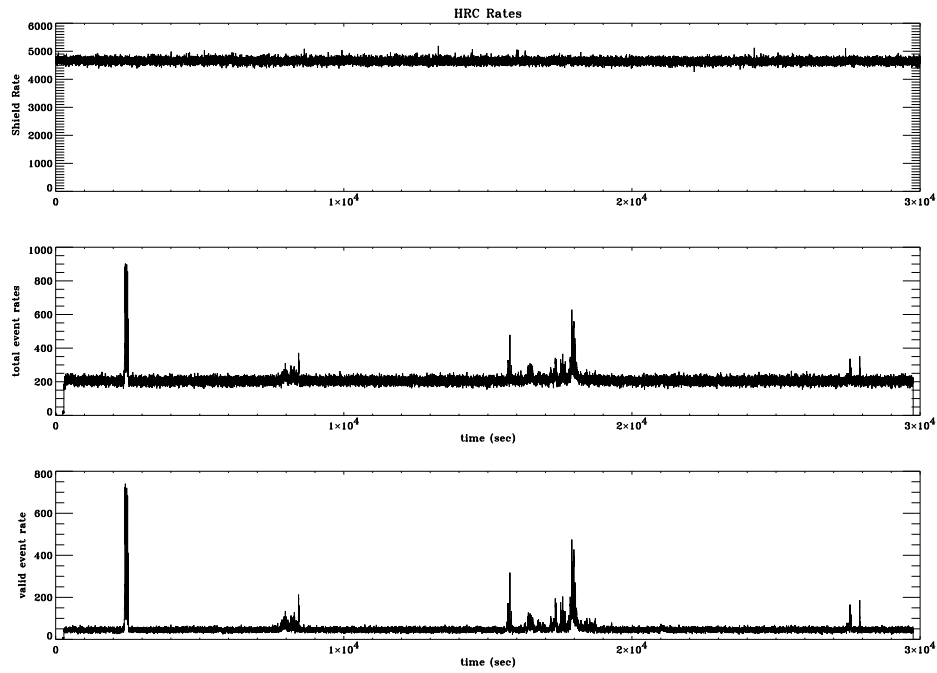
Figure 7.12: An example of the background variability during a \sim 30 ks HRC-I observation of the SNR G21.5-09 taken on 1999-Oct-25. The total event rate (middle) and valid event rate (bottom) show correlated bursts up to \sim 800 cts s -1 . The bursts are uniformly distributed over the detector. The anti-coincidence shield (top) exhibits no correlated enhancements. The total and valid rates differ by \sim 200 cts s -1 due primarily to cosmic ray events that are vetoed and don't appear as valid events in the telemetry.
