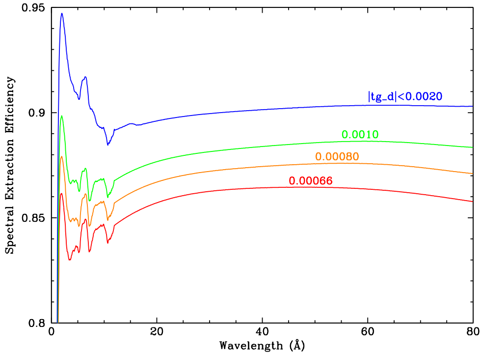
Figure 9.15: Spectral extraction efficiencies for LETG+ACIS for various extraction region half-widths ( tg\_d units are deg). The default spectral extraction region is |tg\_d| < 0.0008 deg. Approximately 10% of the total power is diffracted by the fine-support structure and most of it falls outside the extraction region; the peaks toward shorter wavelengths reflect the inclusion of progressively higher orders of cross-dispersed events within the extraction region. The otherwise general trend of declining efficiency toward short wavelengths is caused by increased scattering. The slight fall-off beyond \sim 60 Å is due to astigmatism, i.e., an increasing fraction of events are lost as the dispersion pattern broadens (see Figure 9.14).
