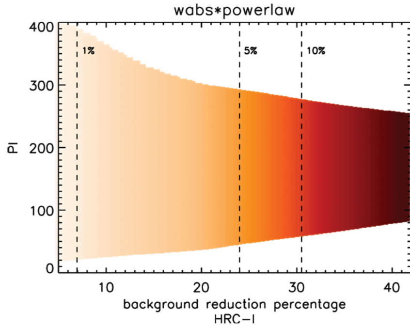
Figure 7.15: An estimate of the range of PI values that should be included to reduce the background by a given percentage is shown in the figure as a shaded band for sources with absorbed power-law spectra. (see https://cxc.cfa.harvard.edu/ciao/threads/hrci_bg_spectra/ ). The depth of the shading indicates how much of the source events are expected to be lost. The vertical dashed lines indicate the background reduction for source event losses of 1%, 5%, and 10%. As shown in Figure 7.14, the background varies with time. Here, for the sake of definiteness, we use the background from the year 2008.
