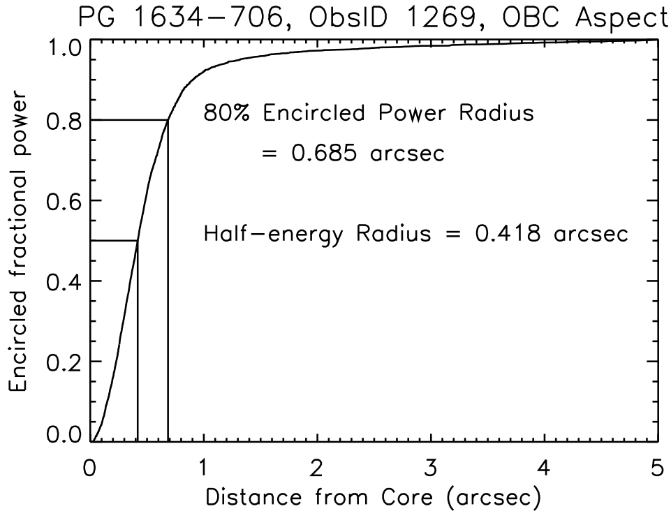
Figure 6.12: The on-orbit encircled broad-band energy versus radius for an ACIS observation of point source PG1634-706 (ObsID 1269). The curve is normalized to unity at a radius of 5 arcsec. The statistical uncertainty is estimated to be 3%, and the systematic uncertainty due to power beyond 5 arcsec is 2%. The effective energy is 1 keV.
