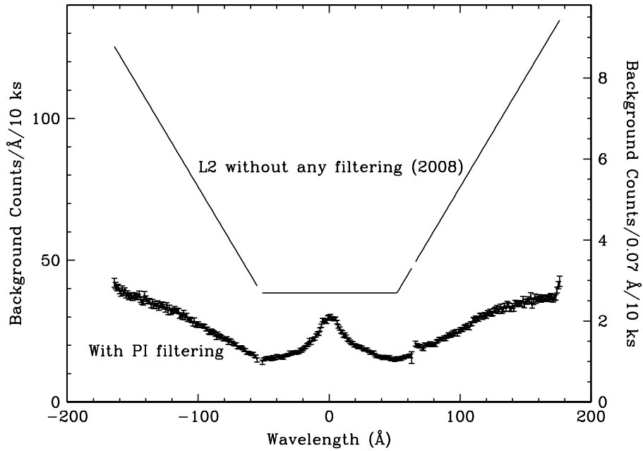
Figure 9.22: The 2008-Jan LETG+HRC-S background rate with and without pulse-height (PI) filtering. These Level 2 rates correspond to 1.1 \times 10^{-6} cts s^{-1} pixel ^{-1} (see Figure 9.21). Data are shown using the standard ‘bowtie’ spectral extraction region (see Figure 9.14). X-ray losses from the observed spectrum as a result of the filtering for 1st order are \sim 1.0\% ; losses will be somewhat larger for higher orders. See https://cxc.harvard.edu/cal/Letg/Hrc.bg for more information.
