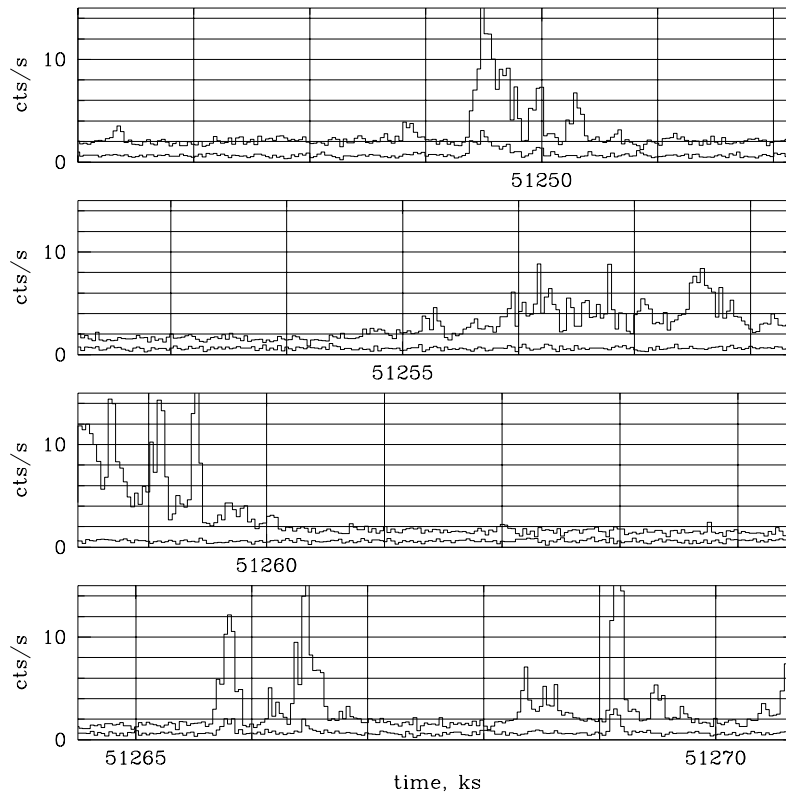
Figure 6.31: An example of the ACIS background counting rate versus time – BI chip (S3; top curve) and an FI chip (I2; bottom curve). These are for the standard grades and the band from 0.3 - 10 keV.
