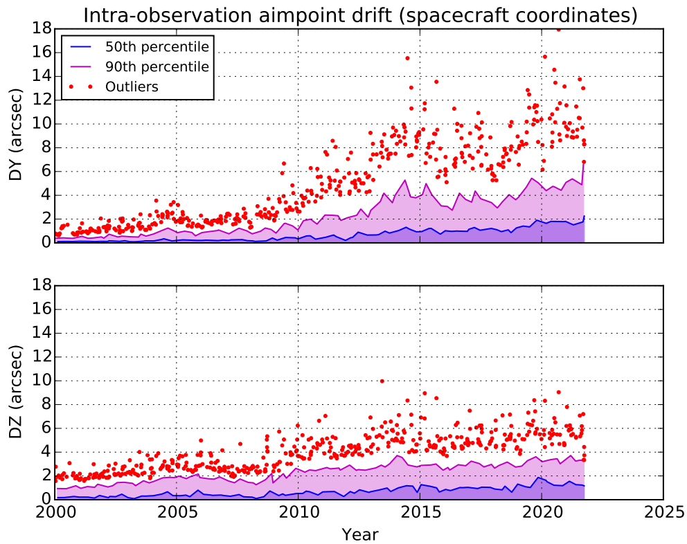
Figure 5.6: Peak to peak aimpoint drift within individual science observations. This figure shows that total intra-observation drift ( DY+DZ ) up to 6 arcsec during observations is possible and, in rare cases, drift over 15 arcsec can occur.
