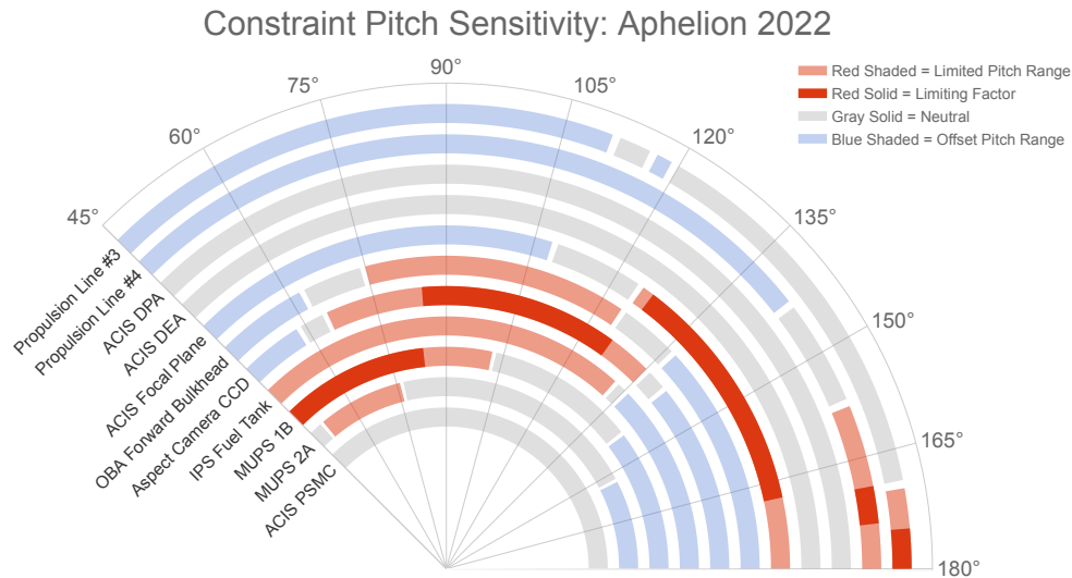
Figure 3.5: Illustration of the thermal impact of solar pitch angle on various spacecraft components. Pale red arcs indicate pitch ranges in which it is more difficult to maintain the component within its thermal restrictions, gray arcs show where components are thermally neutral, and pale blue arcs indicate pitch ranges in which components can recover from time spent in thermally limited pitch regions. Dark red arcs indicate where a component represents the most limiting dwell time restriction at a given pitch angle; the MUPS at low pitch angles, ACA at mid-pitch, ACIS at high pitch, and the propulsion lines at the highest pitch angles. Note that the diagram represents the predicted status during 2022 with ACIS at the focus; thermal constraints will change over time so it should not be used as a guide for planning specific observations. For detailed inquiries regarding pitch sensitivity, please contact the Chandra helpdesk.
