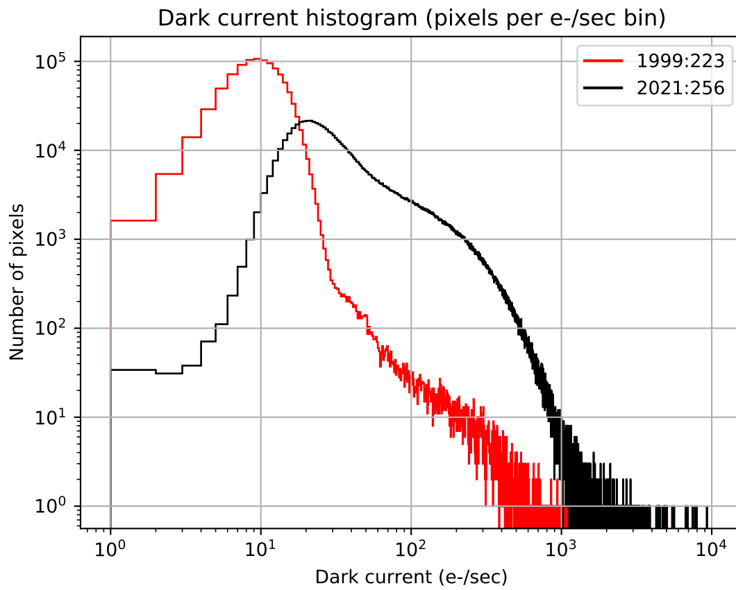
Figure 5.8: Differential histogram of dark current distribution for the ACA CCD in 1999-Aug and 2021-Sep
