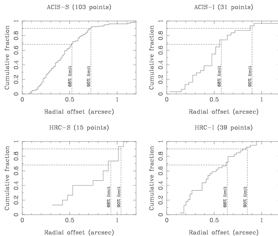
Figure 5.4: Cumulative histogram of celestial accuracy for Chandra X-ray source locations for each SI using observations since 2015-Nov. Radial offset is the distance in arcsec between the optical coordinate, typically from the Tycho-2 catalog, and the Chandra position.
