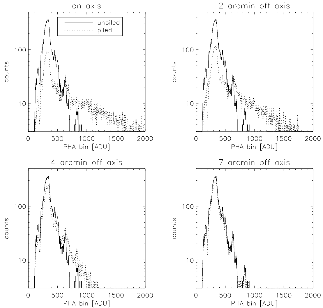
Figure 6.23: MARX simulations of the effect of pile-up on the shape of the spectrum. The true (solid line) and the detected (dotted line) spectra are shown for four different viewing angles. The corresponding “pile-up fractions” – see Section 6.16.2 – are 46%, 40%, 15%, and 2% as the image is moved progressively further off-axis.
