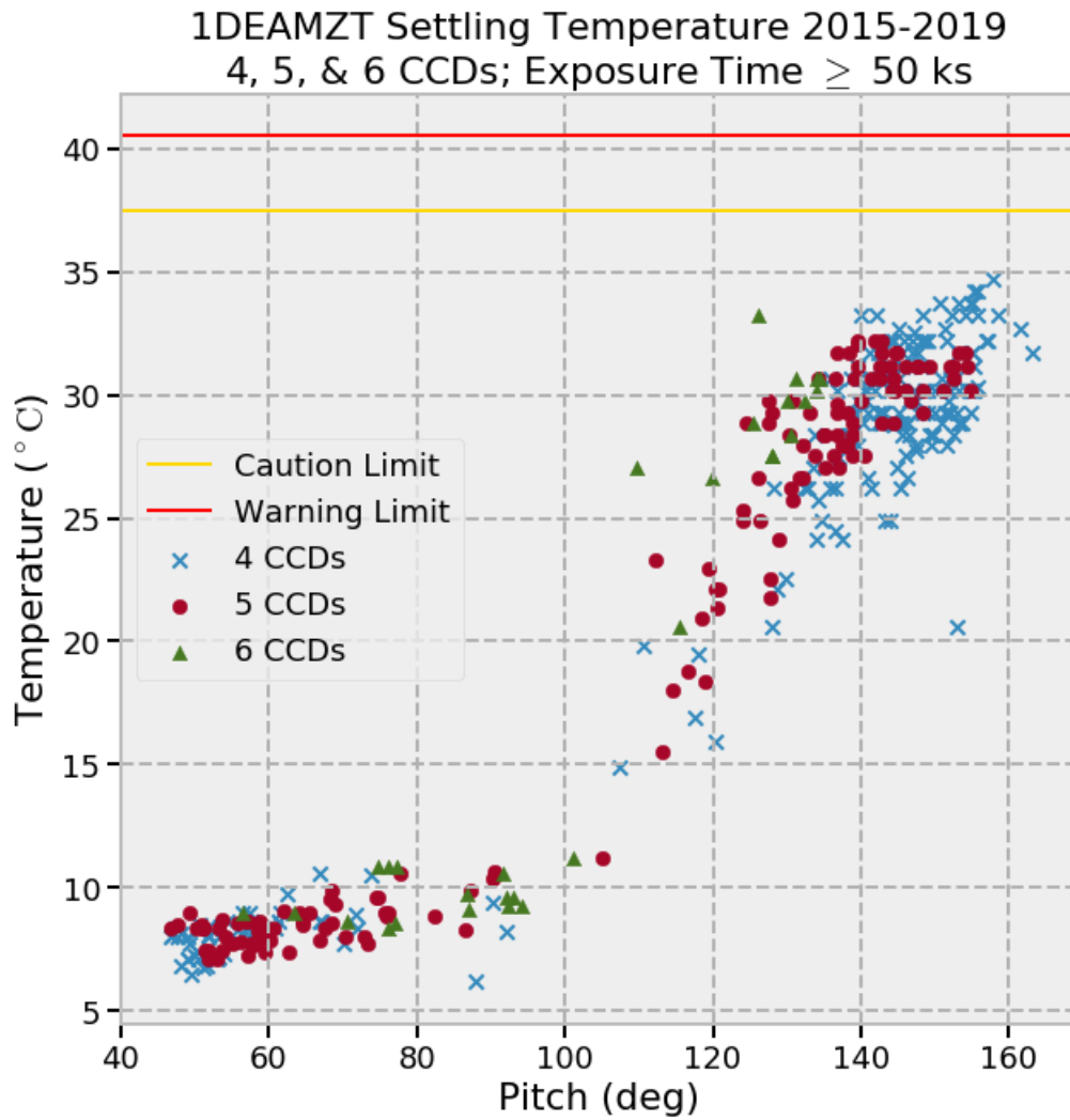
Figure 6.35: DEA temperature as a function of spacecraft pitch angle. 6 CCD observations are indicated by green-filled triangles, 5 CCD observations by red-filled circles and 4 CCD observations are indicated by blue \times s.
