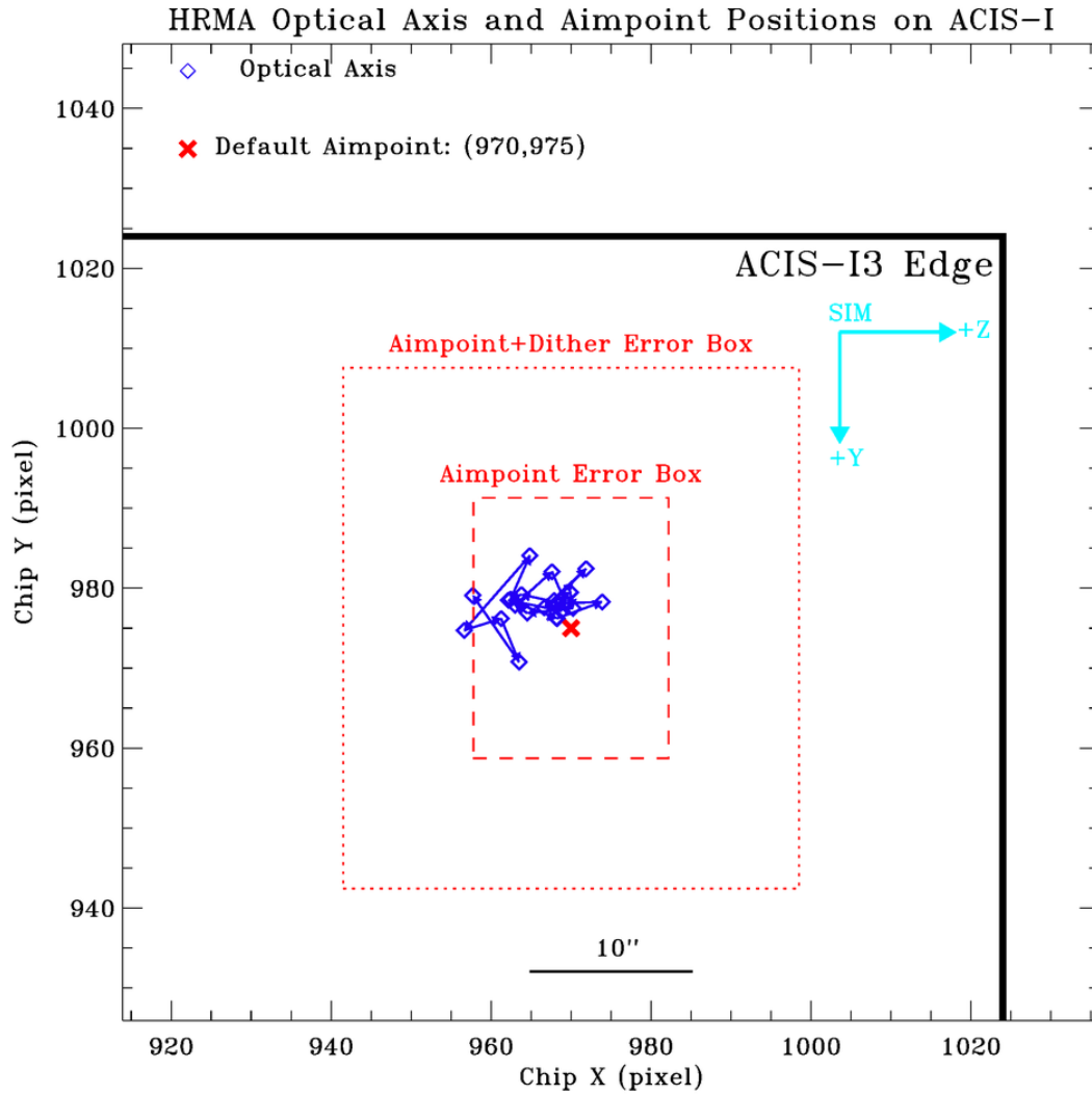
Figure 4.26: Chandra optical axis (blue diamonds) positions for each year and permanent default aimpoint (red cross) on ACIS-I at [970,975]. The small box (red dashed line, 12 arcsec \times 16 arcsec, or 24.4 \times 32.5 pixels) centered at the permanent default aimpoint is the error box of the effective aimpoint center, i.e. an on-axis target can be anywhere inside this box. The large box (red dotted line, 28 arcsec \times 32 arcsec, or 56.9 \times 65.0 pixels) is the error box of effective aimpoint with dither.
