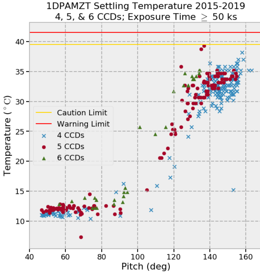
Figure 6.34: DPA temperature as a function of spacecraft pitch angle. 6 CCD observations are indicated by green-filled triangles, 5 CCD observations by red-filled circles and 4 CCD observations are indicated by blue \times s.
