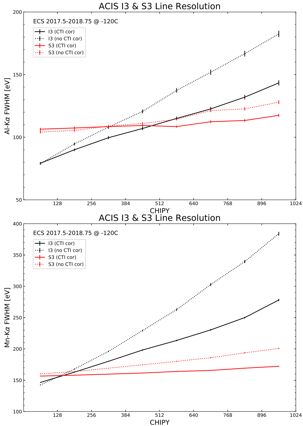
Figure 6.13: Energy resolution (FWHM in eV) versus row number (CHIPY) for several cases is plotted. The top plot shows Aluminum K \alpha (1.49 keV), while the bottom plot is for Manganese K \alpha (5.9 keV). The resolution of the I3 chip, with and without CTI correction) is shown by the black curves, and the S3 resolution is shown by the red curves.
