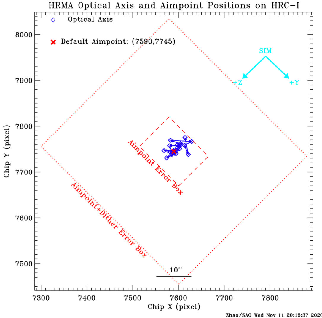
Figure 4.28: Chandra optical axis (blue diamonds) positions for each year and permanent default aimpoint (red cross) on HRC-I at [7590,7745]. The small box (red dashed line, 16 arcsec \times 12 arcsec, or 121.4 \times 91.1 pixels in SIM [Y, Z]) centered at the permanent default aimpoint is the error box of the effective aimpoint center, i.e. an on-axis target can be anywhere inside this box. The large box (red dotted line, 56 arcsec \times 52 arcsec, or 425.0 \times 394.7 pixels in SIM [Y, Z]) is the error box of effective aimpoint with dither.
