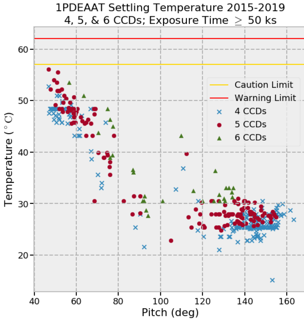
Figure 6.33: ACIS PSMC temperature as a function of spacecraft pitch angle. 6 CCD observations are indicated by green-filled triangles, 5 CCD observations by red-filled circles and 4 CCD observations are indicated by blue \times s.
