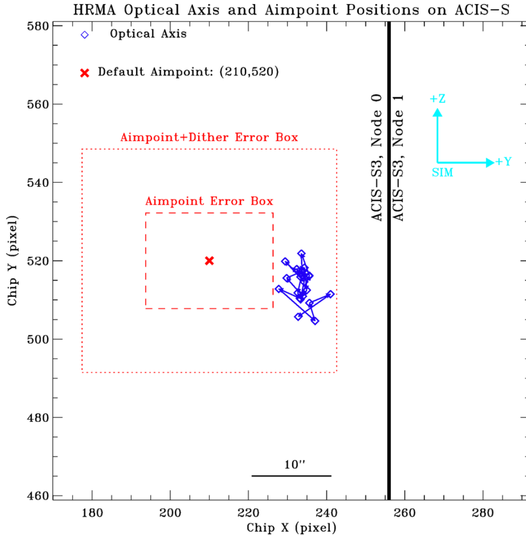
Figure 4.27: Chandra optical axis (blue diamonds) positions for each year and permanent default aimpoint (red cross) on ACIS-S at [210,520]. The small box (red dashed line, 16 arcsec \times 12 arcsec, or 32.5 \times 24.4 pixels) centered at the permanent default aimpoint is the error box of the effective aimpoint center, i.e. an on-axis target can be anywhere inside this box. The large box (red dotted line, 32 arcsec \times 28 arcsec, or 65.0 \times 56.9 pixels) is the error box of effective aimpoint with dither. Note the permanent default aimpoint is \sim 12 arcsec from the optical axis in order to avoid the node boundary 0|1.
