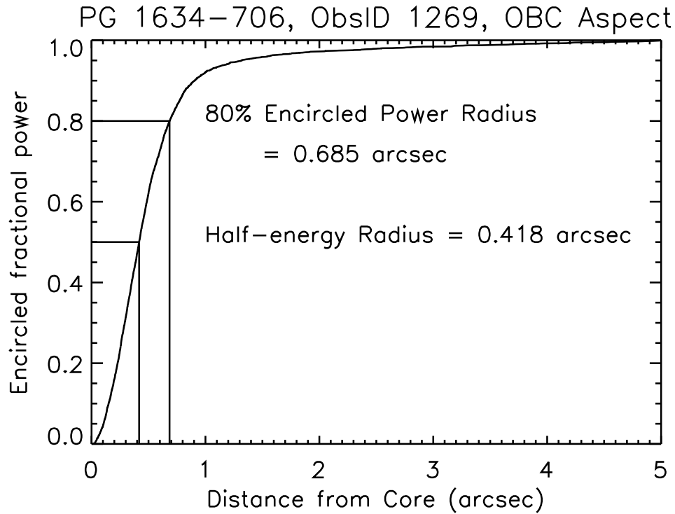
Figure 6.10: The on-orbit encircled broad-band energy versus radius for an ACIS observation of point source PG1634-706 (ObsID 1269). The curve is normalized to unity at a radius of 5 arcsec. The statistical uncertainty is estimated to be 3%, and the systematic uncertainty due to power beyond 5 arcsec is 2%. The effective energy is 1 keV.
