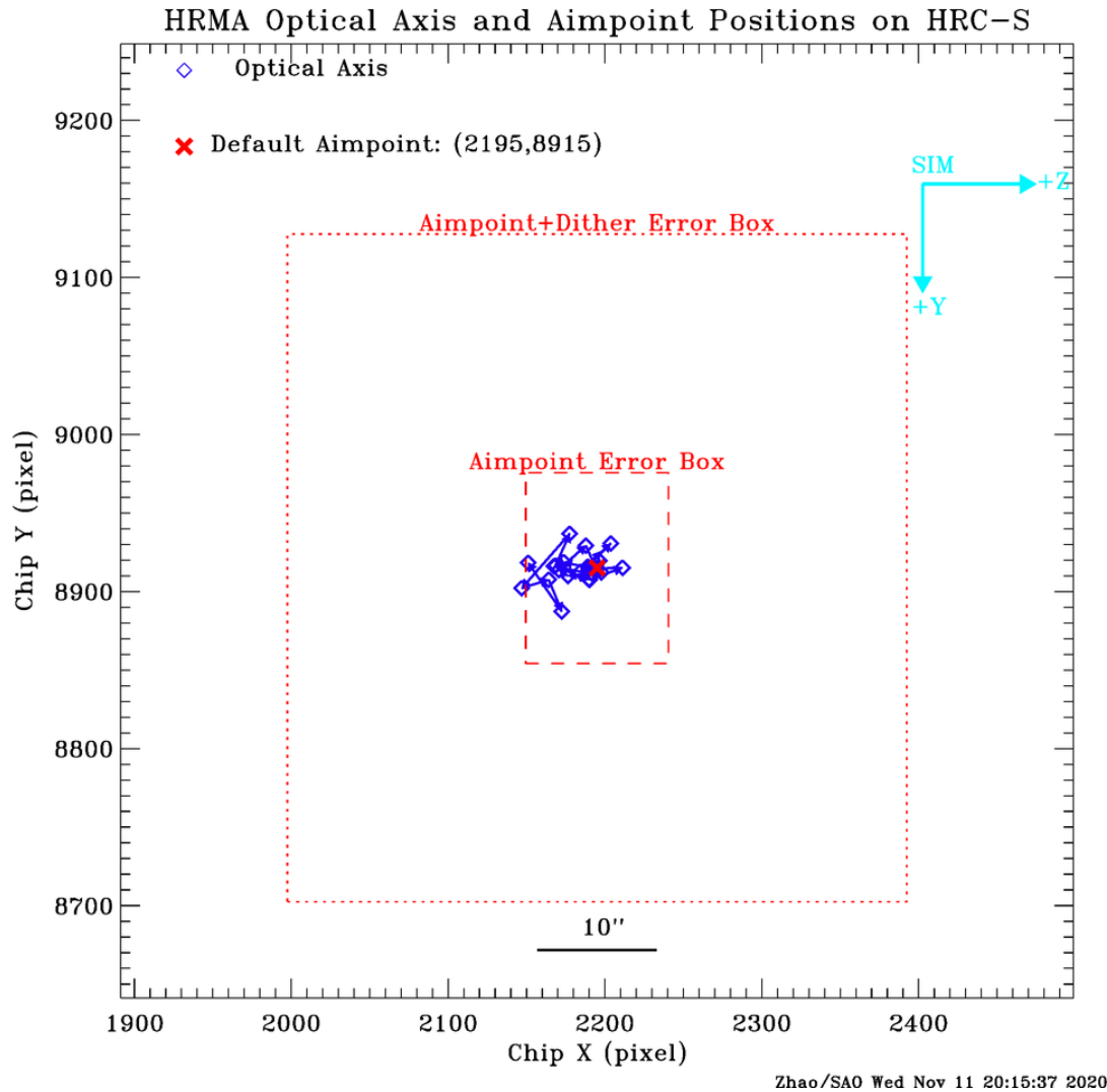
Figure 4.29: Chandra optical axis (blue diamonds) positions for each year and permanent default aimpoint (red cross) on HRC-S at [2195,8915]. The small box (red dashed line, 12 arcsec \times 16 arcsec, or 91.1 \times 121.4 pixels) centered at the permanent default aimpoint is the error box of the effective aimpoint center, i.e. an on-axis target can be anywhere inside this box. The large box (red dotted line, 52 arcsec \times 56 arcsec, or 394.7 \times 425.0 pixels) is the error box of effective aimpoint with dither.
