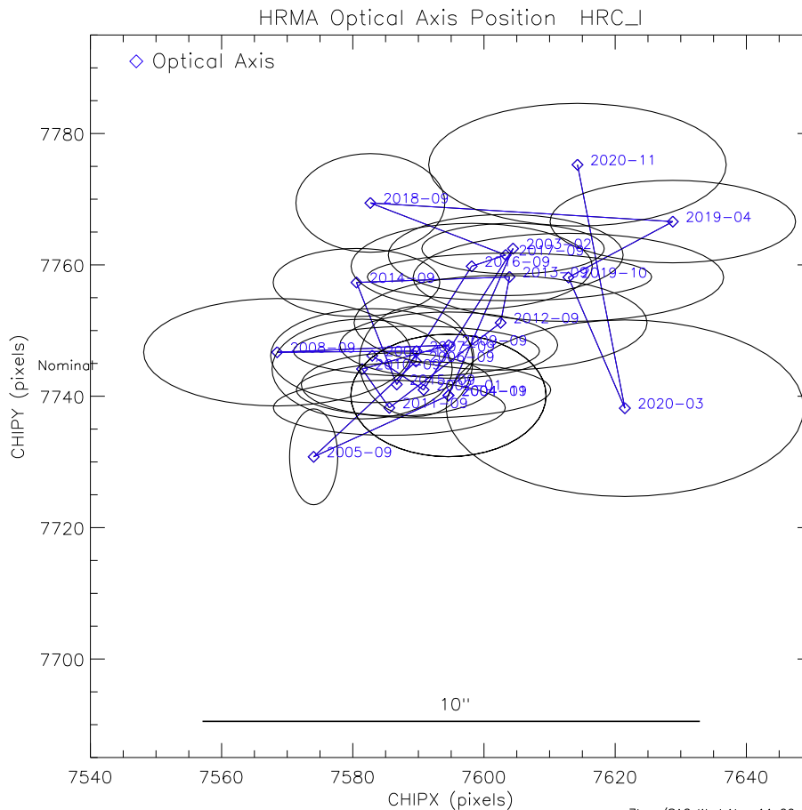
Figure 4.25: Chandra optical axis positions on HRC-I since launch. Each position is labeled by the year-month. The ellipse around each position is the 1\text{-}\sigma measurement error ellipse for that given year. The drift of optical axis position is consistent with the measurement errors. The optical axis position is very stable and well within a 10 arcsec region.
