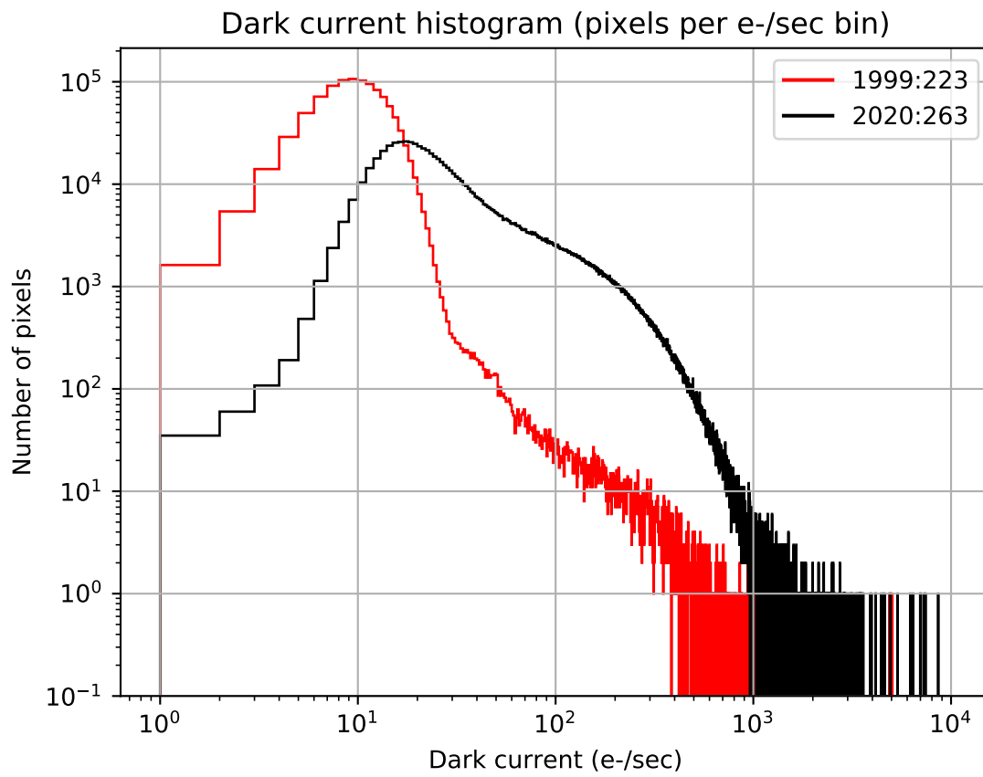
Figure 5.8: Differential histogram of dark current distribution for the ACA CCD in 1999-Aug and 2020-Sep
