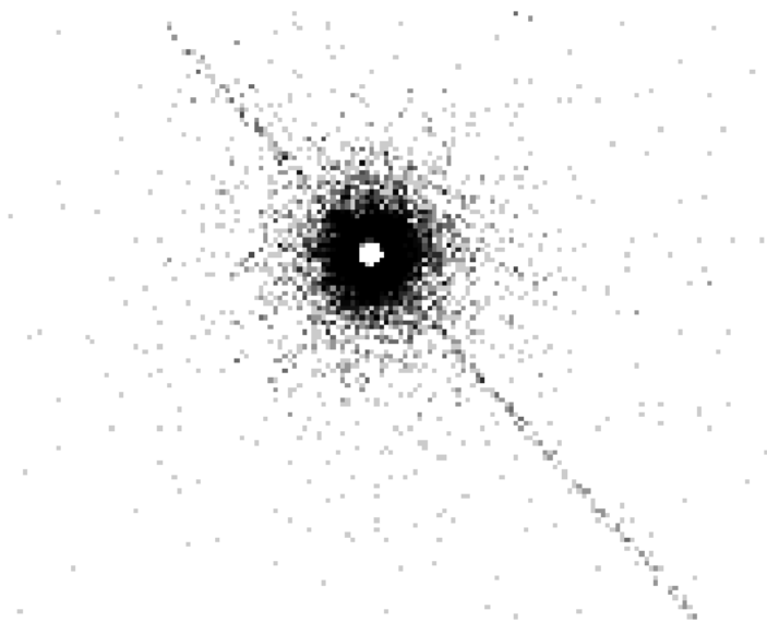
Figure 6.17: Trailed image of a strong X-ray source. The core of the image is faint due to pile-up. Most events here are rejected because of bad grades. The read-out direction is parallel to the trail.
