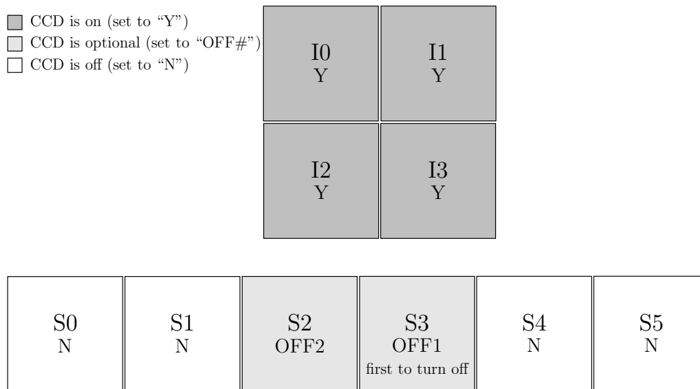
Figure 6.37: ACIS-I imaging, nominal aimpoint (4 Required CCDs, 2 Optional CCDs)
