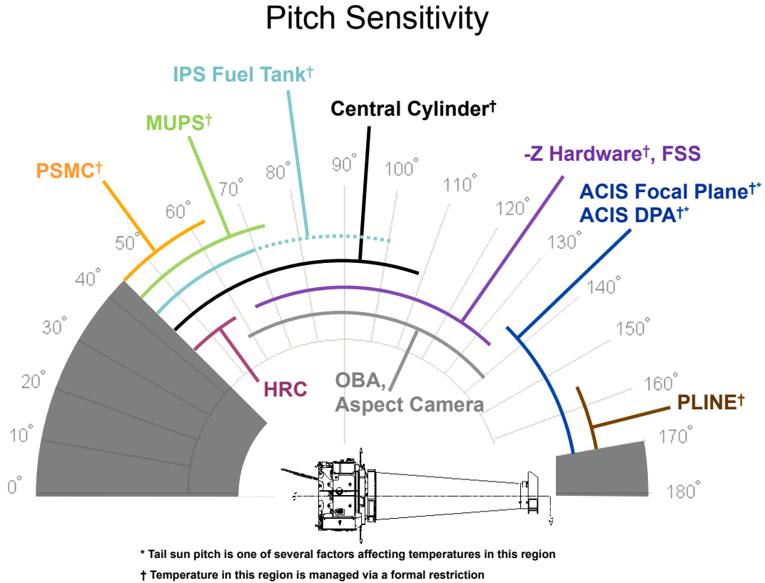
Figure 6.31: Pitch sensitivity of spacecraft components [See the online Proposers' Observatory Guide for a color version of this figure]
