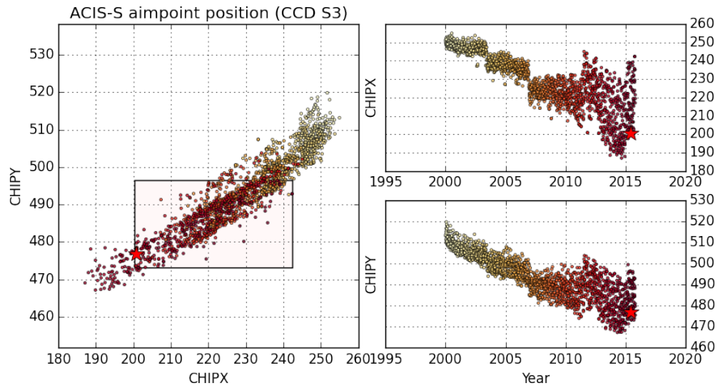
Figure 5.5: Representative sampling of the post-facto observation aimpoint (CHIPX, CHIPY) over the mission, where one ACIS pixel (CHIPX, CHIPY) equals 0.492 arc-sec. This sampling includes extrema within monthly bins. The red star corresponds to the published aimpoint for Cycle 17, while the light magenta rectangle shows the bounding box of aimpoints within the 6-month interval ending on 2015-Nov-1. Note that the rectangle in this figure shows the region over which the aimpoint moved during a specific 6-month period in 2015 and differs from the boxes the users are advised to consider for placement of their target on the detectors.
