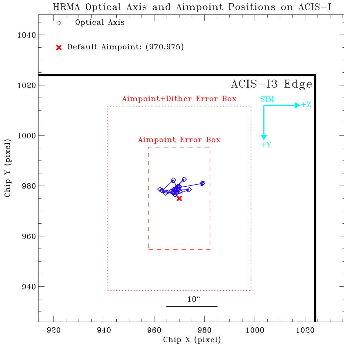
Figure 4.26: Chandra optical axis (blue diamonds) positions for each year and permanent default aimpoint (red cross) on ACIS-I. The small box (red dashed line, 12'' \times 20'' , or 24.4 \times 40.7 pixels) centered at the aimpoint is the error box of the aimpoint center, i.e. an on-axis target can be anywhere inside this box. The large box (red dotted line, 28'' \times 36'' , or 56.9 \times 73.2 pixels) is the error box of aimpoint with dither.
