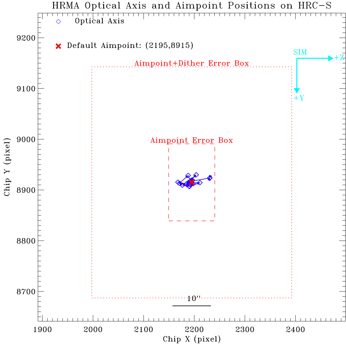
Figure 4.29: Chandra optical axis (blue diamonds) positions for each year and permanent default aimpoint (red cross) on HRC-S. The small box (red dashed line, 12'' \times 20'' , or 91.1 \times 151.8 pixels) centered at the aimpoint is the error box of the aimpoint center, i.e. an on-axis target can be anywhere inside this box. The large box (red dotted line, 52'' \times 60'' , or 394.7 \times 455.4 pixels) is the error box of aimpoint with dither.
