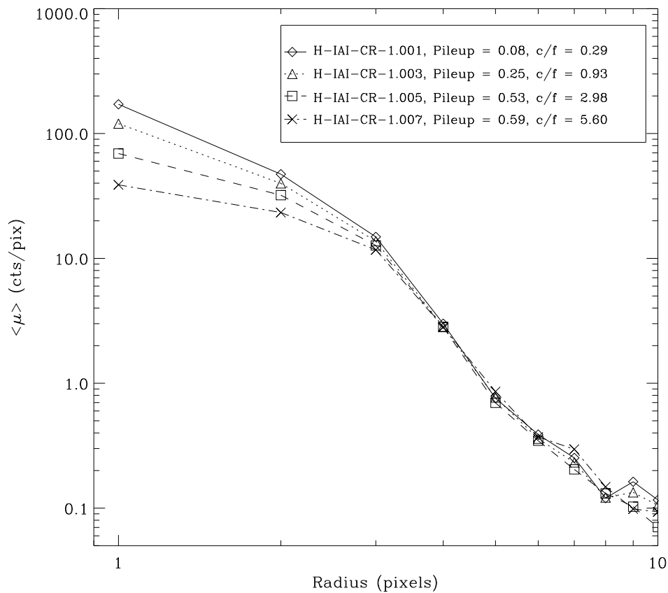
Figure 6.20: The effects of pile-up on the radial distribution of the PSF are illustrated. These data were taken during ground calibration at the XRCF. The specific “OBSIDs”, the counting rate per CCD frame (“c/f”), and the “pile-up fraction” as defined in Section 6.15.2 are given in the inset.
