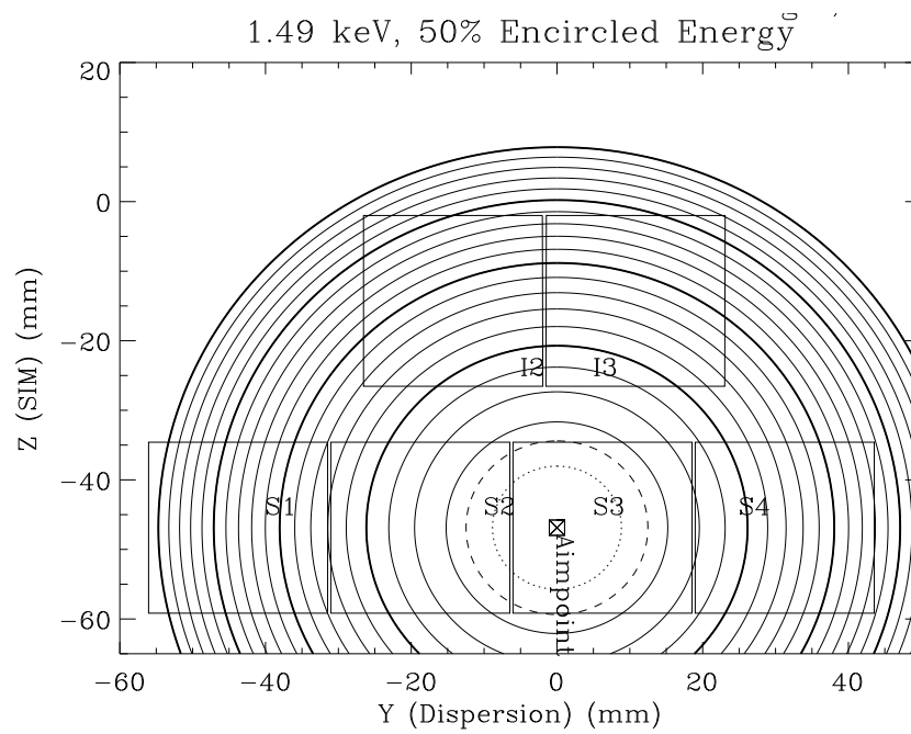
Figure 6.15: Approximate contours of constant 50% encircled energy at 1.49 keV when the ACIS-S aimpoint is selected. The dotted line is 1 arcsec, the dashed line is 1.5 arcsec. The remainder are at 1 arcsec intervals. The thicker solid lines highlight the 5, 10, 15 and 20 arcsec contours.
