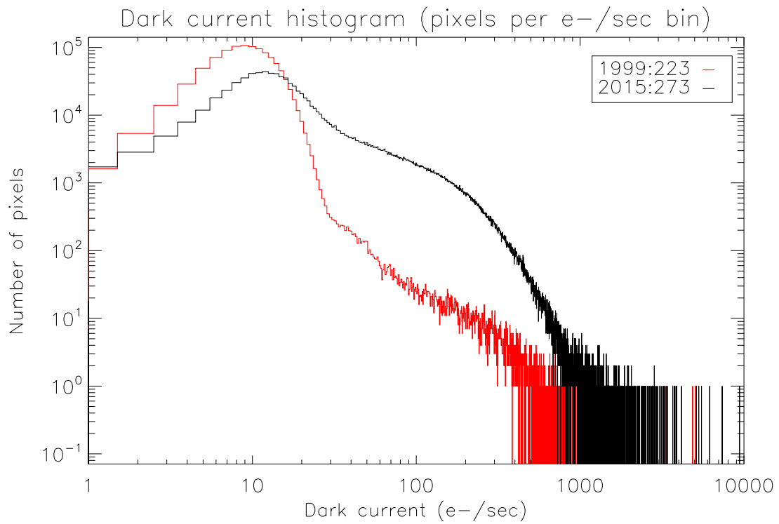
Figure 5.8: Differential histogram of dark current distribution for the ACA CCD in 1999-Aug and 2015-Sep
