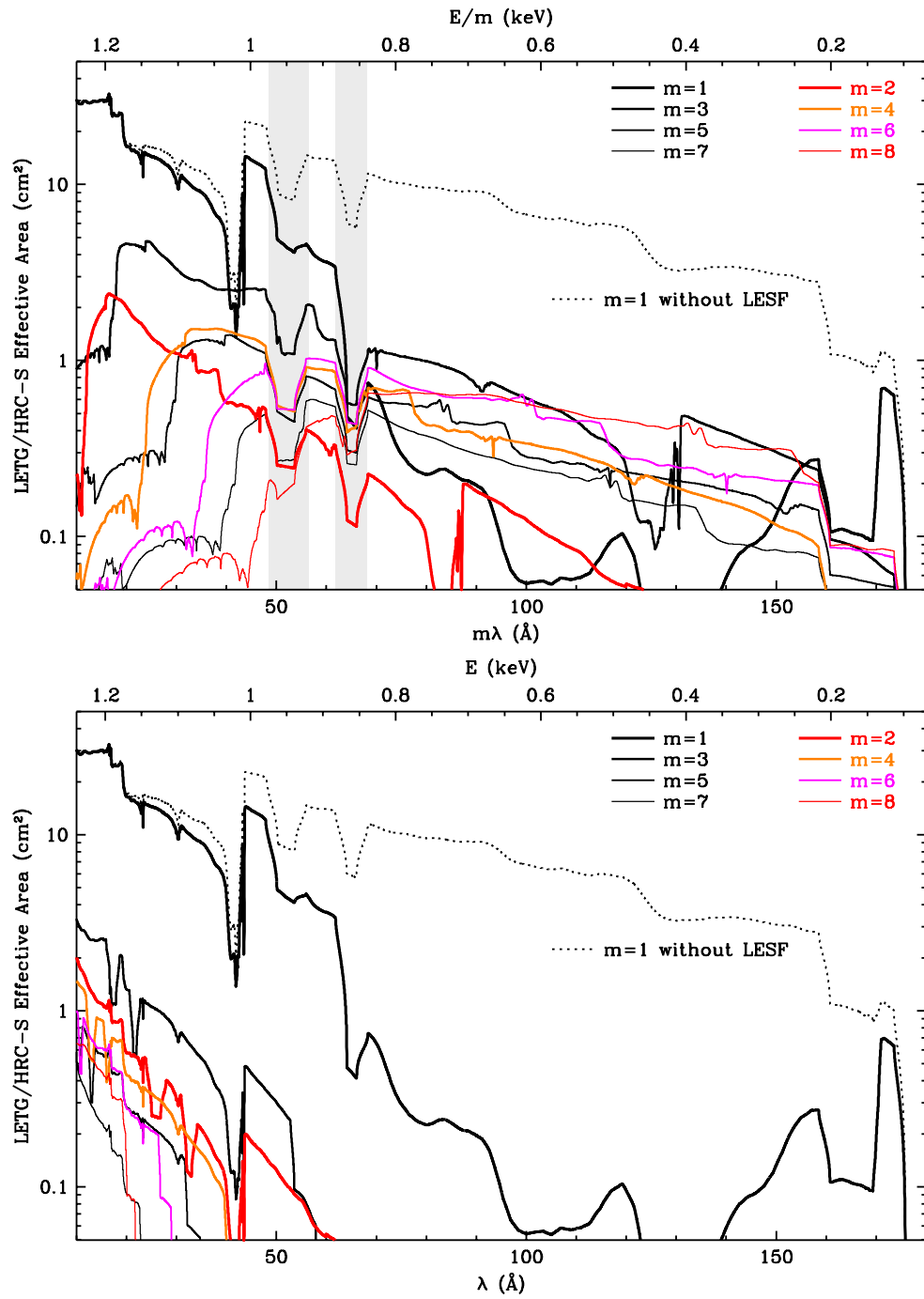
Figure 9.19: The combined HRMA/LETG/HRC-S/LESF effective areas for 1st and higher orders. Positive and negative orders are summed. Note that the wavelength axis begins at 10 Å.
