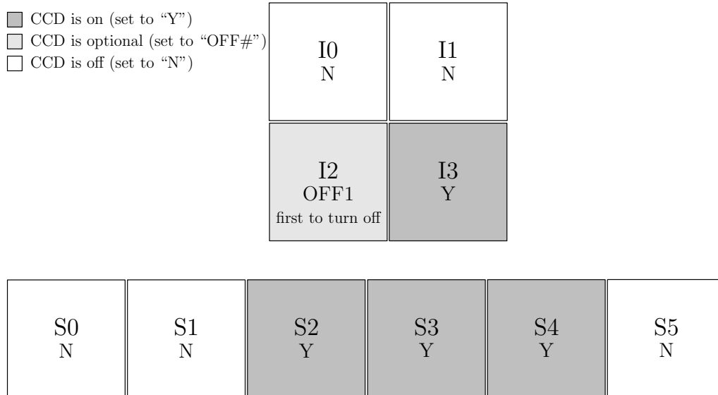
Figure 6.38: ACIS-S imaging, nominal aimpoint (4 Required CCDs, 1 Optional CCD)
