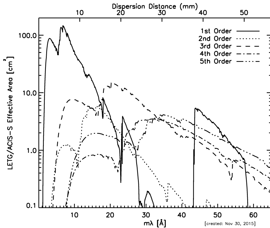
Figure 9.20: The combined HRMA/LETG/ACIS-S effective areas for 1st and higher orders. LETG+ACIS-S areas include the effects of time-dependent contamination. Positive and negative orders are summed.
