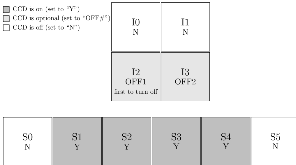
Figure 6.40: ACIS-S imaging, nominal aimpoint (4 Required CCDs, 2 Optional CCDs)
