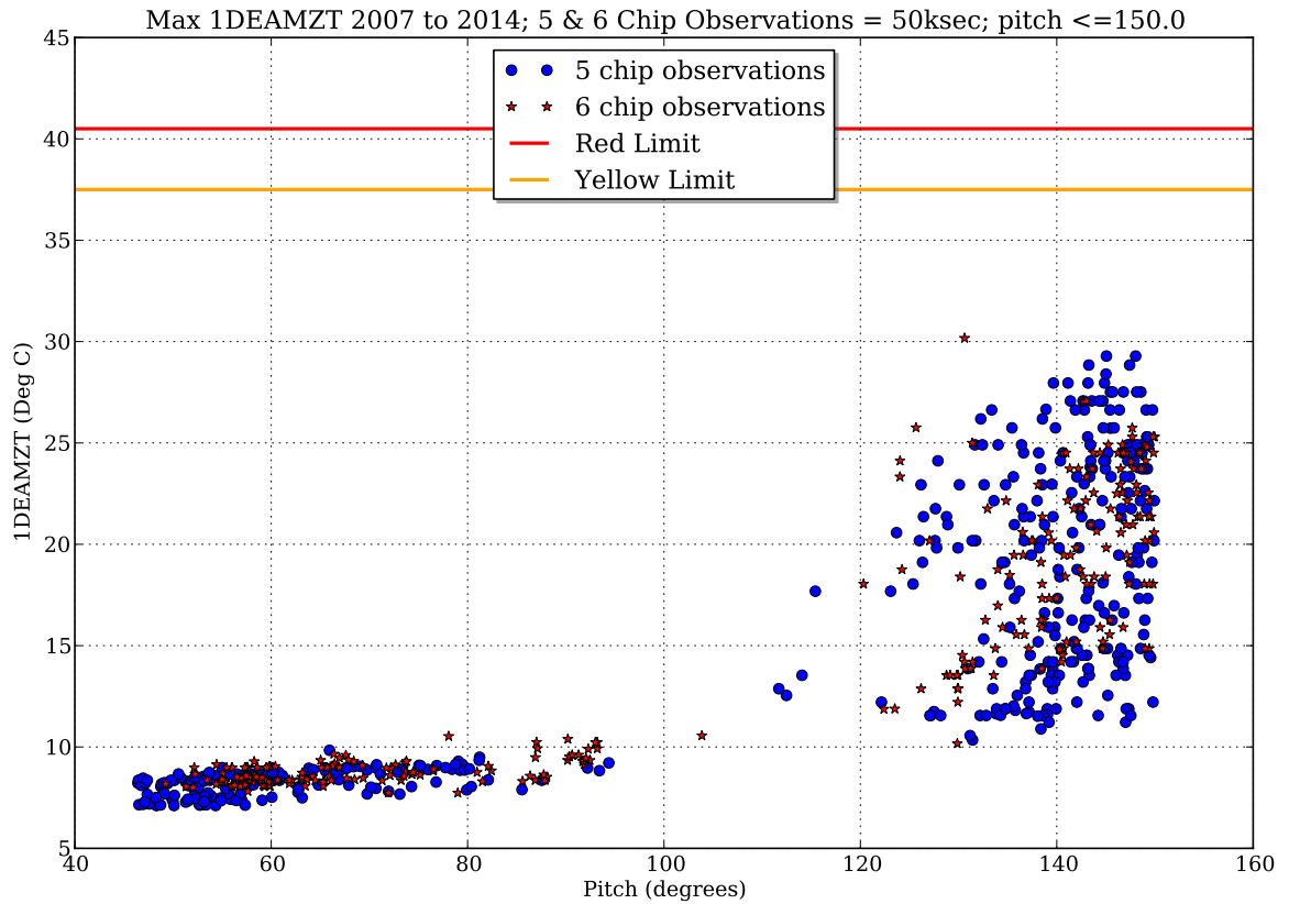
Figure 6.34: DEA temperature versus pitch angle for 5 and 6 CCD observations. This figure shows the variation of DEA temperature with pitch angle. 6-CCD observations are indicated by small (red) stars, and 5-CCD observations are indicated by larger (blue) circles. [See the online Proposers' Observatory Guide for a color version of this figure]
