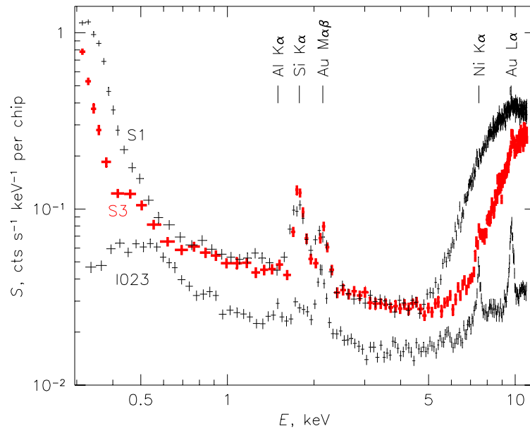
Figure 6.24: Energy spectra of the charged particle ACIS background with ACIS in the stowed position (a 50 ks exposure taken in 2002-Sep; standard grade filtering, no VF filtering). Line features are due to particle-induced fluorescence of material in and surrounding the focal plane.
