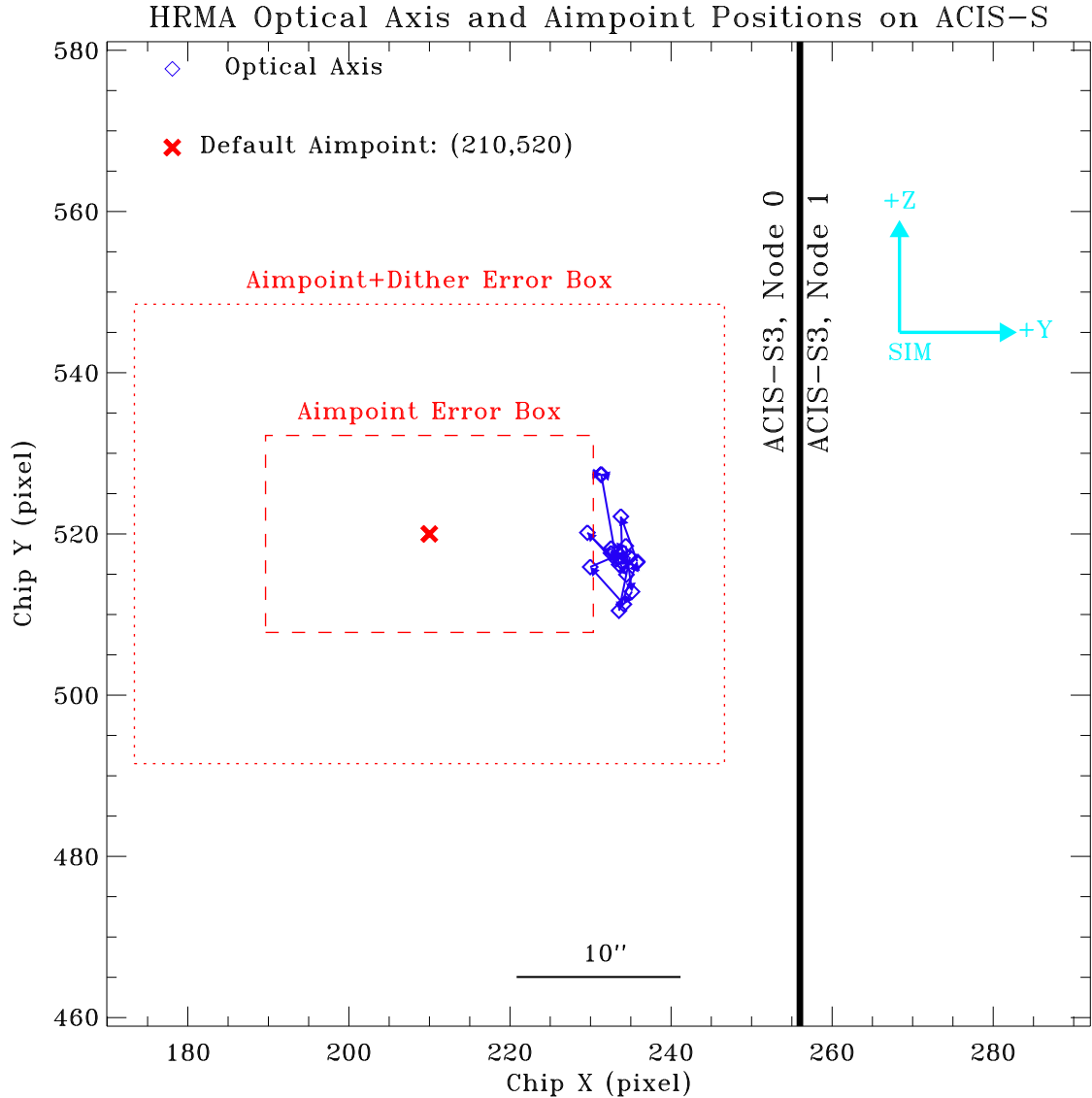
Figure 4.27: Chandra optical axis (blue diamonds) positions for each year and permanent default aimpoint (red cross) on ACIS-S. The small box (red dashed line, 20'' \times 12'' , or 40.7 \times 24.4 pixels) centered at the aimpoint is the error box of the aimpoint center, i.e. an on-axis target can be anywhere inside this box. The large box (red dotted line, 36'' \times 28'' , or 73.2 \times 56.9 pixels) is the error box of aimpoint with dither. Note the permanent default aimpoint is \sim 12'' from the optical axis in order to avoid the node boundary 0|1.
