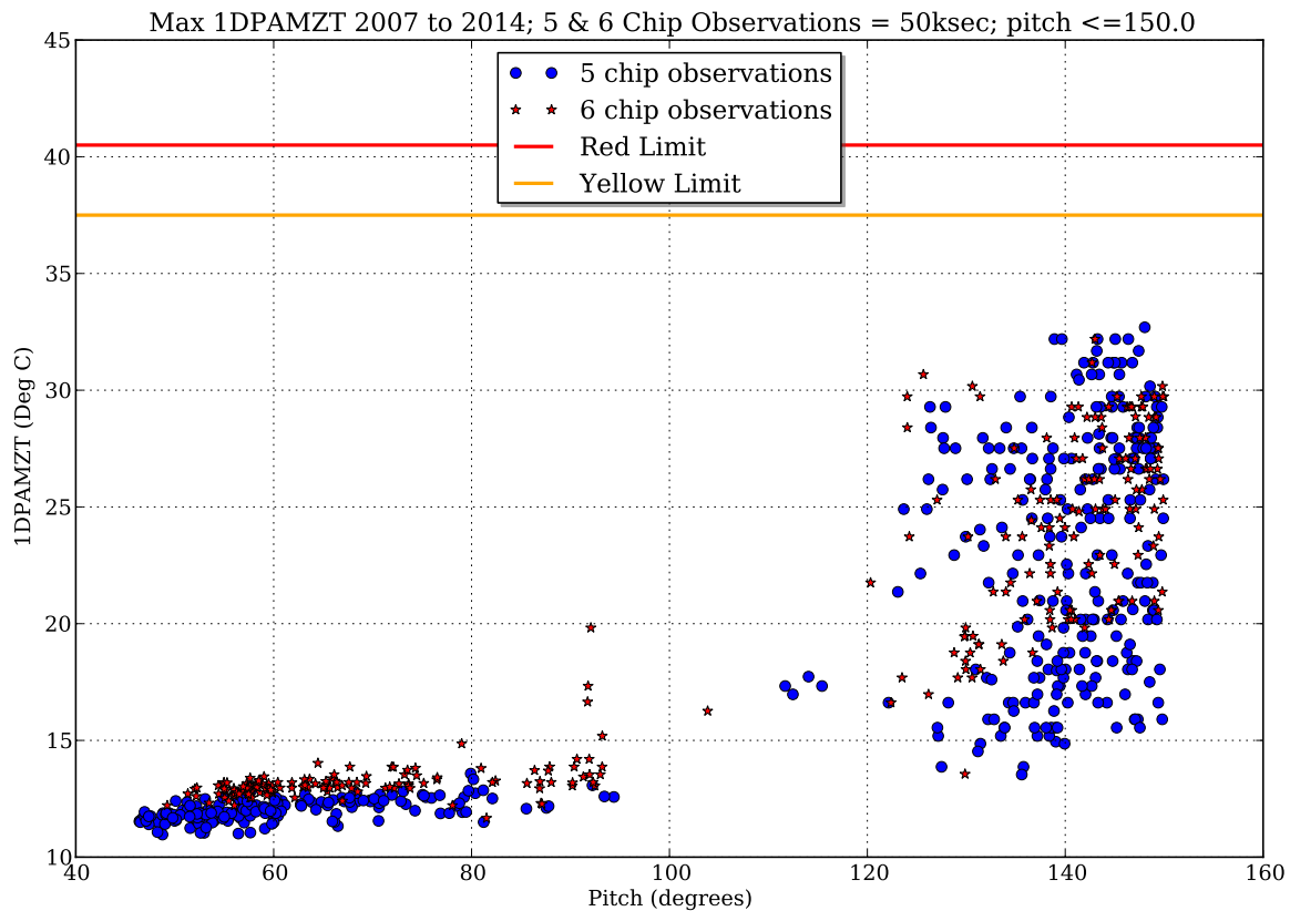
Figure 6.33: DPA temperature as a function of pitch angle for 5 and 6 CCD configurations. This figure shows the variation of DPA temperature with pitch angle. 6-CCD observations are indicated by small (red) stars, and 5-CCD observations are indicated by larger (blue) circles. [See the online Proposers' Observatory Guide for a color version of this figure]
