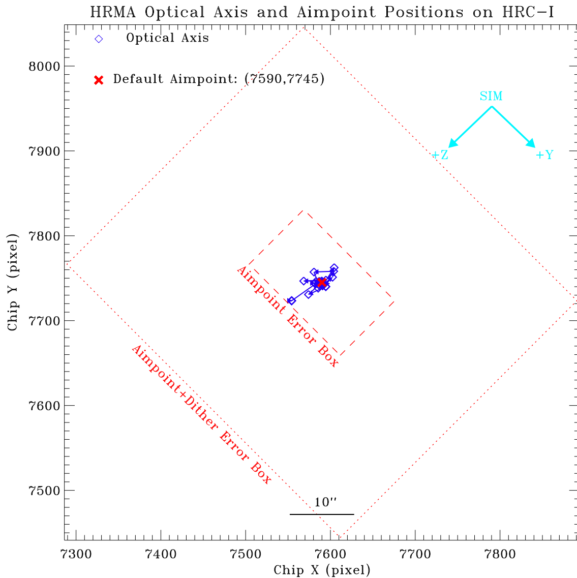
Figure 4.28: Chandra optical axis (blue diamonds) positions for each year and permanent default aimpoint (red cross) on HRC-I. The small box (red dashed line, 20'' \times 12'' , or 151.8 \times 91.1 pixels in SIM [Y, Z]) centered at the aimpoint is the error box of the aimpoint center, i.e. an on-axis target can be anywhere inside this box. The large box (red dotted line, 60'' \times 52'' , or 455.4 \times 394.7 pixels in SIM [Y, Z]) is the error box of aimpoint with dither.
