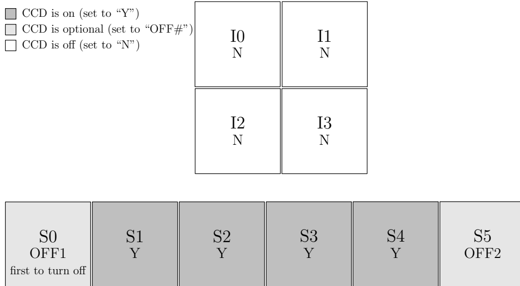
Figure 6.41: ACIS-S spectroscopy, nominal aimpoint (4 Required CCDs, 2 Optional CCDs)
