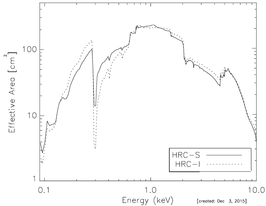
Figure 7.17: The effective area of the HRMA/HRC-I (dashed line) and the central segment of the HRMA/HRC-S in imaging mode (solid line) integrated over the full PSF. Absorption edges are due to the iridium coating on the mirrors, the CsI MCP coating, and the polyimide/Al of the UVIS.
