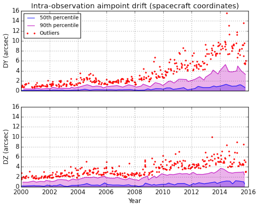
Figure 5.6: Peak to peak aimpoint drift within individual science observations.
