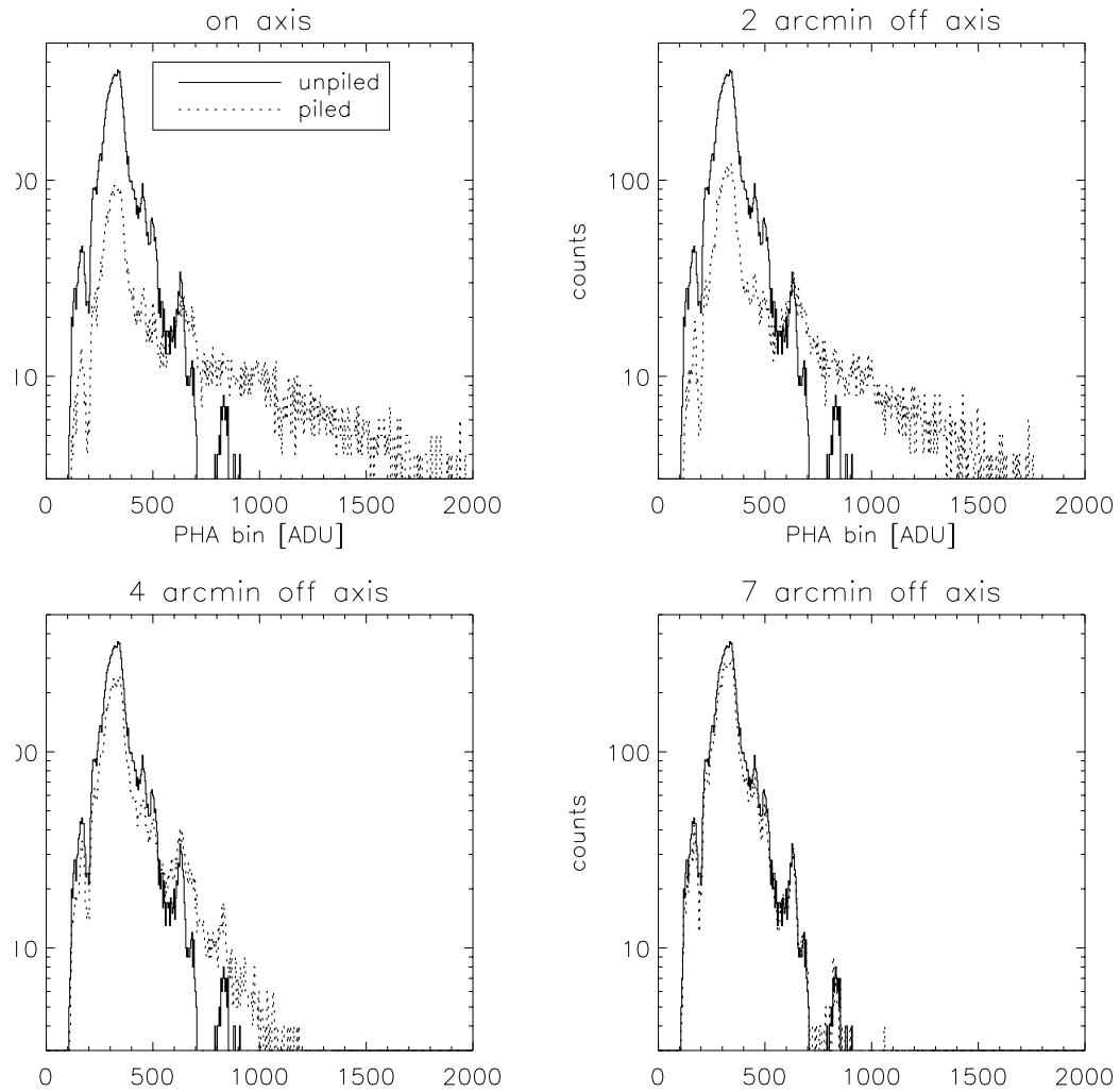
Figure 6.22: MARX simulations of the effect of pile-up on the shape of the spectrum. The true (solid line) and the detected (dotted line) spectra are shown for four different viewing angles. The corresponding “pile-up fractions” – see Section 6.15.2 – are 46%, 40%, 15%, and 2% as the image is moved progressively further off-axis.
