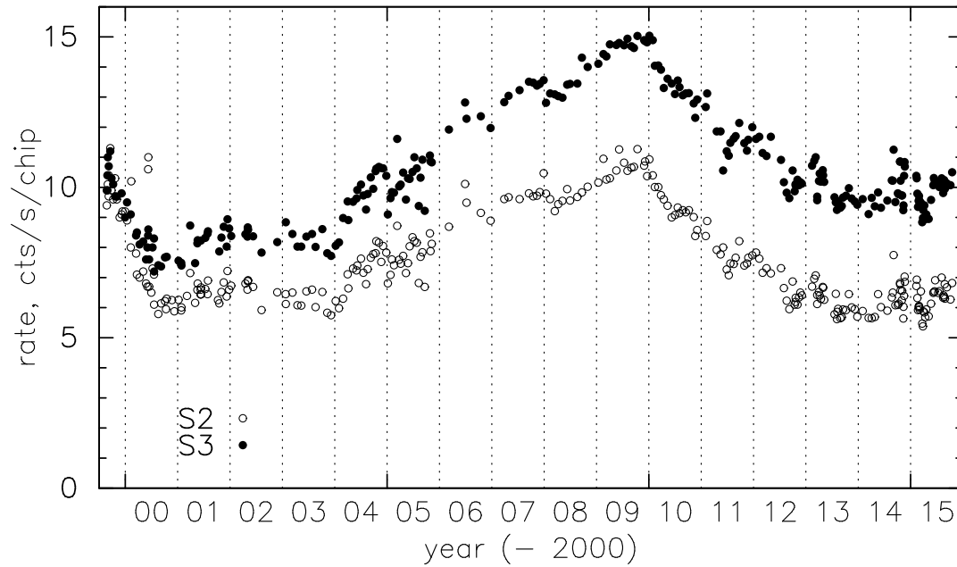
Figure 6.27: Total telemetered background rates (including all grades and the upper event cutoff at 15 keV) for chips S2 (FI) and S3 (BI) as a function of time. Vertical dashed lines are year boundaries.
