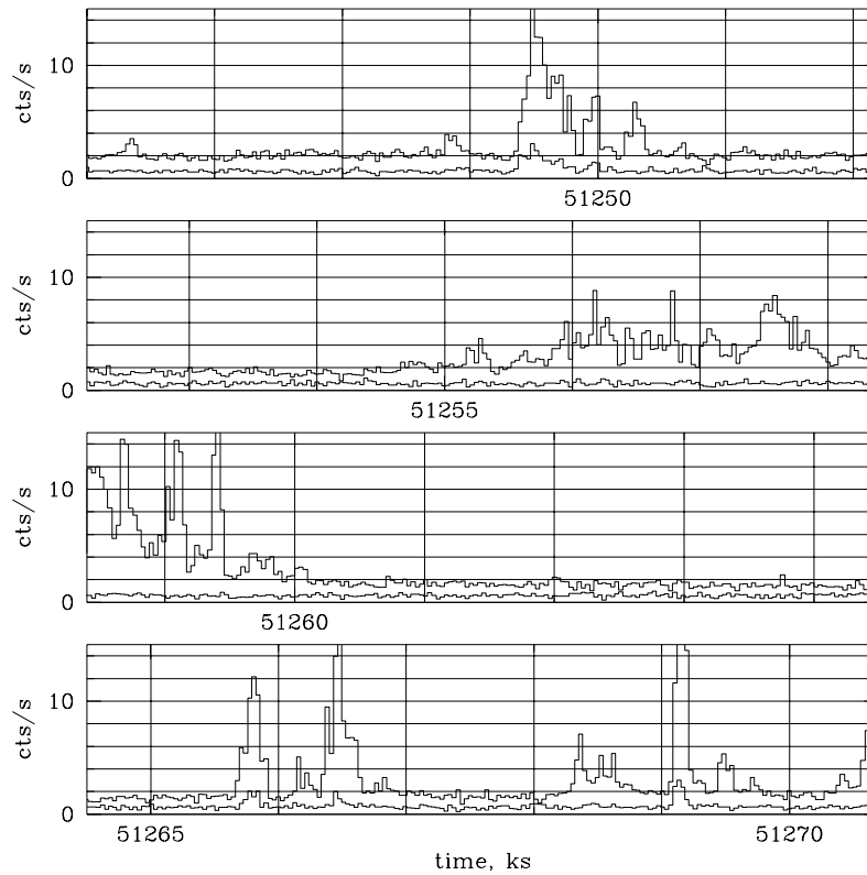
Figure 6.28: An example of the ACIS background counting rate versus time – BI chip (S3; top curve) and an FI chip (I2; bottom curve). These are for the standard grades and the band from 0.3 - 10 keV.
