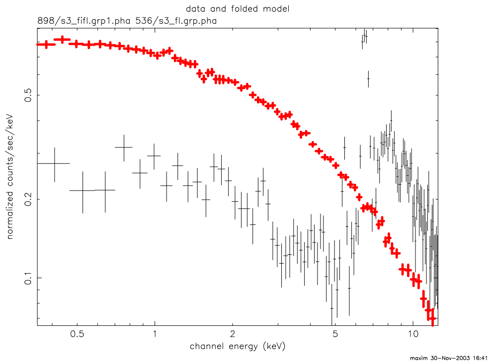
Figure 6.30: Spectra of different background flares in chip S3. Thick crosses show a common flare species that affects only the BI chips. Thin crosses show one of the several less common flare species that affect both the BI and FI chips. Note how both these spectra are different from the quiescent spectrum (see Figure 6.26).
