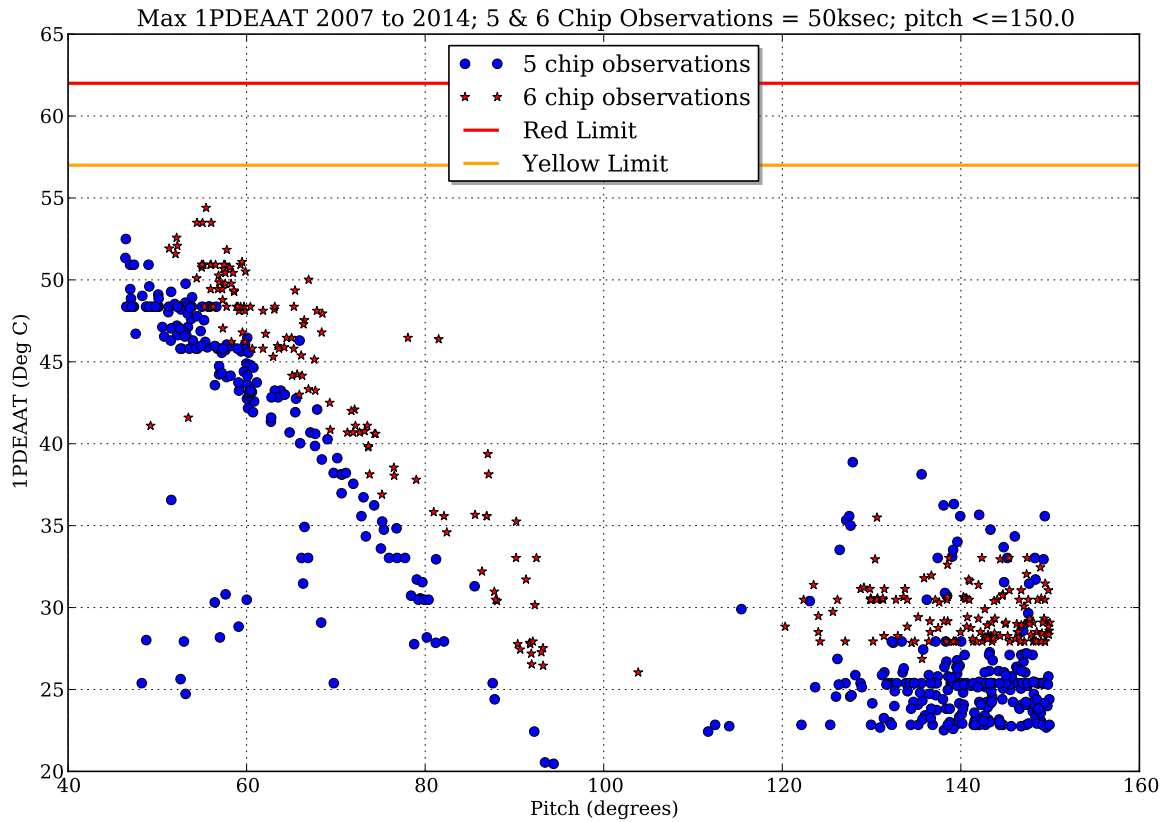
Figure 6.32: ACIS PSMC temperature as a function of spacecraft pitch angle 6-CCD observations are indicated by small (red) stars, and 5-CCD observations are indicated by larger (blue) circles. [See the online Proposers' Observatory Guide for a color version of this figure]
