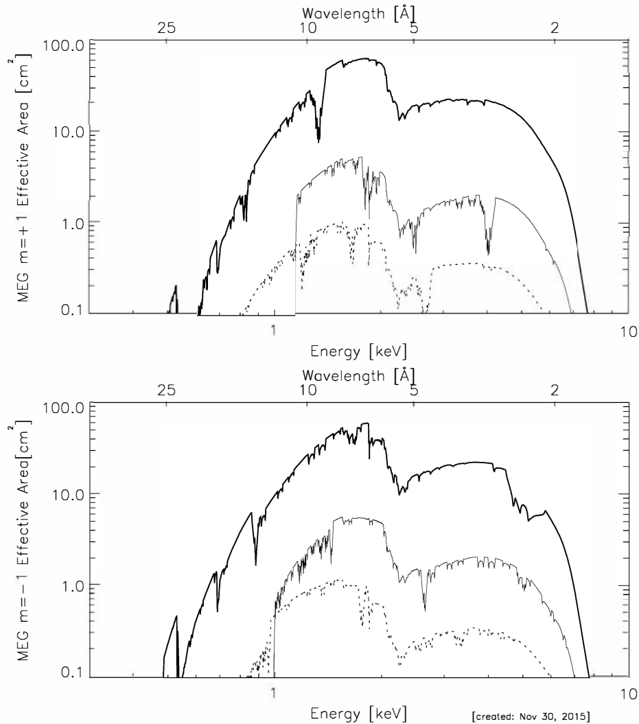
Figure 8.9: The HETGS MEG effective area, integrated over the PSF is shown with energy and wavelength scales. The m = +1, +2, +3 orders (falling on ACIS chips S5, S4, S3; left to right) are displayed in the top panel and the m = -1, -2, -3 orders (falling on ACIS chips S0, S1, S2; left to right) are in the bottom panel. The thick solid lines are first order; the thin solid line is third order; and the dotted line is second order.
