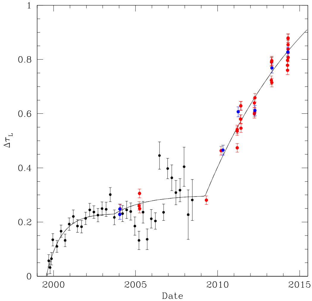
Figure 6.8: Difference in the optical depth between near the center of the chip and the edge of the chip near the readout versus time. ACIS-I3 data are shown as light gray (red) circles, and ACIS-S3 data as dark gray (blue) circles. The black circles are ECS data. (See the online Proposers' Observatory Guide for a color version of this figure.)
