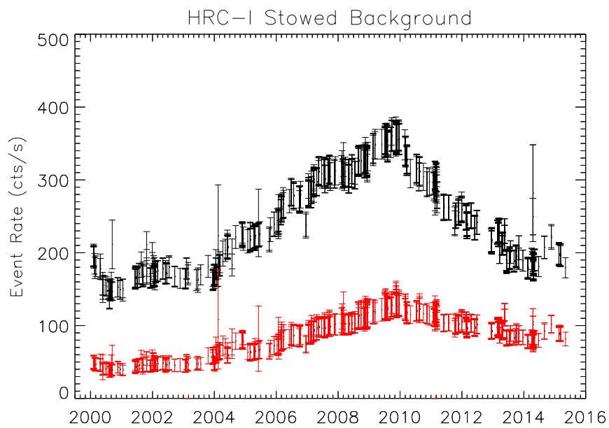
Figure 7.20: The change in HRC-I stowed background rate with time. The total rate (black points and error bars, upper set) and the valid rate (red points and error bars, lower set) are shown. The HRC-S data are similar.
