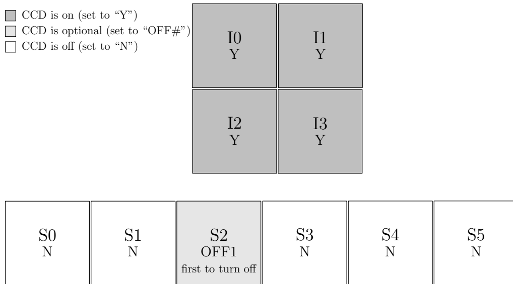
Figure 6.35: ACIS-I imaging, nominal aimpoint (4 Required CCDs, 1 Optional CCD)
