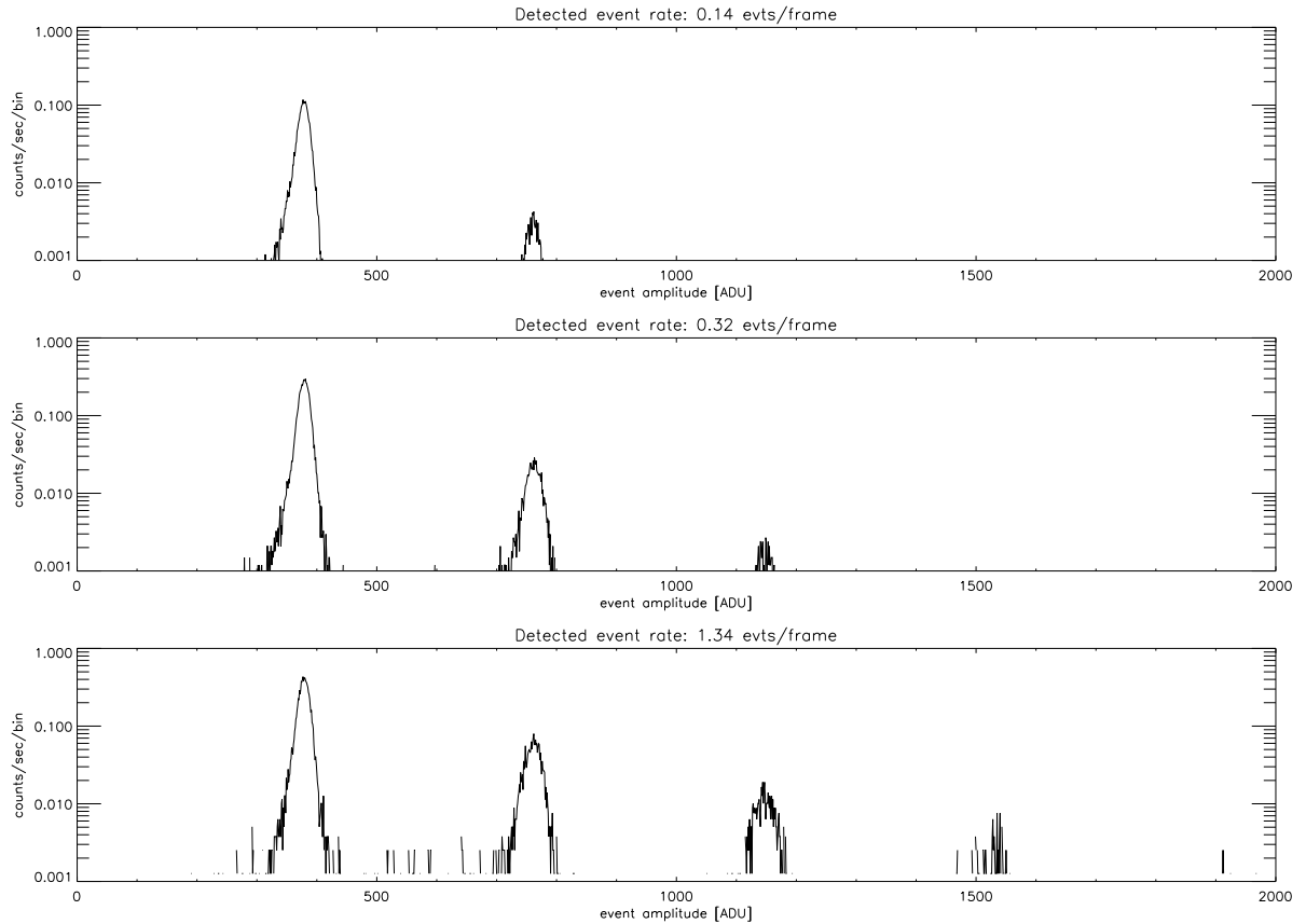
Figure 6.19: The effects of pile-up at 1.49 keV ( \text{Al K}\alpha ) as a function of source intensity. Data were taken during HRMA-ACIS system level calibration at the XRCF. Single-photon events are concentrated near the pulse height corresponding to the \text{Al K}\alpha line ( \sim 380 ADU), and events with 2 or more photons appear at integral multiples of the line energy.
