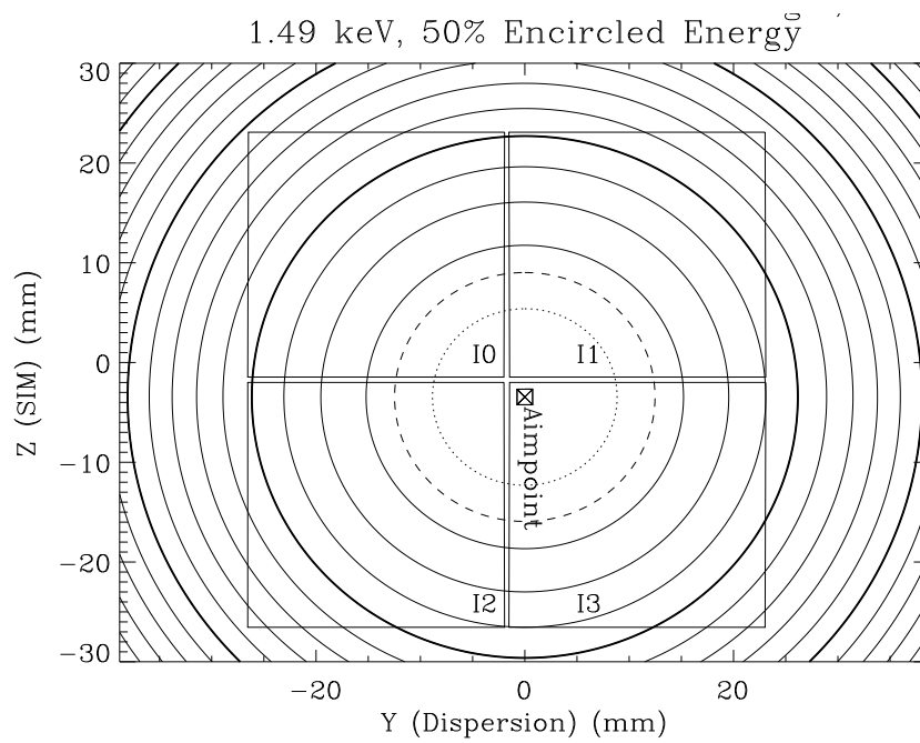
Figure 6.14: Approximate contours of constant 50% encircled energy at 1.49 keV when the ACIS-I aimpoint is selected. The dotted line is 1 arcsec, the dashed line is 1.5 arcsec. The remainder are at 1 arcsec intervals. The thicker solid lines highlight the 5, 10, and 15 arcsec contours.
