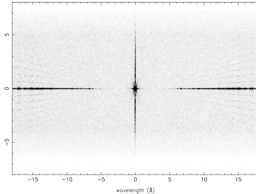
Figure 9.23: HRC-S detector image of LETGS observation of Capella. In order to illustrate the stretching of the cross-dispersion axis, both axes are in \text{\AA} with 1.148 \text{ \AA/mm} ; only the central 30 mm of the central plate is shown. The full extent of the telemetered six-tap cross-dispersion window is shown and measures 9.9 mm. The areas of reduced background at top and bottom are due to dither effects. Star-shaped coarse support structure diffraction is seen around zeroth order, and “cat’s whiskers” fine support structure diffraction is seen above and below the primary dispersion axis, as well as in the vertical line through zeroth order.
