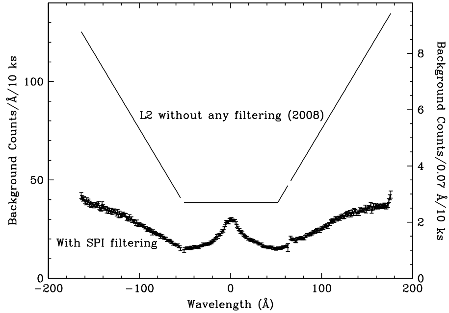
Figure 9.22: The Jan 2008 LETGS+HRC-S background rate with and without pulse-height filtering. These Level 2 rates correspond to 1.1 \times 10^{-6} cts s^{-1} pixel ^{-1} (see Figure 9.21). Data are shown using the standard ‘bowtie’ spectral extraction region (see Figure 9.14). X-ray losses from the observed spectrum as a result of the filtering for 1st order are \sim 1.25\% ; losses will be slightly higher for higher orders. See http://cxc.harvard.edu/cal/Letg/Hrc_bg for more information.
