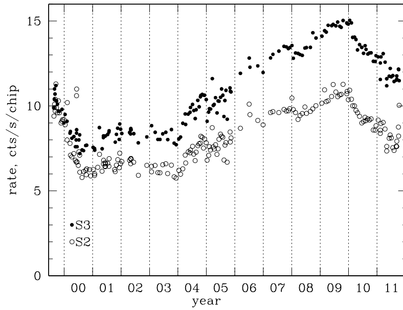
Figure 6.24: Total telemetered background rates (including all grades and the upper event cutoff at 15 keV) for chips S2 (FI) and S3 (BI) as a function of time. Vertical dashed lines are year boundaries.
