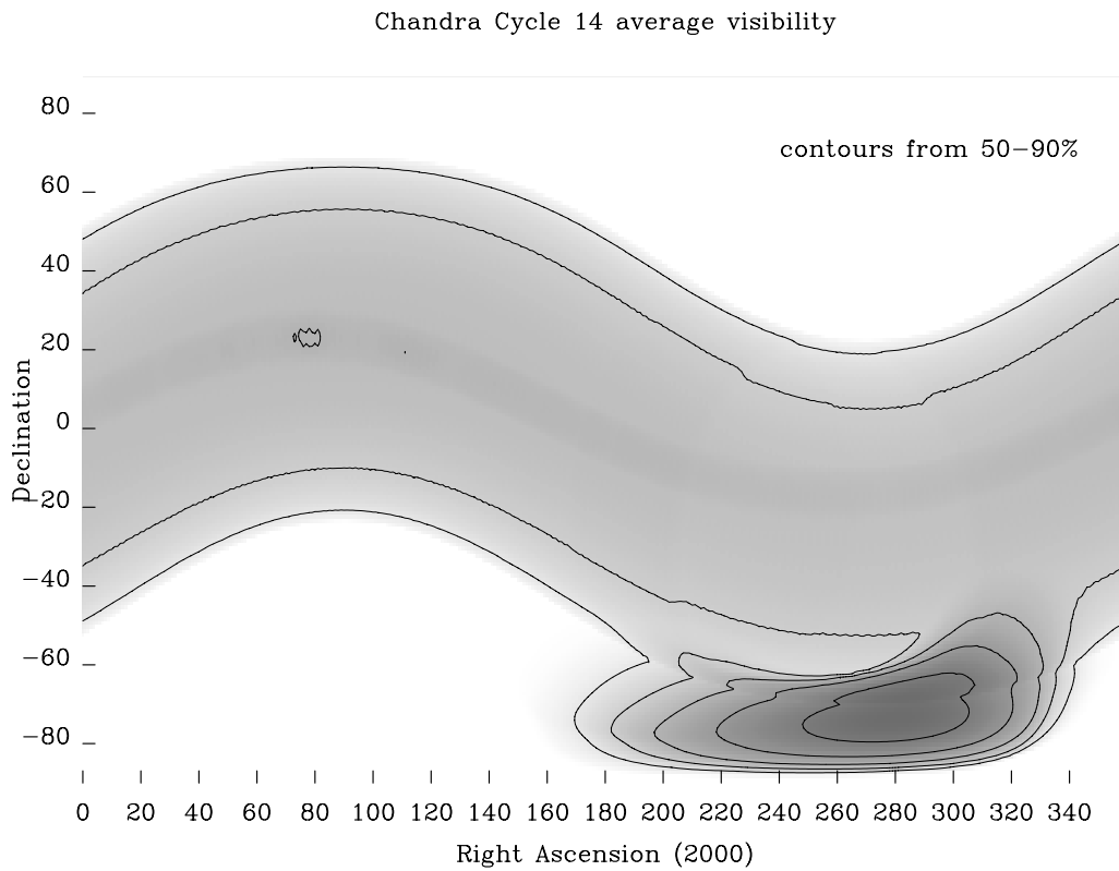
Figure 3.3: The Chandra visibility showing contours of fractional visibility averaged over the 12-month interval of Cycle 14. The darker the shade of gray, the lower the visibility. The five contour levels correspond to 50%, 60%, 70%, 80%, and 90% average visibility.
