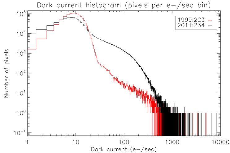
Figure 5.6: Differential histogram of dark current distribution for the ACA CCD in 1999-Aug and 2011-Aug
