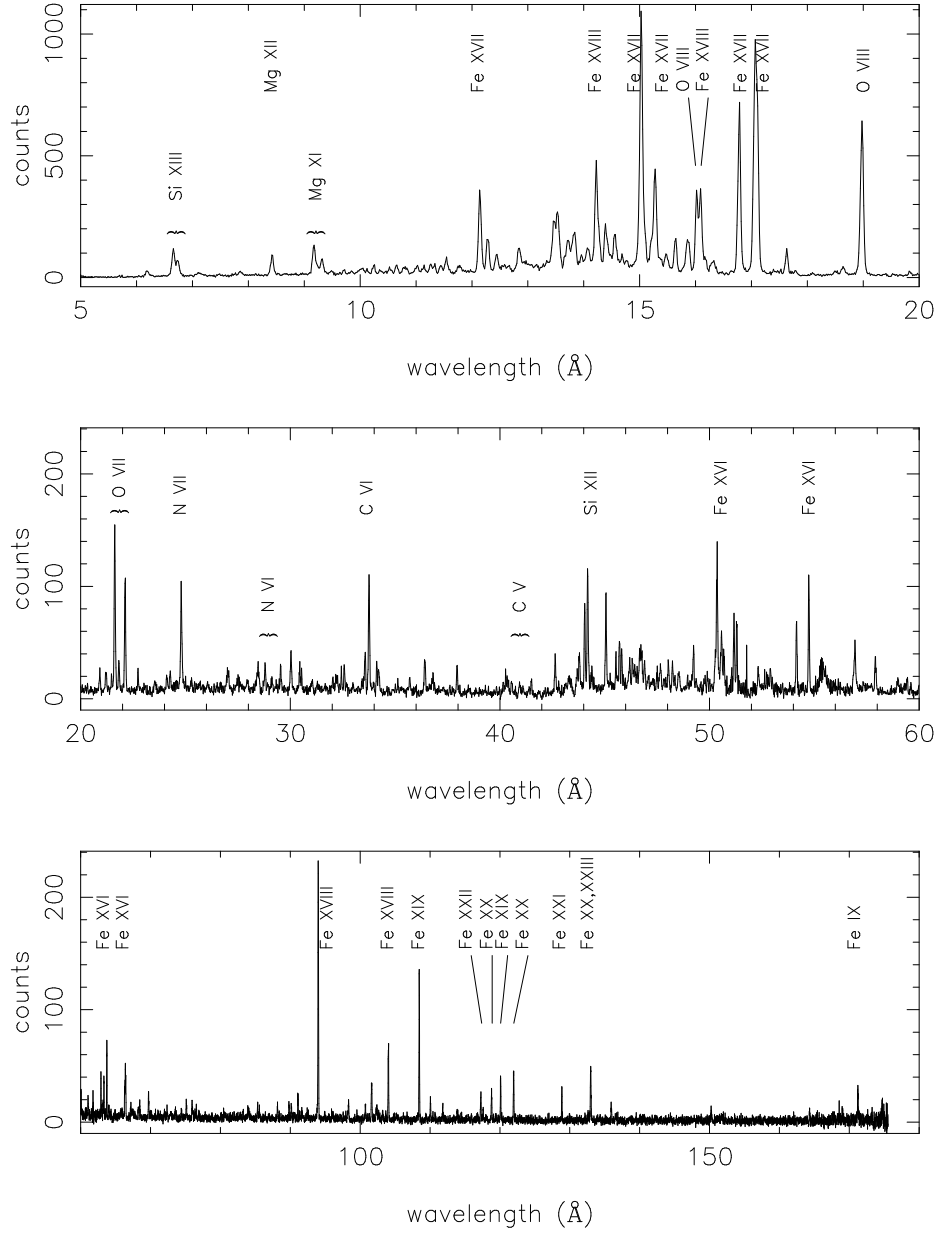
Figure 9.26: Extracted LETGS spectrum of Capella with some line identifications (from Brinkman et al. 2000, ApJ, 530, L111). Many of the lines visible between 40 and 60 Å are 3rd order dispersion of the strong features seen in 1st order in uppermost panel.
