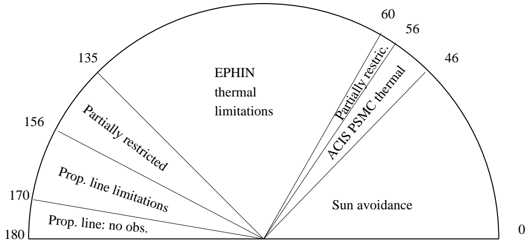
Figure 3.4: Diagram to illustrate ranges of solar pitch angle (the angle between the pointing direction and the satellite-Sun line) within which different major observing limitations apply. Table 3.1 provides quantitative estimates for the observing limitations in the solar pitch angle ranges shown in the drawing.
