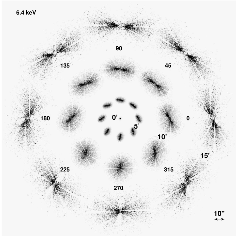
Figure 4.15: Simulated 6.4 keV images, for the HRMA only. Images are shown with a linear stretch, as they would appear on the sky, at three off-axis angles ( 5' , 10' , and 15' and various azimuths. The images are all to the same scale, illustrated by the scale bar. The spacing between images is arbitrary. The surface brightness of the images at 10' and 15' has been enhanced to show structure. Spokes in the images are due to shadowing by mirror support struts. Cusps in are due to a slight misalignment of the parabolic and hyperbolic mirrors. These simulations are at an effective roll of zero – observations should be “de-rolled” before comparison to these images.
