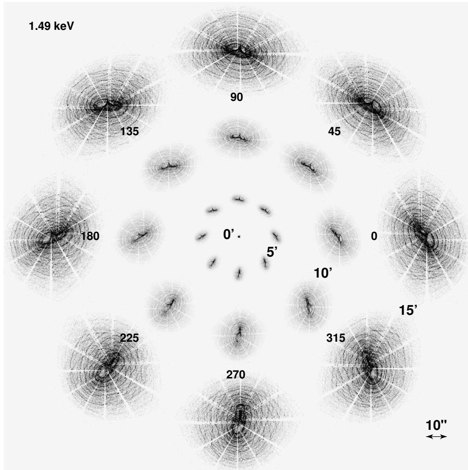
Figure 4.14: Simulated 1.49 keV images, for the HRMA only. Images are shown with a linear stretch, as they would appear on the sky, at three off-axis angles (5', 10', and 15' and various azimuths. The images are all to the same scale, illustrated by the scale bar. The spacing between images is arbitrary. The surface brightness of the images at 10' and 15' has been enhanced to show structure. Spokes in the images are due to shadowing by mirror support struts. Cusps are due to a slight misalignment of the parabolic and hyperbolic mirrors. These simulations are at an effective roll of zero – observations should be "de-rolled" before comparison to these images.
