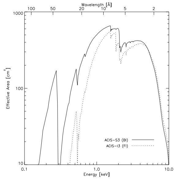
Figure 6.4: The HRMA/ACIS predicted effective area versus the energy on a log scale. The dashed line is for the FI CCD I3, and the solid line is for the BI CCD S3.
