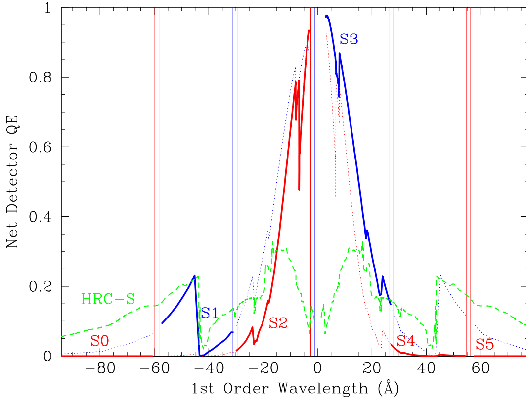
Figure 9.6: Comparison of detector quantum efficiencies for the ACIS FI and BI chips, and for the HRC-S, when used with the LETG. The thick dashed (green) line is for HRC-S, while the thick solid curves are for ACIS. The thin dotted curves indicate FI quantum efficiencies at dispersions where first order photons fall on BI chips, and vice-versa. Quantum efficiencies shown for ACIS are for the default Y-offset = +1.5' ; the HRC-S curves correspond to Y-offset = 0. Y-offsets may be chosen to tailor the coverage of BI chips (S1 and S3; blue QE curve), which have higher QE at low energies than the FI chips (S0, S2, S4, S5; bottom/red curve). Vertical lines indicate ACIS chip gaps (with dither, 1.5 \text{ \AA} ). For clarity, -3 to +3 \text{ \AA} is not shown for ACIS. See Section 9.4.2/Offset Pointing for more information regarding the choice of Y-offset.
