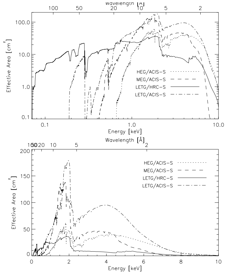
Figure 1.4: Comparison of the first-order effective areas in square centimeters (integrated over the line spread function) of the MEG, HEG and LETG spectrometers. Top panel is log and bottom panel is linear scale. The (+/-) first orders of the diffracted spectrum have been added. The curves using ACIS show the predicted values for the middle of Cycle 11 (2010-05-15)
