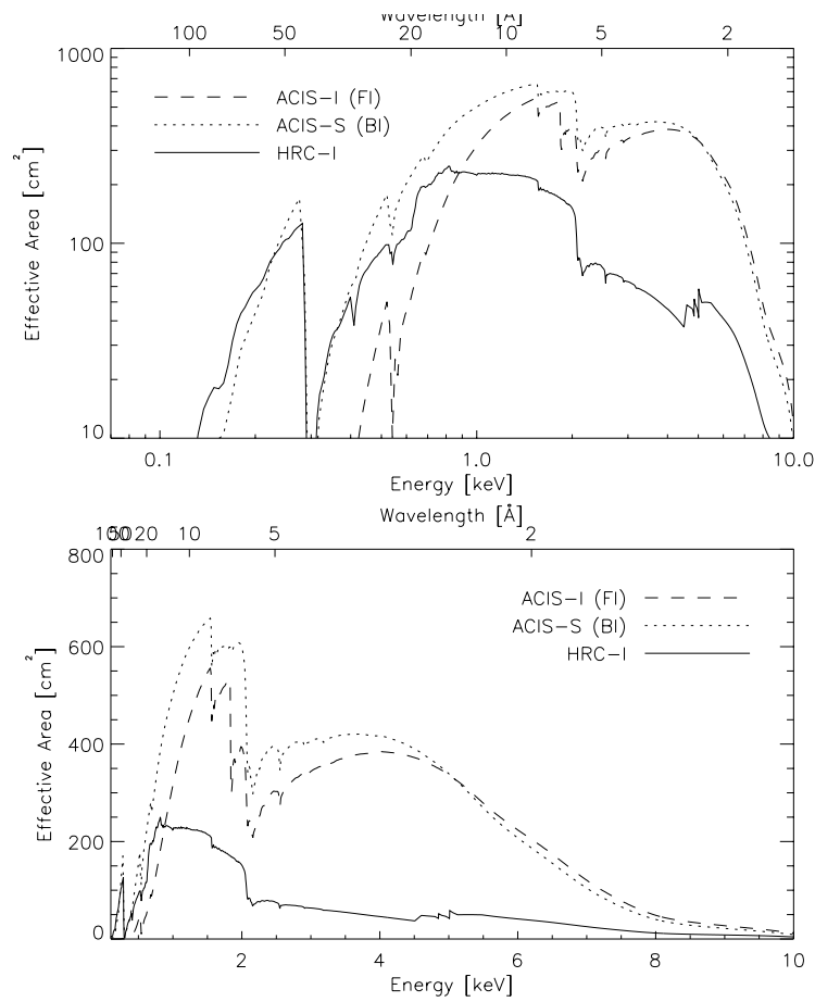
Figure 1.3: Comparison of the on-axis effective areas for observing a point source (integrated over the PSF ) of the HRMA/HRC-I, the HRMA/ACIS(FI), and the HRMA/ACIS(BI) combinations. Top panel is log and bottom panel is linear scale. The ACIS curves show the predicted values for the middle of Cycle 11 (2010-05-15).
