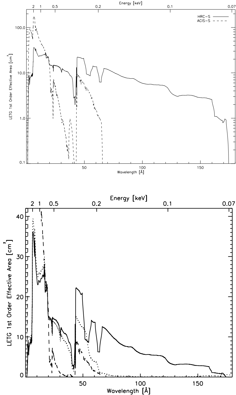
Figure 9.17: LETGS 1st-order effective area for an on-axis point source, with HRC-S and ACIS-S detector configurations with log (top) and linear (bottom) scaling. The bottom plot also shows the HRC-S/LESF combination (dotted line). Positive and negative orders are summed. LETG+ACIS-S areas were computed using an effective area model that included the effects of contamination build-up extrapolated to the level expected in mid-May 2009. Note that the vertical scale of the linear plot has been truncated.
