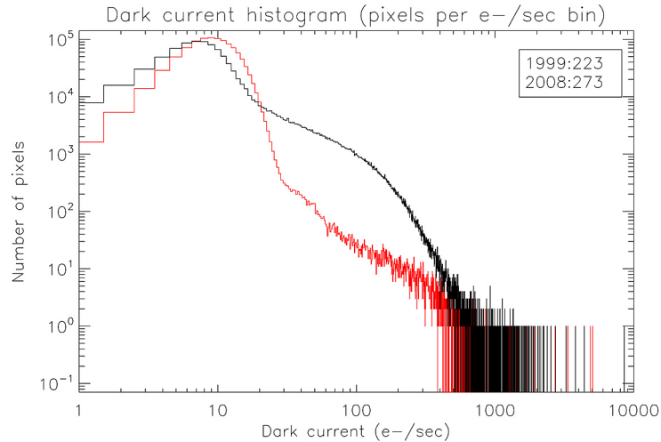
Figure 5.6: Differential histogram of dark current distribution for the ACA CCD in 1999-Aug and 2008-Sept
