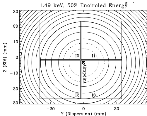
Figure 6.10: Approximate contours of constant 50% encircled energy at 1.49 keV when the ACIS-I default aimpoint is selected. The dotted line is 1 arcsec, the dashed line is 1.5 arcsec. The remainder are at 1 arcsec intervals. The thicker solid lines highlight the 5, 10, and 15 arcsec contours.
