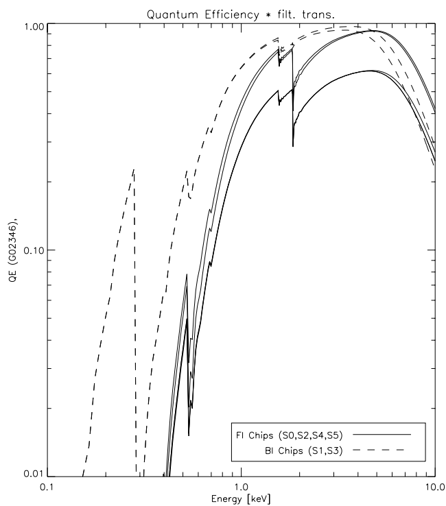
Figure 6.3: The quantum efficiency, convolved with the transmission of the appropriate optical blocking filter, of the FI CCDs (from a row nearest the readout) and the two BI CCDs as a function of energy. S3 is somewhat thicker, hence more efficient, than S1. This figure includes the effects of molecular contamination. There is also a small change, implemented in Cycle 9, near the Si K edge at 1.84 keV
