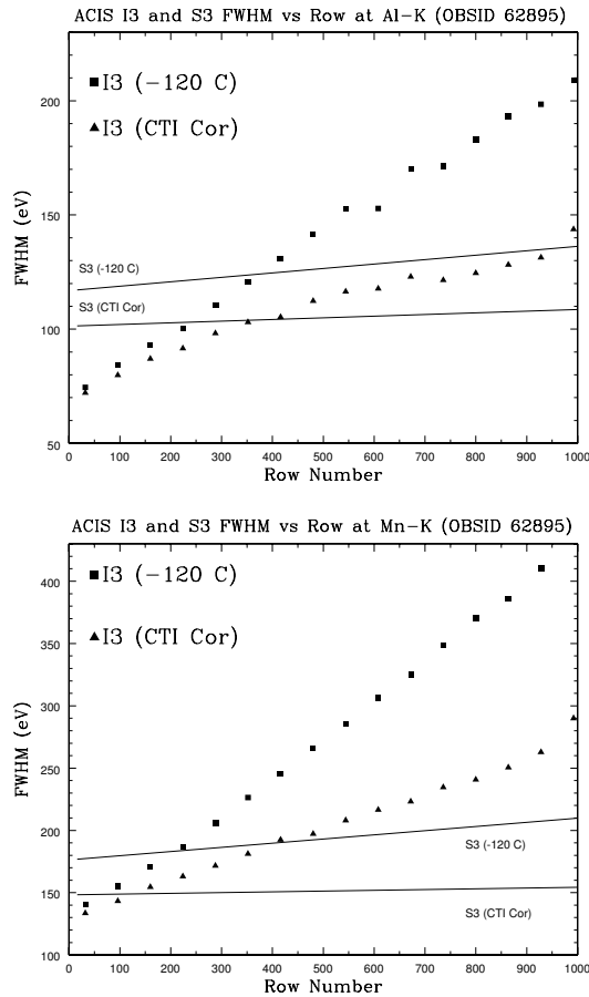
Figure 6.9: An example of the application of the CXC CTI-corrector in two energy bands. The upper plot shows data for the Al-K line (1.49 keV), and the lower for Mn-K (5.9 keV). The square data points are the FWHM of lines averaged over 32-row bins. The triangle data points are the FWHM of CTI-corrected lines. The upper line shows the uncorrected performance of the S3 chip, while the lower line shows the CTI-corrected performance of the S3 chip. These data are from March 2000.
