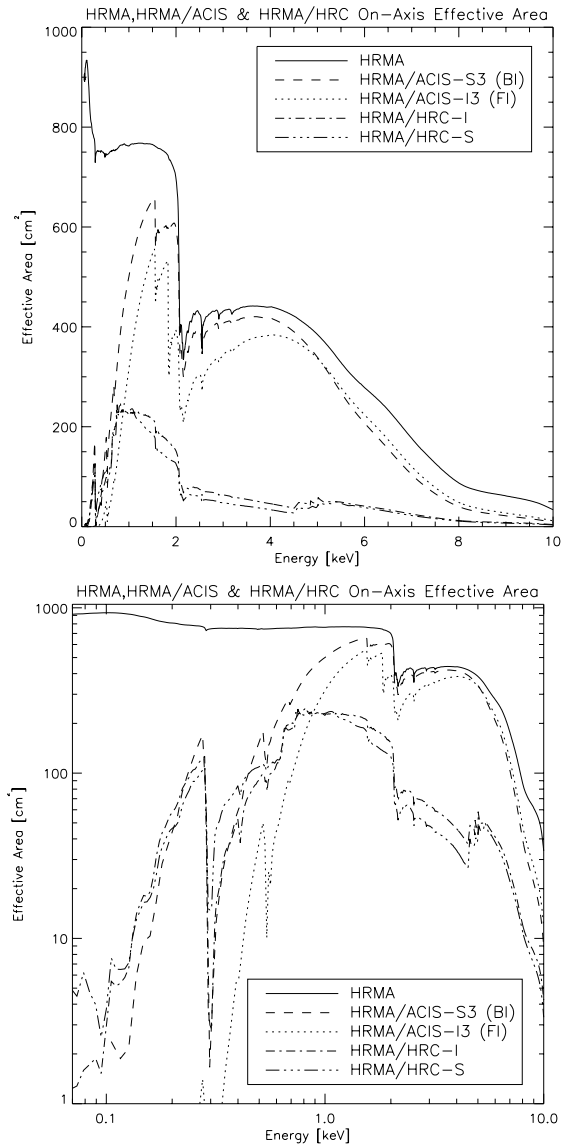
Figure 4.4: The HRMA/ACIS and HRMA/HRC effective areas versus X-ray energy in linear-linear (top) and log-log (bottom) scales. The structure near 2 keV is due to the iridium M-edge. The HRMA effective area is calculated by the raytrace simulation based on the HRMA model and scaled by the XRCF calibration data. The HRMA/ACIS effective area is the product of the HRMA effective area and the Quantum Efficiency (QE) of ACIS-I3 (front illuminated) or ACIS-S3 (back illuminated). The HRMA/HRC effective area is the product of HRMA effective area and the QE of HRC-I or HRC-S at their aimpoints, including the effect of UV/Ion Shields (UVIS). [Note: the colored lines are viewable in the electronic version]
