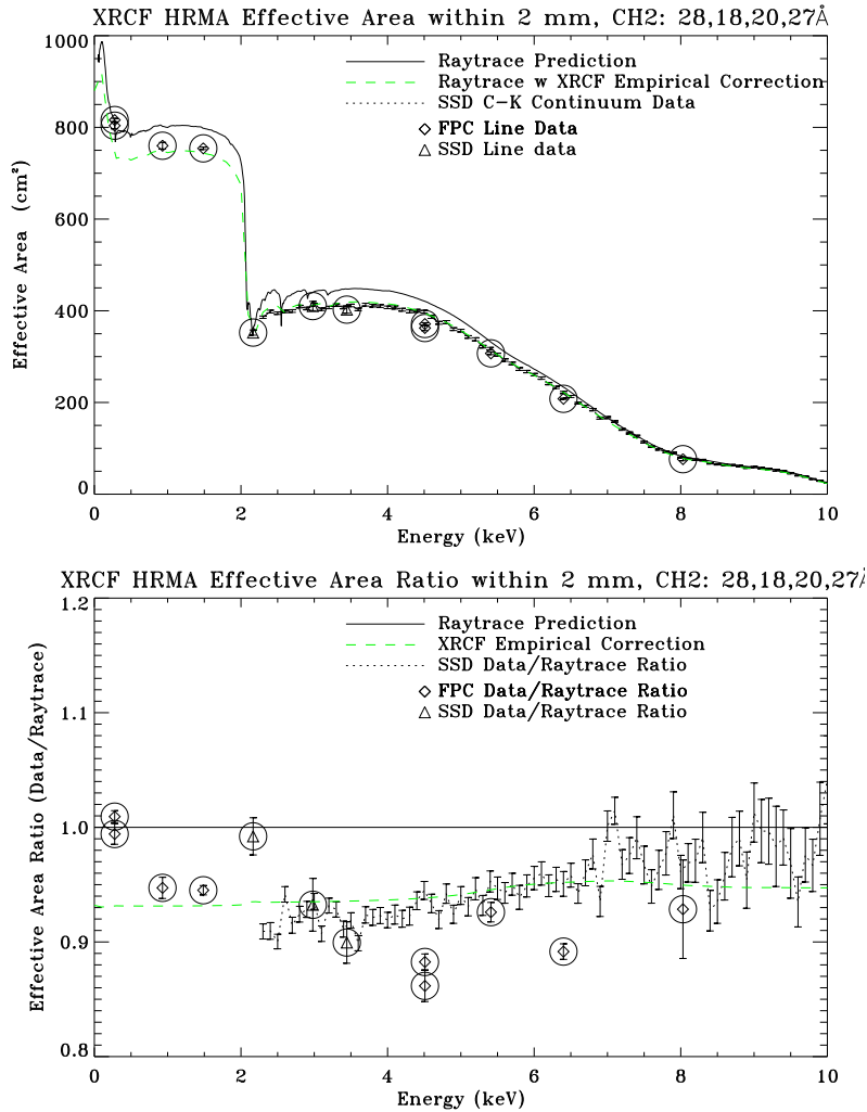
Figure 4.3: The HRMA Effective area: The raytrace prediction (top panel) and the ratio (bottom panel) of the XRCF measurements to the raytrace simulation are shown as a function of energy. The raytrace includes the effects of molecular contamination of variable thickness on the mirrors. The dotted line (to emphasize that these measurements were taken simultaneously) with error bars shows the data taken with a solid state detector (SSD) with a C-K continuum source. Data obtained from spectral line sources with a flow proportional counter (FPC) are shown as diamonds; obtained with a solid state detector (SSD) are shown as triangles. All the line measurements are circled for clarity. The dashed (green) line in the bottom panel shows the XRCF empirical correction to the raytrace based on the XRCF data. The dashed (green) line in the upper panel shows the absolute HRMA effective area with the XRCF empirical correction. [Note that the color is viewable only in the electronic version.]
