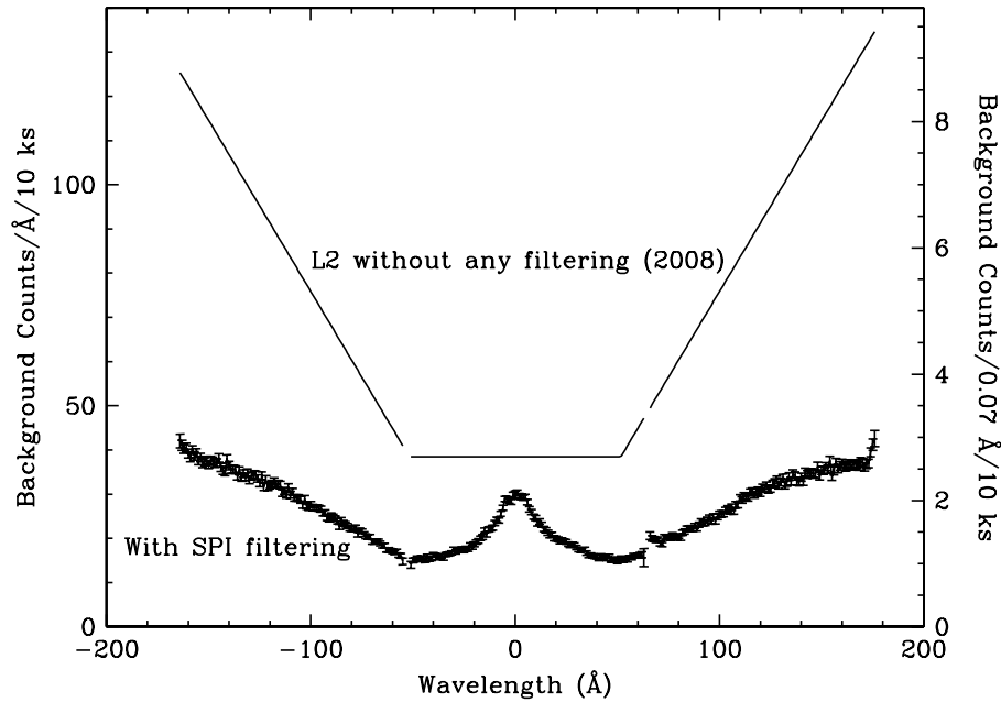
Figure 9.21: The LETGS+HRC-S background rate with and without the new SPI filter. Data are shown using the standard ‘bowtie’ spectral extraction region (see Figure 9.14). X-ray losses from the observed spectrum as a result of the filtering for 1st order are \sim 1.25\% ; losses will be slightly higher for higher orders. See the “LETG/HRC-S Background Filtering page” for more information.
