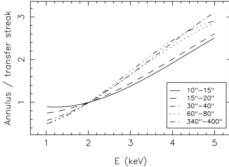
Figure 4.10: Hardening of the diffuse mirror scattering halo with distance from the image. The ratio of spectra extracted for a number of annuli centered on the specular image to the spectrum extracted from the ACIS transfer streak. The legend indicates the annular radii in arcsec.
