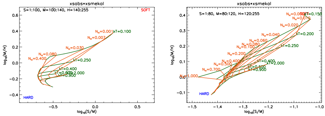
Figure 7.10: As in Figure 7.9, for a set of higher plasma temperatures.
