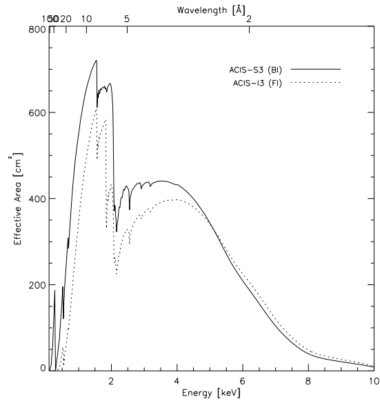
Figure 6.5: The HRMA/ACIS predicted effective area versus the energy on a linear scale. The dashed line is for the FI CCD I3, and the solid line is for the BI CCD S3.
