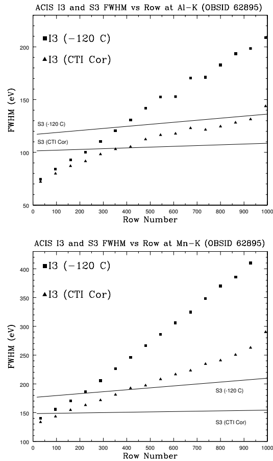
Figure 6.9: An example of the application of the CXC CTI-corrector in two energy bands. The upper plot shows data for the Al-K line (1.49 keV), and the lower for Mn-K (5.9 keV). The square data points are the FWHM of lines averaged over 32-row bins. The triangle data points are the FWHM of CTI-corrected lines. The upper line shows the uncorrected performance of the S3 chip, while the lower line shows the CTI-corrected performance of the S3 chip. These data are from March 2000.
