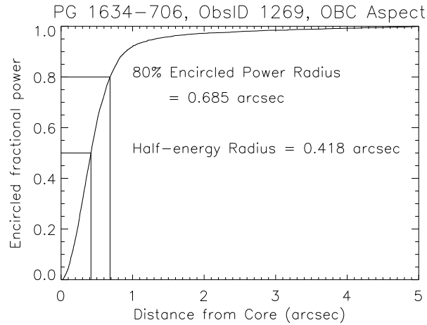
Figure 6.7: The on-orbit encircled broad-band energy versus radius for an ACIS observation of point source PG1634-706 (ObsID 1269). The effective energy is 1 keV.
