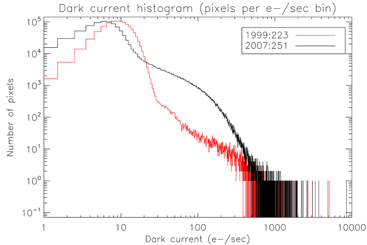
Figure 5.6: Differential histogram of dark current distribution for the ACA CCD in 1999-Aug (gray) and 2007-Sept (black)
