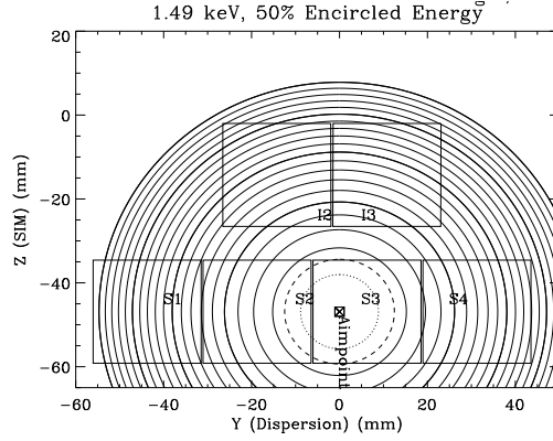
Figure 6.11: Approximate contours of constant 50% encircled energy at 1.49 keV when the ACIS-S default aimpoint is selected. The dotted line is 1 arcsec, the dashed line is 1.5 arcsec. The remainder are 1 arcsec intervals. The thicker solid lines highlight the 5, 10, 15 and 20 arcsec contours.
