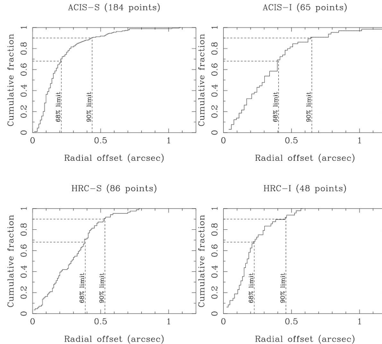
Figure 5.4: Cumulative histogram of celestial accuracy for Chandra X-ray source locations for each SI. Radial offset is the distance in arcsec between the optical coordinate, typically from the Tycho-2 catalog, and the Chandra position.
