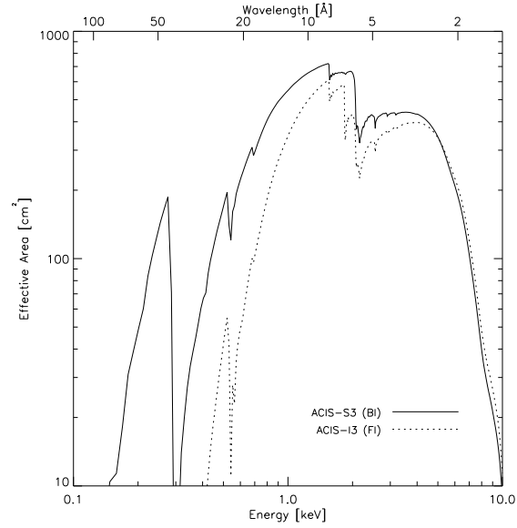
Figure 6.4: The HRMA/ACIS predicted effective area versus the energy on a log scale. The dashed line is for the FI CCD I3, and the solid line is for the BI CCD S3.
