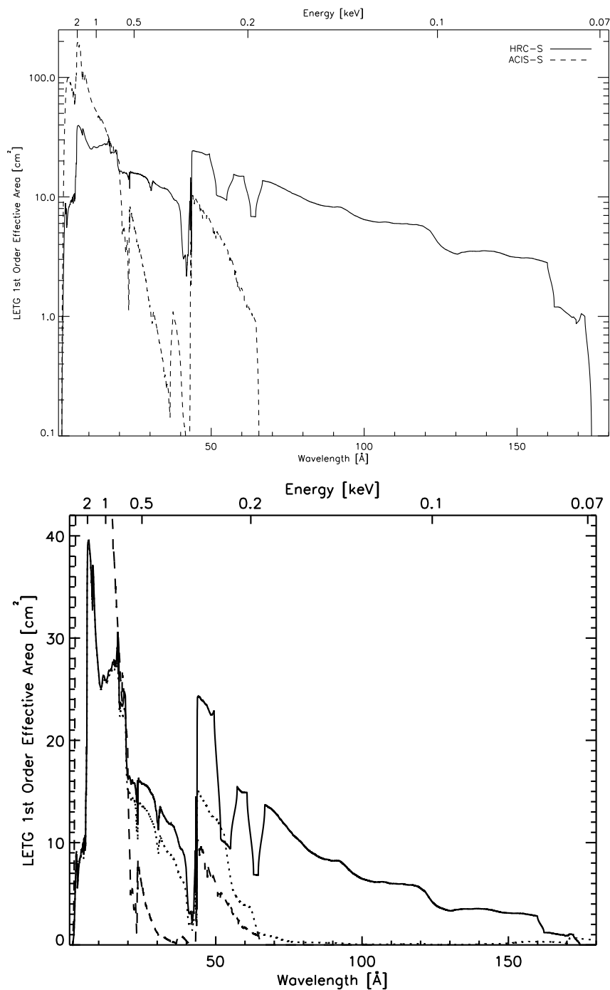
Figure 9.17: LETGS 1st-order effective area for an on-axis point source, with HRC-S, HRC-S LESF and ACIS-S detector configurations with log and linear scaling. Positive and negative orders are summed. LETG+ACIS-S areas were computed using an effective area model that included the effects of contamination build-up extrapolated to the level expected in mid-May 2009. Note that the vertical scale of the linear plot has been truncated.
