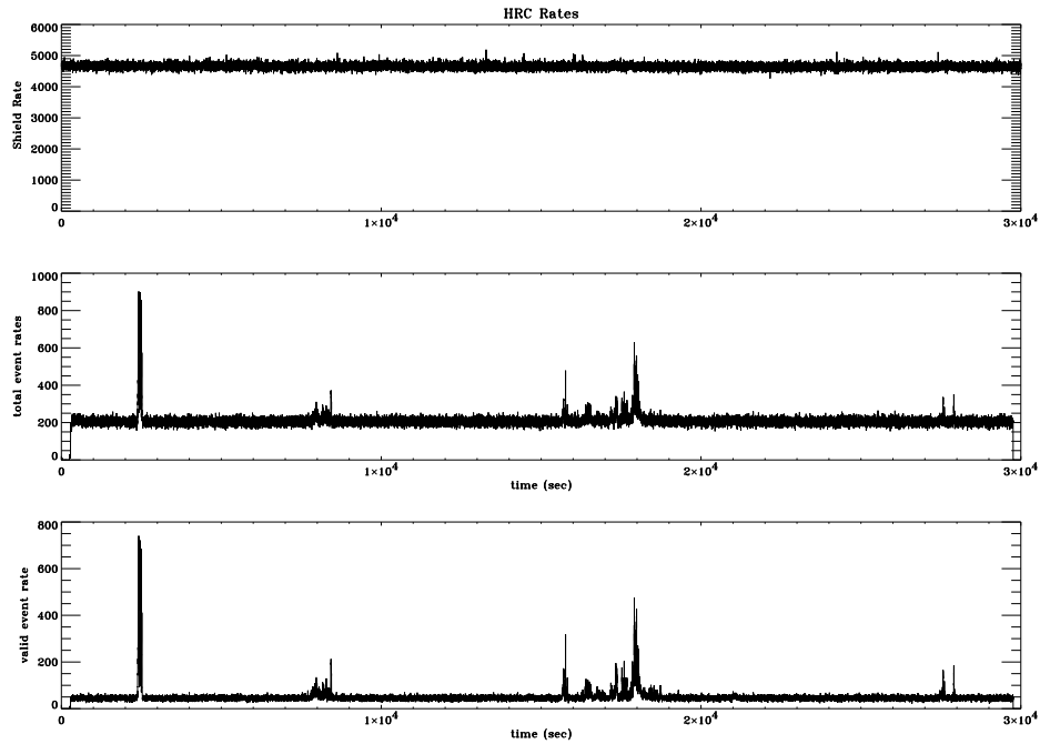
Figure 7.18: An example of the background variability during a \sim 30 ks HRC-I observation of the SNR G21.5-09 taken on 1999-10-25. The total event rate (middle) and valid event rate (bottom) show correlated bursts up to \sim 800 \text{cts s}^{-1} . The bursts are uniformly distributed over the detector. The anti-coincidence shield (top) exhibits no correlated enhancements. The total and valid rates differ by \sim 200 \text{cts s}^{-1} due primarily to cosmic ray events that are vetoed and don't appear as valid events in the telemetry.
