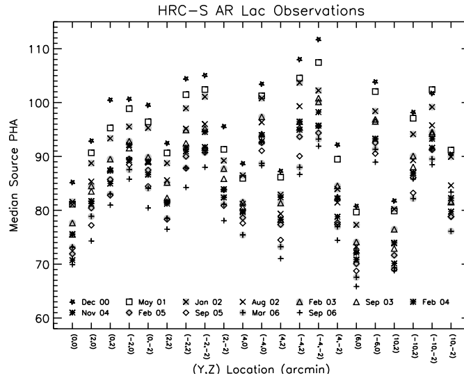
Figure 7.13: As in Figure 7.12, for the HRC-S. When there are two observations in a year, the first one is shown shaded. The same temporal trend is seen as for HRC-I in Figure 7.12.
