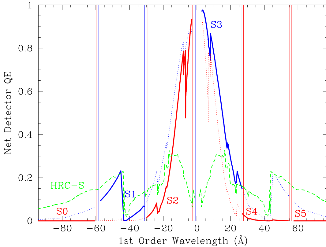
Figure 9.6: Comparison of QEs of ACIS FI and BI chips (and the HRC-S) when used with the LETG. QEs shown above are for Y-offset = +1.5' (0 for HRC-S). Y-offsets may be chosen to tailor the coverage of BI chips (S1 and S3; top/blue QE curve), which have higher QE at low energies than the FI chips (S0,S2,S4,S5; bottom/red curve). Dashed (green) line is for HRC-S, thick solid curves are for ACIS. Vertical lines indicate ACIS chip gaps (with dither, 1.5 Å). For clarity, -3 to +3 Å is not shown for ACIS. See Section 9.4.2/Offset Pointing for more information regarding the choice of Y-offset.
