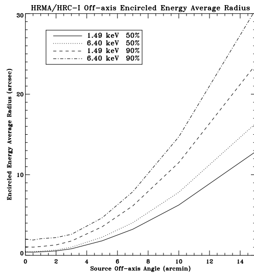
Figure 7.6: Encircled energy as a function of source off-axis angle for 50% and 90% encircled energy for 1.49 and 6.40 keV for the combined HRMA/HRC-I. A conservative contribution from the aspect solution is included ( \text{FWHM} = 20 \mu\text{m} ( 0.41'' )). A plot for the HRC-S would be almost identical since the PSFs of the two instruments are virtually identical and independent of off-axis angle.
