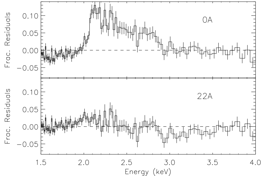
Figure 4.5: Combined residuals from power law fits to 18 blazar observations (Marshall, H.L., 2005). The residuals in the upper panel are based upon models of contaminant free optics, while those in the lower are based upon a model of the mirror surfaces which includes a thin (22Å) hydrocarbon layer. Features in observations near the Ir M edges should be regarded with skepticism.
