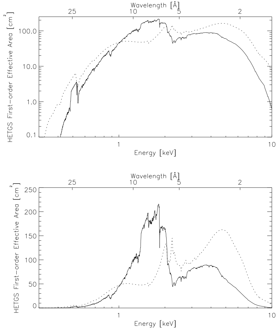
Figure 8.11: The modelled total first-order (solid curve) and zeroth-order (dotted curve) effective area, integrated over the PSF, of the HRMA-HETG-ACIS-S combination, as a function of energy. The first-order data are the same as those plotted in Figures 8.7 and 8.9. The plotted first-order values are the sums of the area at a particular energy from both orders (+/-) of both MEG and HEG spectra. Both a log-log and a log-linear version are shown.
