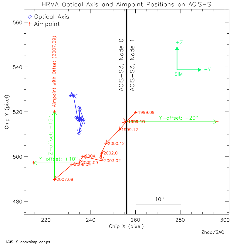
Figure 6.12: Position of the optical axis on the S3 CCD at various times in the mission. Since 1999, the aimpoint (position of optimal focus) has drifted (dark lines), and default pointing offsets (lighter lines) have been changed several times to move the image away from the node boundary. Dates are given in format YYYY.MM (year, followed by month).
