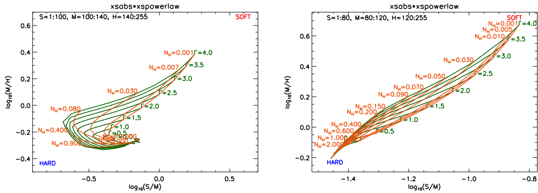
Figure 7.8: The color-color grid for a power-law spectral model, calculated for the HRC-I ( left ) and the HRC-S ( right ). The PI channels are grouped into three bands, S = 1 : 100 , M = 100 : 140 , and H = 140 : 255 for the HRC-I, and S = 1 : 80 , M = 80 : 120 , and H = 120 : 255 for the HRC-S, and their logarithmic ratios are plotted along the two axes for specific values of the model parameters \Gamma (the index of the power-law function) and N_H (the absorbing column density in units of 10^{22} \text{ cm}^{-2} ).
