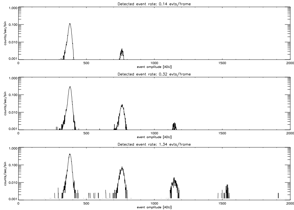
Figure 6.16: The effects of pileup at 1.49 keV (Al K\alpha ) as a function of source intensity. Data were taken during HRMA-ACIS system level calibration at the XRCF. Single-photon events are concentrated near the pulse height corresponding to the Al K\alpha line ( \sim 380 ADU), and events with 2 or more photons appear at integral multiples of the line energy.
