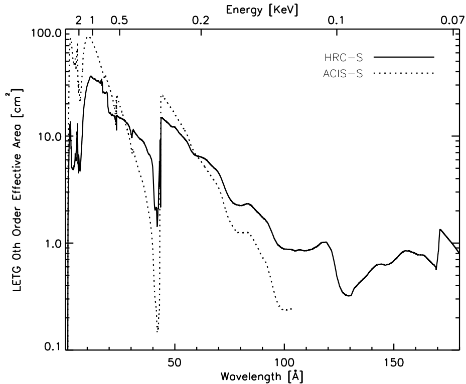
Figure 9.16: LETGS 0th-order effective area for an on-axis point source for the LETG with HRC-S and ACIS-S detectors. The 0th-order effective area for the HRC-S/LESF combination is the same as for the HRC-S. LETG+ACIS-S areas were computed using an effective area model that included the effects of contamination build-up extrapolated to the level expected in mid-May 2009.
