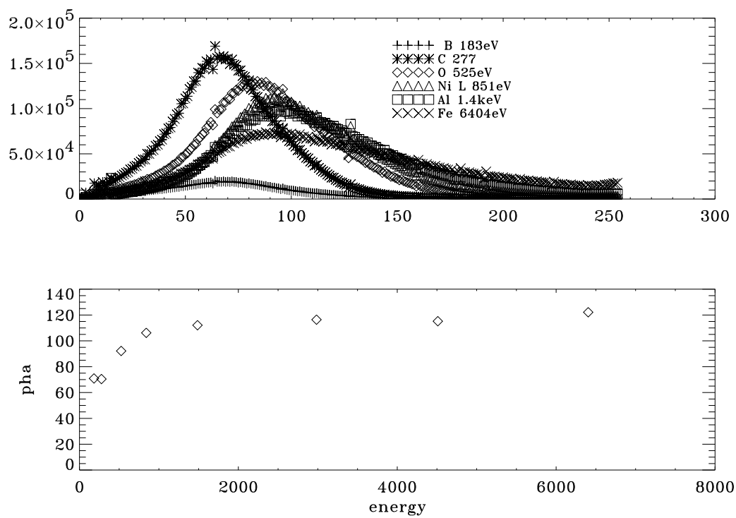
Figure 7.7: Pulse height versus energy for the HRC-I detector (top) and the centroid of the pulse height distribution versus energy (bottom). These data were obtained at SAO during flat field, normal-incidence-illumination tests. The voltage settings have been changed in-flight and thus the applicability of these data is questionable. They are presented here only for illustrative purposes.
