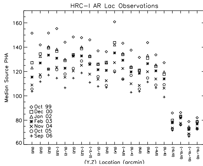
Figure 7.12: The median PHA derived for AR Lac observations carried out at numerous locations across the HRC-I detector. There also exist intrinsic variations in the spectrum which have not been accounted for in this figure. The values from data obtained at different years are shown with different symbols. Note the steady decline in the median PHA with time for all pointings.
