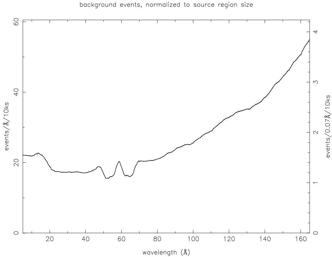
Figure 9.28: The LETG+HRC-S background count rate in the spectral extraction window as a function of wavelength for use in observation planning. Both + and – orders have been combined. These curves correspond to the “medium” (2% X-ray loss) PH filter described in the text. The left y axis is in units of \text{cts}/\text{\AA}/10\text{ ks} , while that on the right is in units of \text{cts}/0.07\text{ \AA}/10\text{ ks} ; the latter corresponds to a typical line width over which most of the observed flux is distributed in the case of an intrinsically narrow spectral line compared to the instrument LRF.
