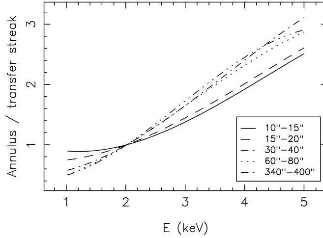
Figure 4.10: The ratio of the spectrum in a given annulus to the spectrum in the central core as a function of energy all normalized to 1 at 2 keV. The central core spectrum was determined from the "transfer streak" to minimize pileup which was still \sim 4\% .
