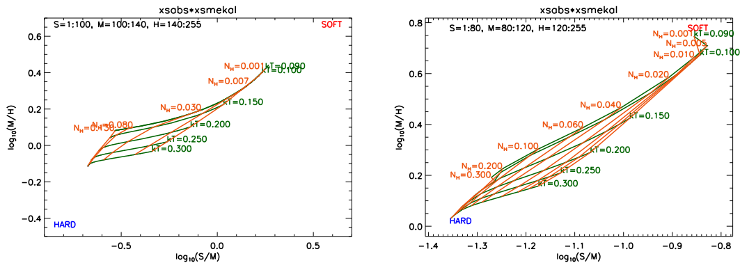
Figure 7.9: As in Figure 7.8, for a MEKAL thermal model at relatively low temperatures. The loci of constant plasma temperature ( kT ) are labeled by their value in keV.
