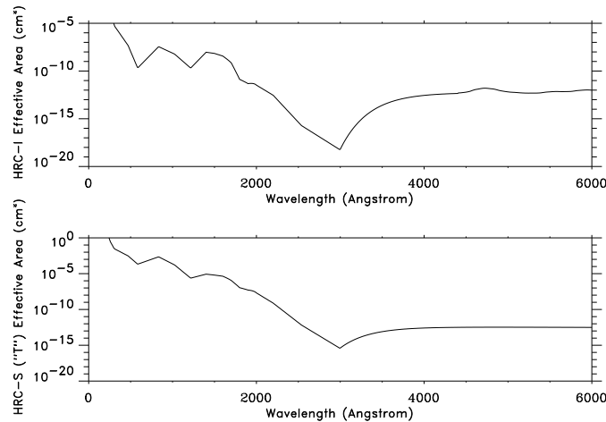
Figure 7.16: The HRC-I (top) and the center section of the HRC-S (bottom) UV/Ion shield effective area as a function of wavelength.
