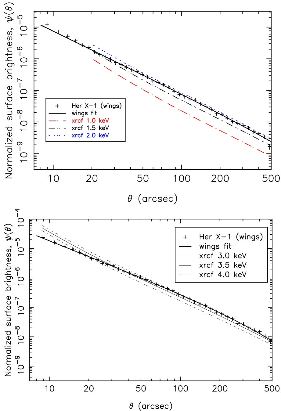
Figure 4.9: Radial profile of the Her X-1 scattering wings. Upper panel: 1.0-2.0 keV. The heavy solid line is a powerlaw plus exponential cutoff fit to the data; the heavy dash-dot lines are results from an empirical model based on ground testing for 1.0, 1.5, and 2.0 keV (lower curve to upper curve). Lower panel: Radial profiles of the Her X-1 scattering wings for 3.0-4.0 keV. The results for the empirical ground-based model are also plotted.
