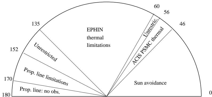
Figure 3.3: Diagram to illustrate ranges of solar pitch angle (the angle between the pointing direction and the satellite-Sun line) within which different observing limitations apply. Table 3.1 provides quantitative estimates for the observing limitations in the solar pitch angle ranges shown in the drawing.
