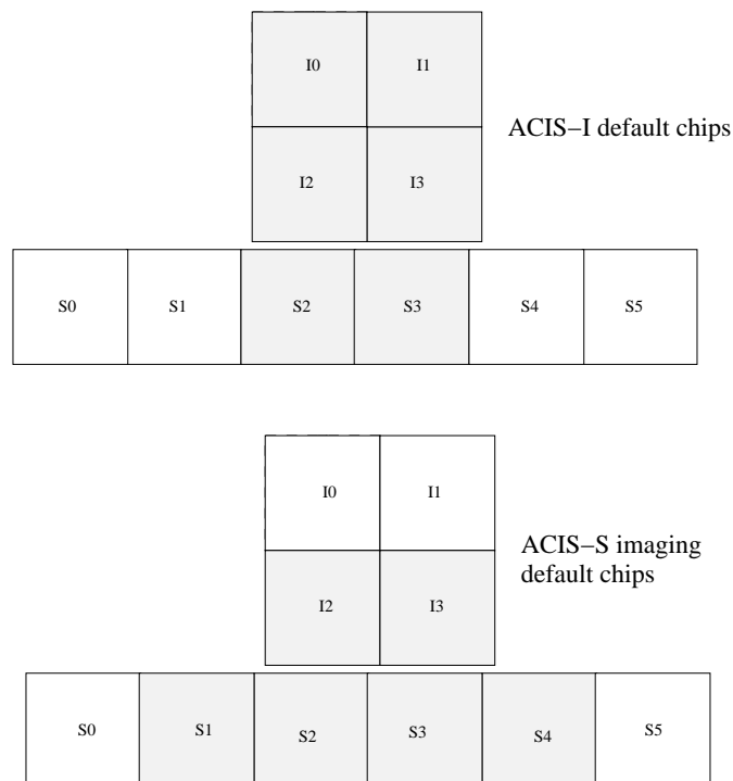
Figure 6.2: A schematic drawing of the ACIS focal plane, not to scale. The ACIS-I array consists of chips I0-I3. Chips S2 and S3 are often turned on in addition to I0-I3 when ACIS-I is used in imaging mode as indicated in the top figure. ACIS-S consists of chips S0-S5. When operated in imaging mode chips S1-S4 plus I2 and I3 are often turned on (bottom figure). When operated in spectroscopy mode S0-S5 are usually turned on. See 6.20.1 for more details on chip choices.
