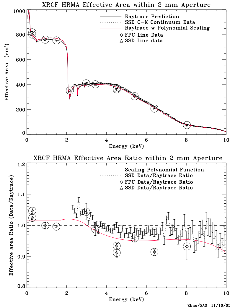
Figure 4.2: The HRMA effective area at the XRCF. Top panel: the solid line is the raytrace simulation of the effective area within a 2 mm diameter aperture at the focus; the dashed line with error bars shows the data taken with a solid state detector (SSD) with a C-K continuum source; the symbols in big circles show data taken with a flow proportional counter (FPC: diamonds) or SSD (triangles) with spectral line sources. The bottom panel shows the deviation of the data from the raytrace: the dotted line is the ratio of the SSD C-K continuum data to the raytrace; the diamonds and triangles show the ratio of the FPC and SSD data to the raytrace, respectively. Also shown (in red) is a solid line that represents the results of fitting a polynomial to the data. This fit gave equal weight to the deviations of the continuum and line measurements. [Note the red line is viewable in the electronic version.]
