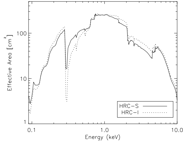
Figure 7.17: The effective area of the HRMA/HRC-I (dashed line) and the central segment of the HRMA/HRC-S in imaging mode (solid line) integrated over the full PSF . Absorption edges are due to the iridium coating on the mirrors, the CsI MCP coating, and the polyimide/Al of the UVIS.
