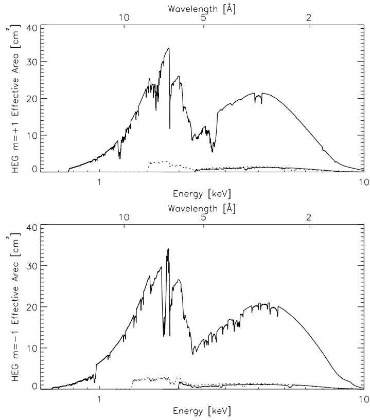
Figure 8.8: The HETGS HEG effective area: same caption as previous figure, except the vertical scale is now linear.
