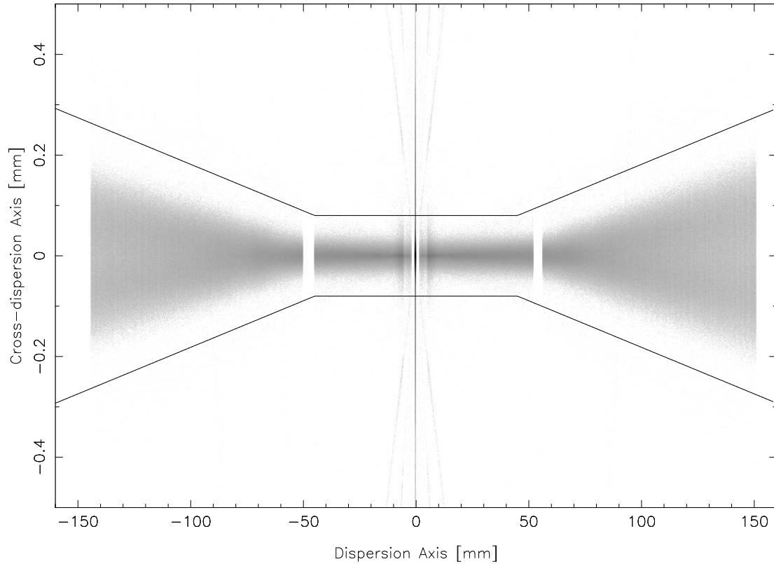
Figure 9.14: A MARX simulation of a flat spectrum illustrating the broadening of the LETG+HRC-S profile in the cross-dispersion direction, and showing the “bow-tie” spectral extraction window. The cross-dispersion profile of an LETG+ACIS-S spectrum is approximately constant across its smaller wavelength range and the default extraction window is rectangular.
