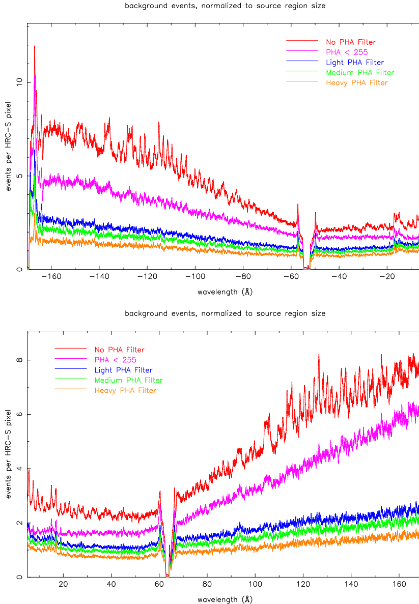
Figure 9.21: The LETG+HRC-S background from an observation of Capella. Spectra were derived from standard ‘bowtie’ background extraction region (see Figure 9.14). The curves from the top down correspond to: background spectrum with no PI filtering; minimal filtering (PHA=255 events removed) with 0% X-ray event loss; light filtering with 0.5% X-ray loss; 2% X-ray loss; and 5-15% X-ray loss. X-ray losses are for 1st order; losses will be slightly higher for higher orders, especially with heavier filtering. PI filtering can not be applied at wavelengths shorter than 6 Å. The units of the y axis are total events/dispersion-pixel (summed in the cross dispersion direction), where one HRC pixel is 6.43 \mu\text{m} wide ( 0.0074 \text{ \AA} ). The exposure time was 85 ks.
