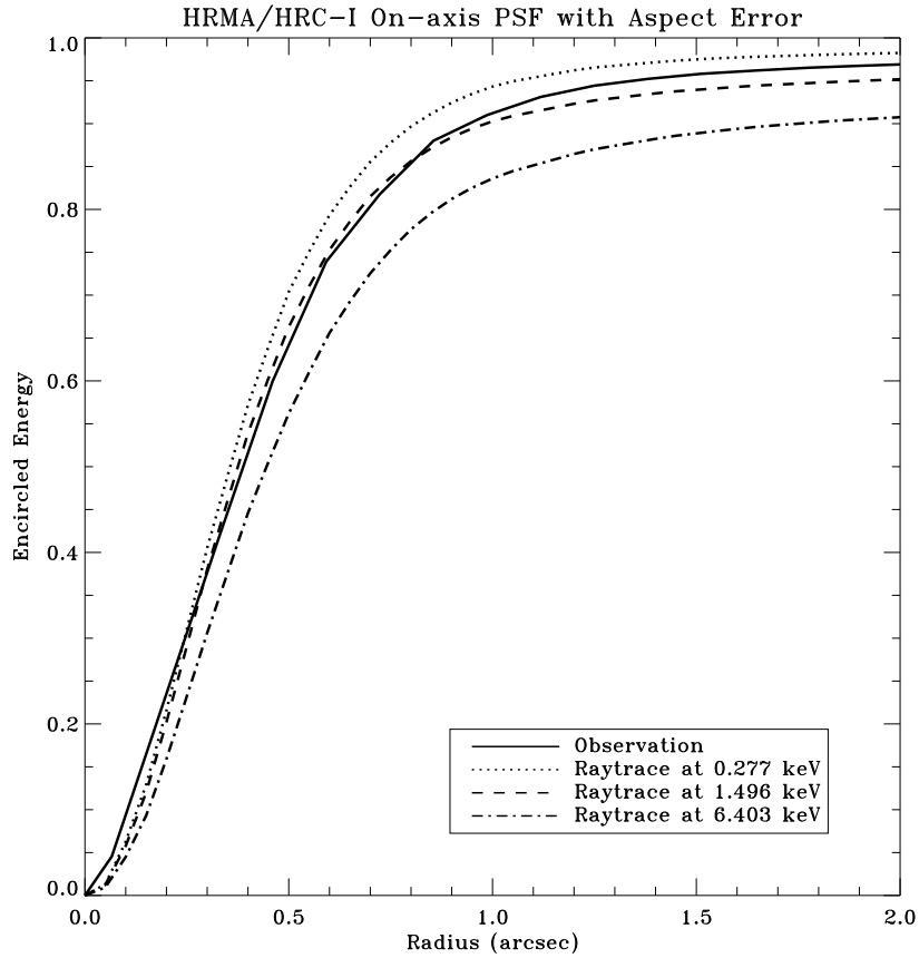
Figure 4.18: The HRMAHRC-I on-axis fractional encircled energy as a function of angular radius from a point source (Ar Lac) observed in flight compared to raytrace simulations for an on-axis point-source at selected X-ray energies, including the aspect uncertainties and the HRC-I pixelization effects.
