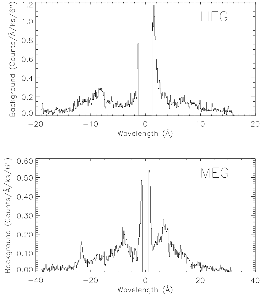
Figure 8.24: The background spectrum is plotted for the HEG (top) and MEG (bottom) for a long observation of the late-type star HR 1099 (observation ID 62538). The background was normalized to a 6 arcsec wide aperture but determined from a substantially larger region out to 50 arcsec from the source dispersion line. The spectrum was binned to 0.1 Å to show details of structure that may be observed in a typical HETGS observation. The spikes near zeroth order are due to increased background included in the pulse height selection at high energies.
