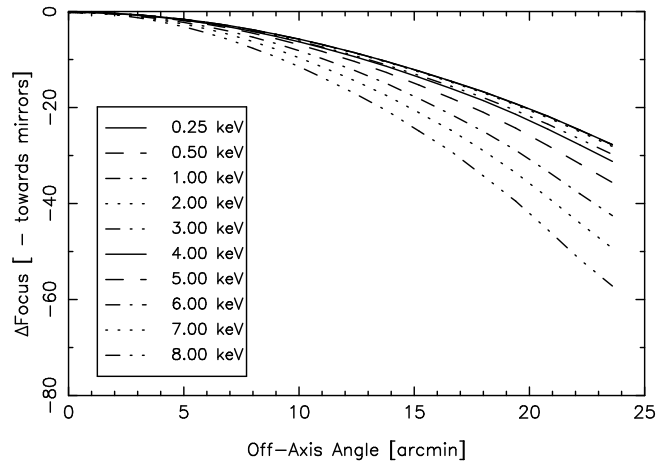
Figure 4.11: The HRMA focal surface (from simulations), indicating its dependence on energy and off-axis source position. It deviates more from the detector planes at higher energies and larger off-axis angles, leading to significant degradation of image quality.
