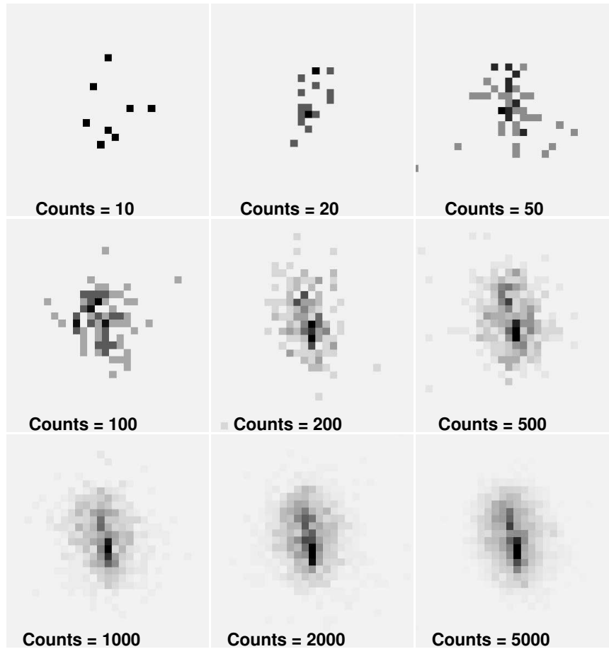
Figure 4.16: A simulated 1.49 keV point source at an off-axis angle of 5' , binned to ACIS pixels. The panels show what the source would look like with a varying number of counts. Note how the morphology is a strong function of the number of counts, and how even with a large number of counts one might mistake it for an extended source or even for multiple sources.
