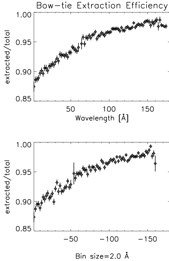
Figure 9.15: The spectral extraction efficiency for 1st order, representing the fraction of the power diffracted into the LETG 1st order that is enclosed within the default CIAO “bow-tie” spectral extraction window as a function of 1st order wavelength. The “missing” power at long wavelengths is primarily due to diffraction of photons outside of the extraction region by the fine support structure, while scattering losses dominate at shorter wavelengths. These extraction efficiencies were determined using MARX raytrace simulations. In-flight data, though noisier, have been found to agree with these efficiencies to a level of about 5% or better. The uncertainty in the effective area calibration resulting from the extraction efficiency alone is therefore less than 1%.
