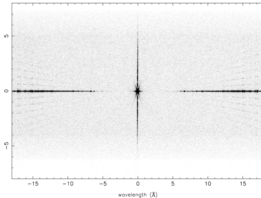
Figure 9.22: HRC-S detector image of LETGS observation of Capella. In order to illustrate the stretching of the cross-dispersion axis, both axes are in \text{\AA} with 1.148 \text{ \AA}/\text{mm} ; only the central 30 mm of the central plate is shown. The full extent of the telemetered six-tap cross-dispersion window is shown and measures 9.9 mm. The areas of reduced background at top and bottom are due to dither effects. Star-shaped coarse support structure diffraction is seen around zeroth order, and “cat’s whiskers” fine support structure diffraction is seen above and below the primary dispersion axis, as well as in the vertical line through 0th order.
