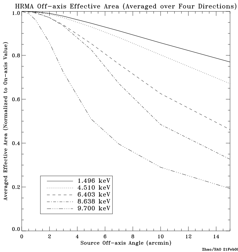
Figure 4.4: The HRMA effective area versus off-axis angle, averaged over four azimuthal directions, for selected energies, normalized to the on-axis area for that energy.
