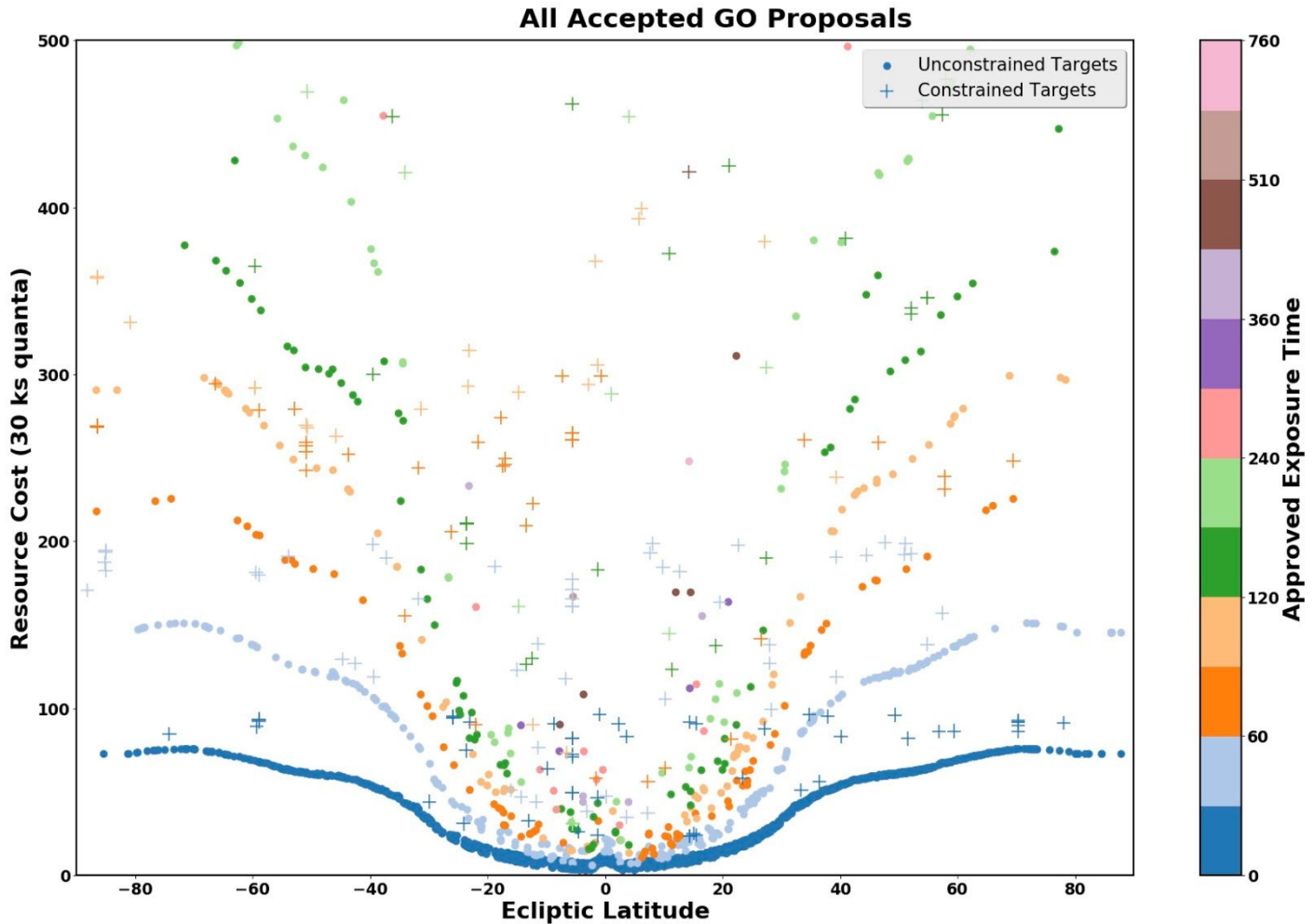
Figure 1: Plot of Resource Cost (RC) values for observing programs from Chandra Cycles 14-21, calculated using RC formulation for Cycle 22. Circles correspond to observations without constraints, for which RC values depend only on ecliptic latitude (X-axis) and exposure time (color bar at right) in units of 30 ks segments (rounded up to nearest integer). Crosses correspond to targets with observing constraints, for which the nature and difficulty of the constraint is compounded with the values associated with the sky position and exposure time. The plot is truncated at RC values of 500, but larger values can result for highly-constrained, long observations.
