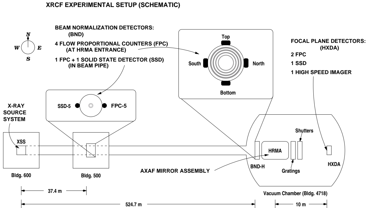
Figure 1.1: Schematic of XRCF
