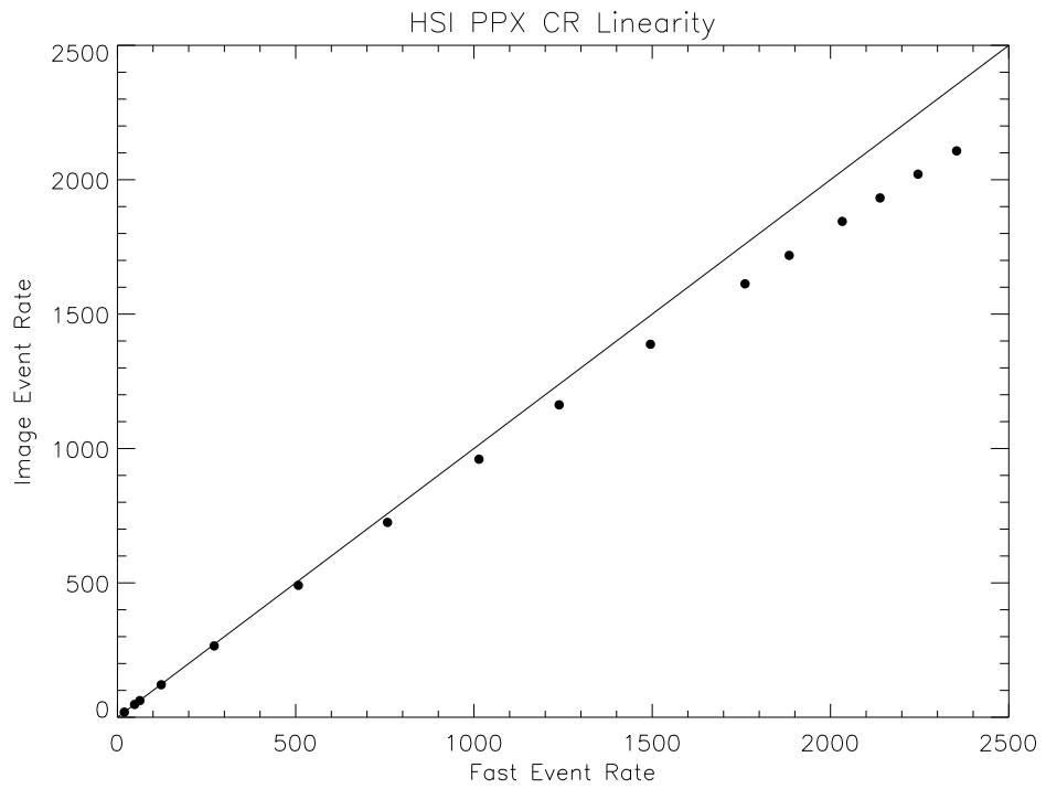
Figure 7.3: HSI post-processing electronics image count rate linearity
