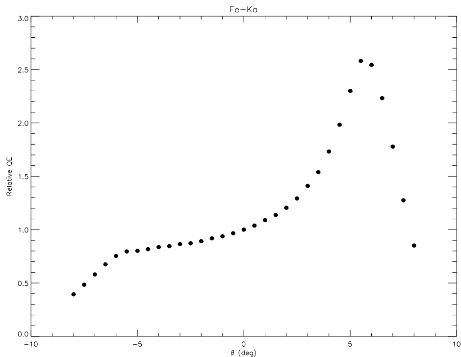
Figure 7.1: (continued) Fe-K.
