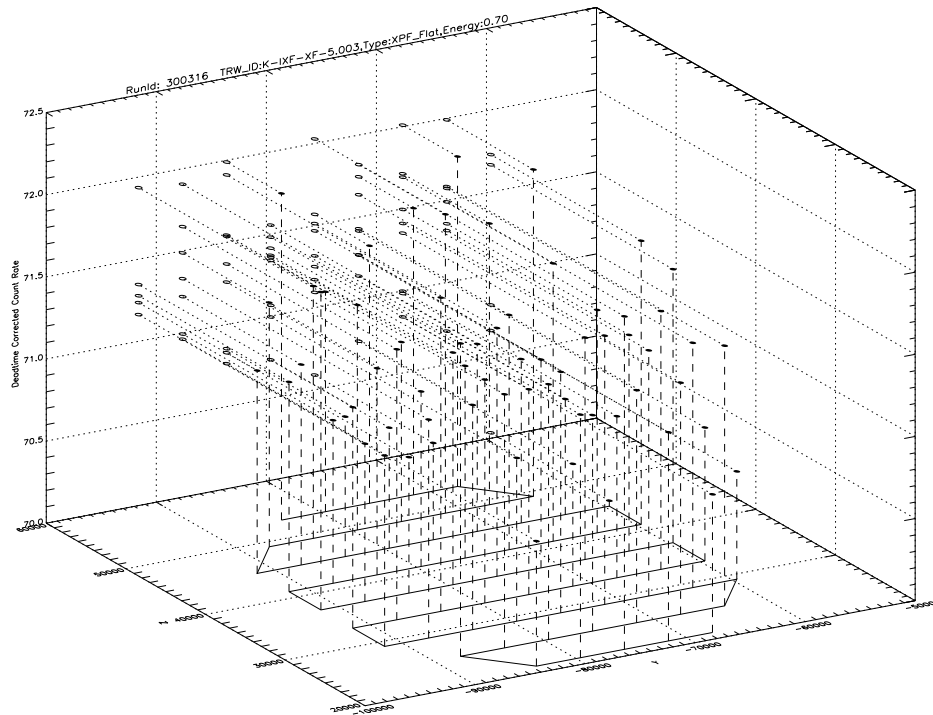
Figure 7.4: Sample flat field FPC scan pattern
