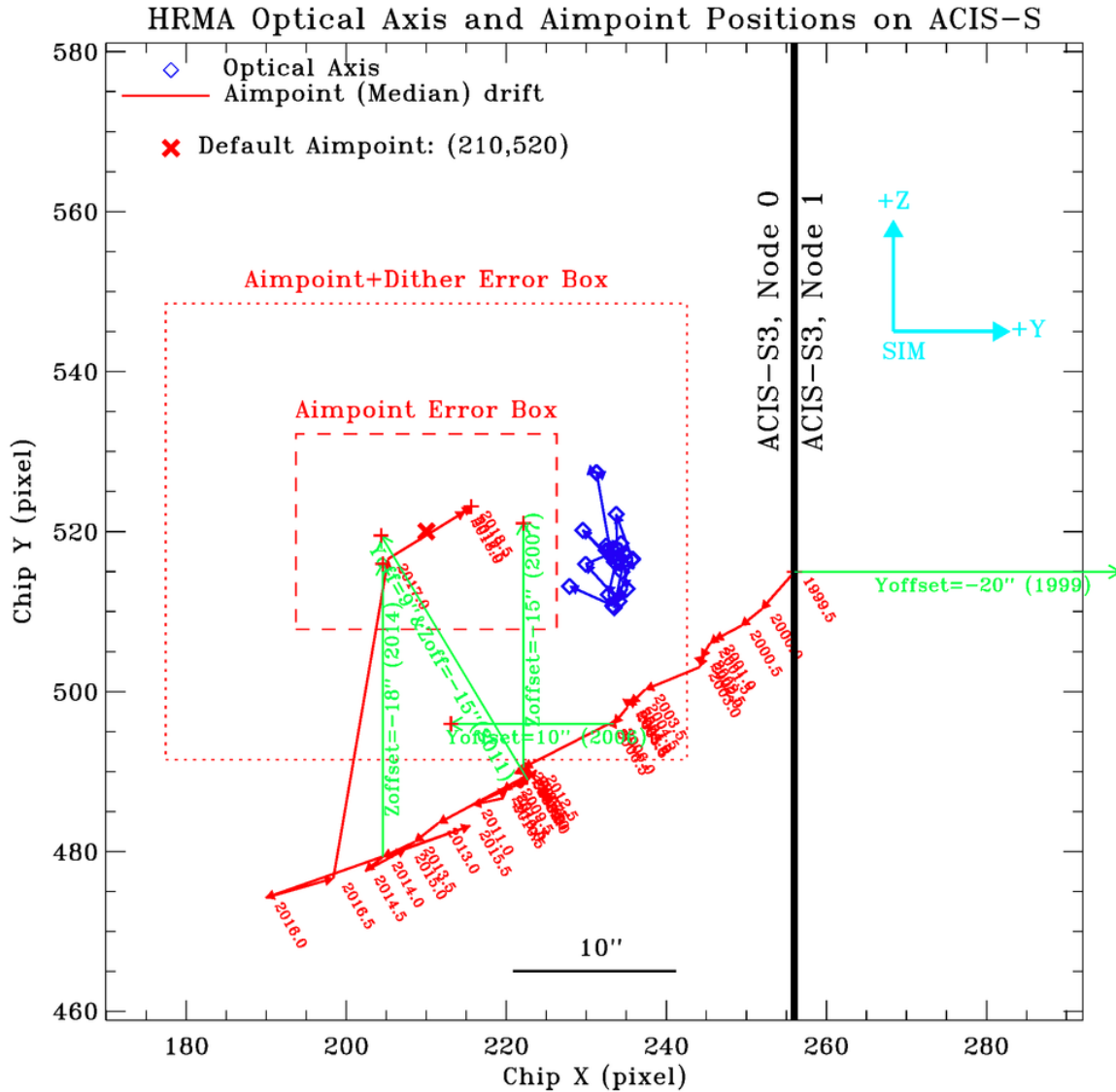
Figure 17: Chandra optical axis (blue) and median aimpoint (red, see Fig. 12) positions in half year bins on ACIS-S. Each aimpoint position is labeled by the year. The green arrows in the figure show the default offsets (starting in the year labels next to the green arrows) applied before 2016. All the observations were conducted with these default offsets, unless the observers requested otherwise. Starting in 2016 (Cycle 18), aimpoint is dynamically adjusted to put at the permanent default position (marked as red “x”) near the optical axis. The dotted and dashed rectangles are the error boxes of the default aimpoint implementation, with and without the dither. The cyan colored arrows show the SIM coordinates.
