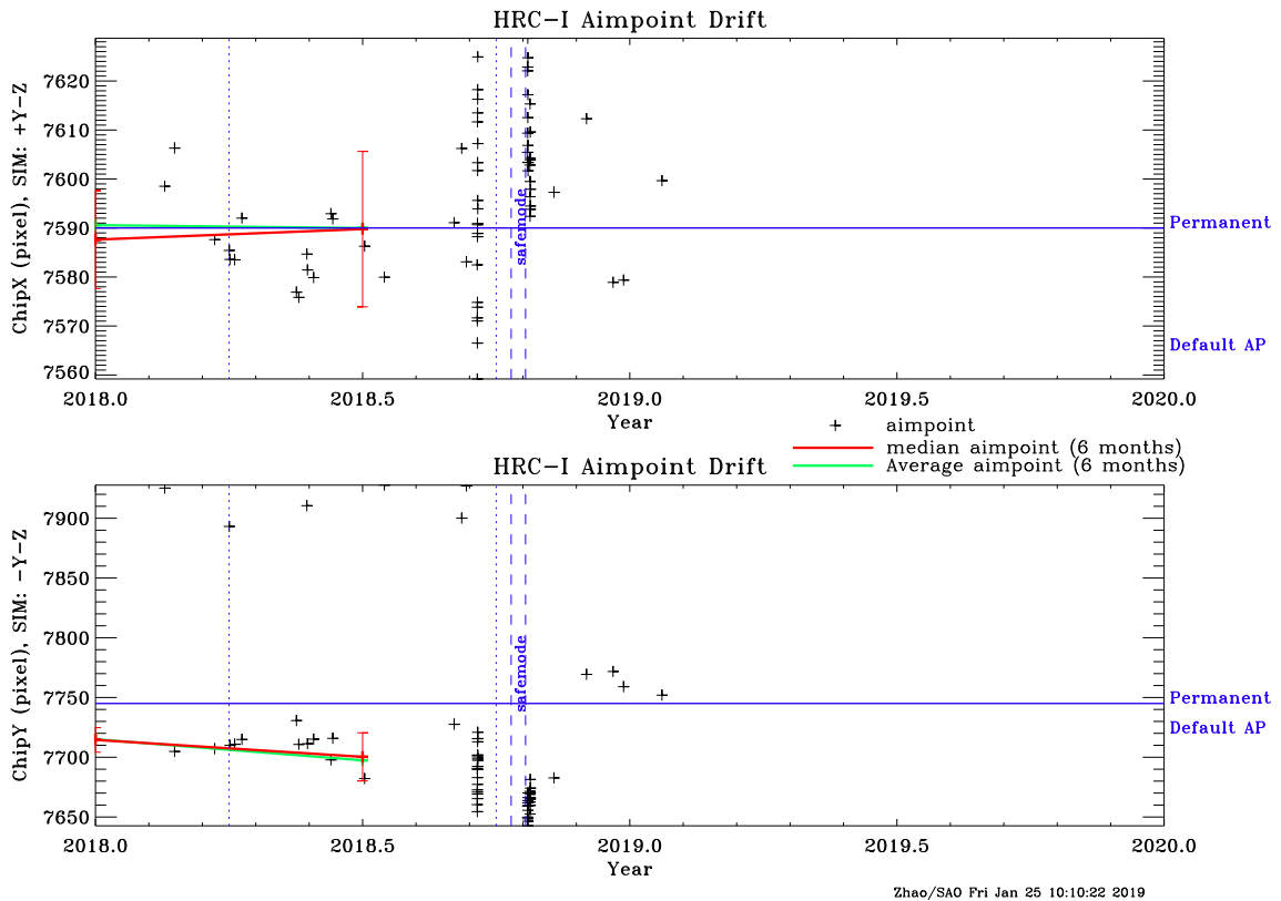
Figure 7: Aimpoint position as a function of time on HRC-I in the past year. The gap between the two vertical dashed lines indicate when Chandra was in safemode (Oct. 10–21, 2018).
