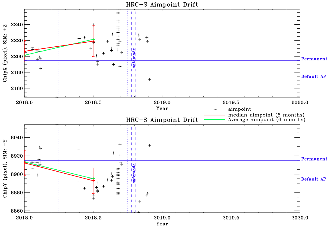
Figure 9: Aimpoint position as a function of time on HRC-S in the past year. The gap between the two vertical dashed lines indicate when Chandra was in safemode (Oct. 10–21, 2018).
