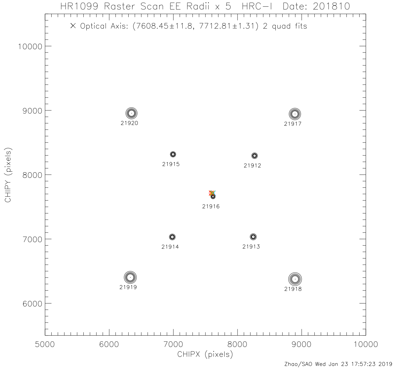
Figure 25: The first HRC-I raster scan observation of HR1099 during the HRMA cool down (in the morning of 2018-10-22). Circles around each observation point have the 50% – 90% encircled energy radii \times 5 . The numbers under the circles are the OBSIDs of the observations. The data are fit to two orthogonal 1-D quadratic equations. The optical axis is at the intersection of two minimum coordinates.
