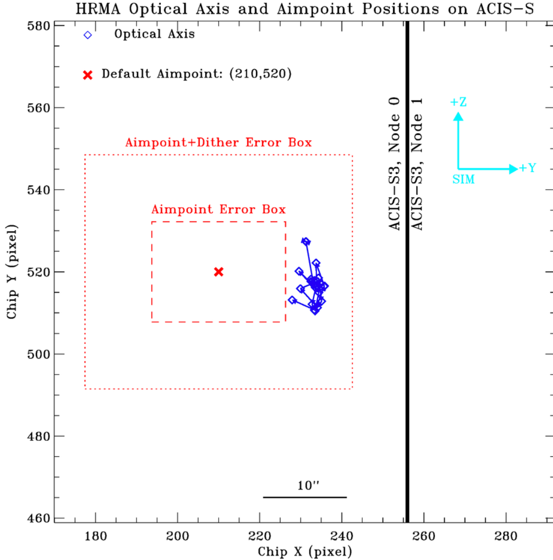
Figure 22: Chandra optical axis (blue diamonds) positions for each year and permanent default aimpoint (red cross) on ACIS-S at [210,520]. The small box (red dashed line, 16'' \times 12'' , or 32.5 \times 24.4 pixels) centered at the aimpoint is the error box of the aimpoint center, i.e. an on-axis target can be anywhere inside this box. The large box (red dotted line, 32'' \times 28'' , or 65.0 \times 56.9 pixels) is the error box of aimpoint with dither. Note the permanent default aimpoint is \sim 12'' from the optical axis in order to avoid the node boundary 0|1.
