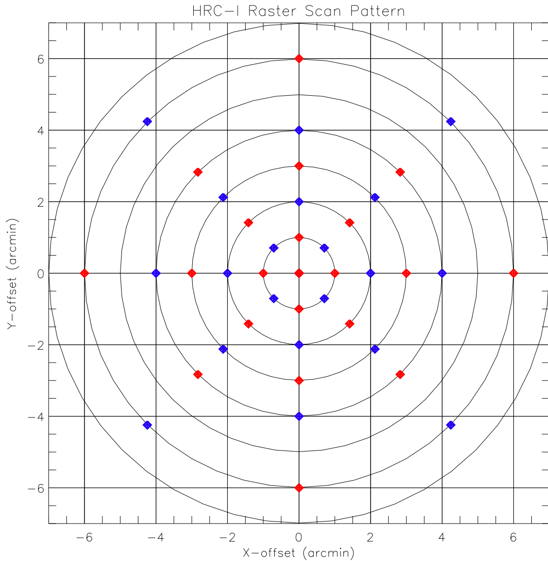
Figure 28: New raster scan pattern of HRC-I measurements of ArLac. The scan is divided into two groups and 21 and 20 observations each. The red dots indicate the first group; the blue dots indicate the second group.
