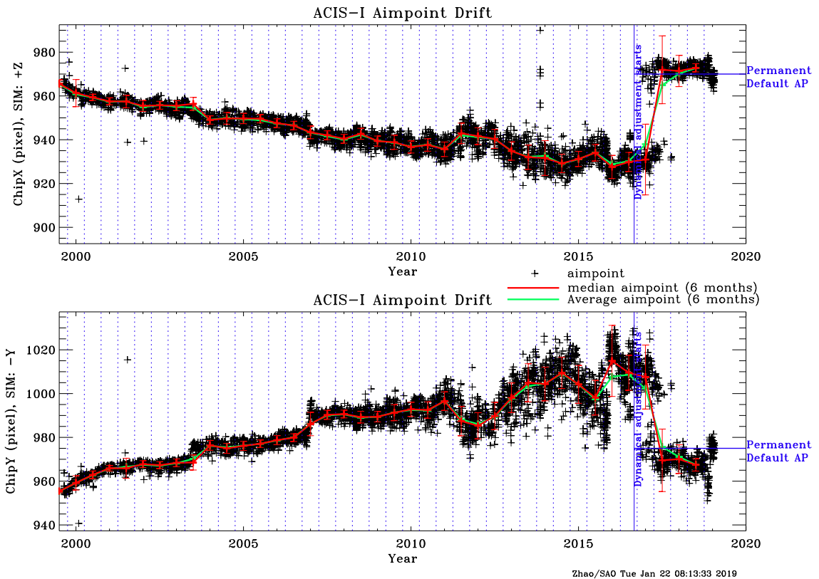
Figure 10: Aimpoint position as a function of time on ACIS-I since launch. Solid red (green) lines show the median (average) aimpoint drift in 6 month bins, separated by vertical dotted blue lines. The vertical solid blue line indicates the start of the dynamical aimpoint adjustment.
