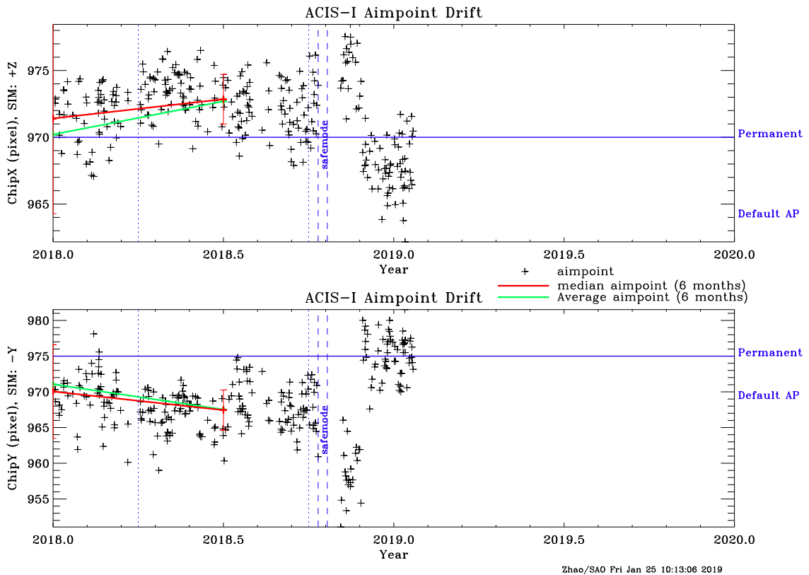
Figure 11: Aimpoint position as a function of time on ACIS-I in the past year. The gap between the two vertical dashed lines indicate when Chandra was in safemode (Oct. 10–21, 2018).
