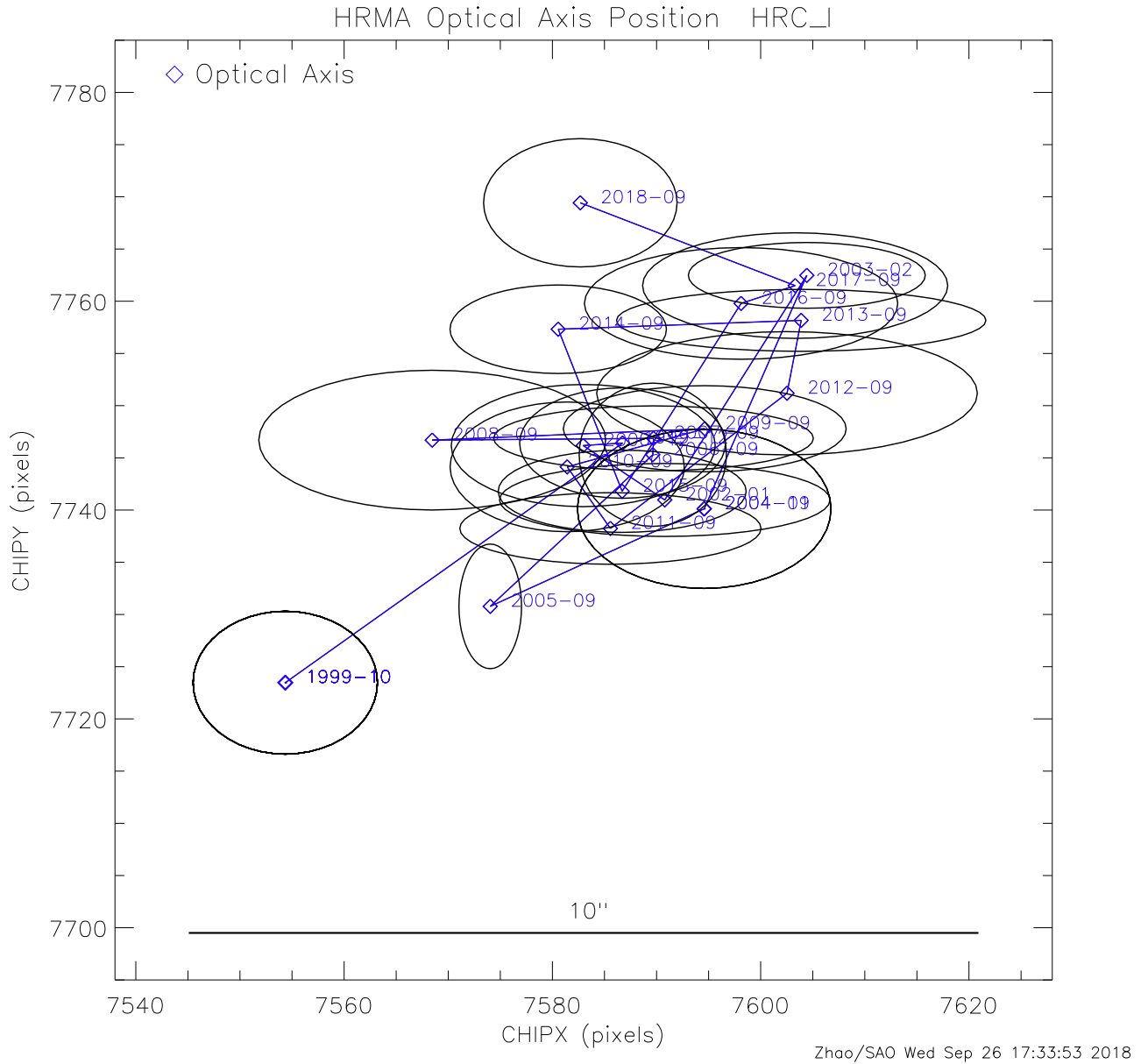
Figure 5: Chandra optical axis positions on HRC-I since launch. Each position is labeled by the year-month. The ellipse around each position is the 1 - \sigma measurement error ellipse for that given year. The drift of optical axis position is consistent with the measurement errors. The optical axis position is very stable and well within a 10'' region. Since year 2000, the optical axis drift was well within a 6'' region.
