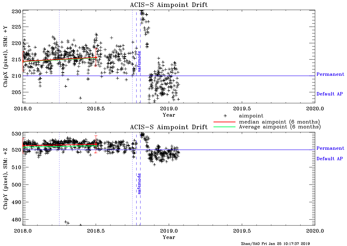
Figure 13: Aimpoint position as a function of time on ACIS-S in the past year. The gap between the two vertical dashed lines indicate when Chandra was in safemode (Oct. 10–21, 2018).
