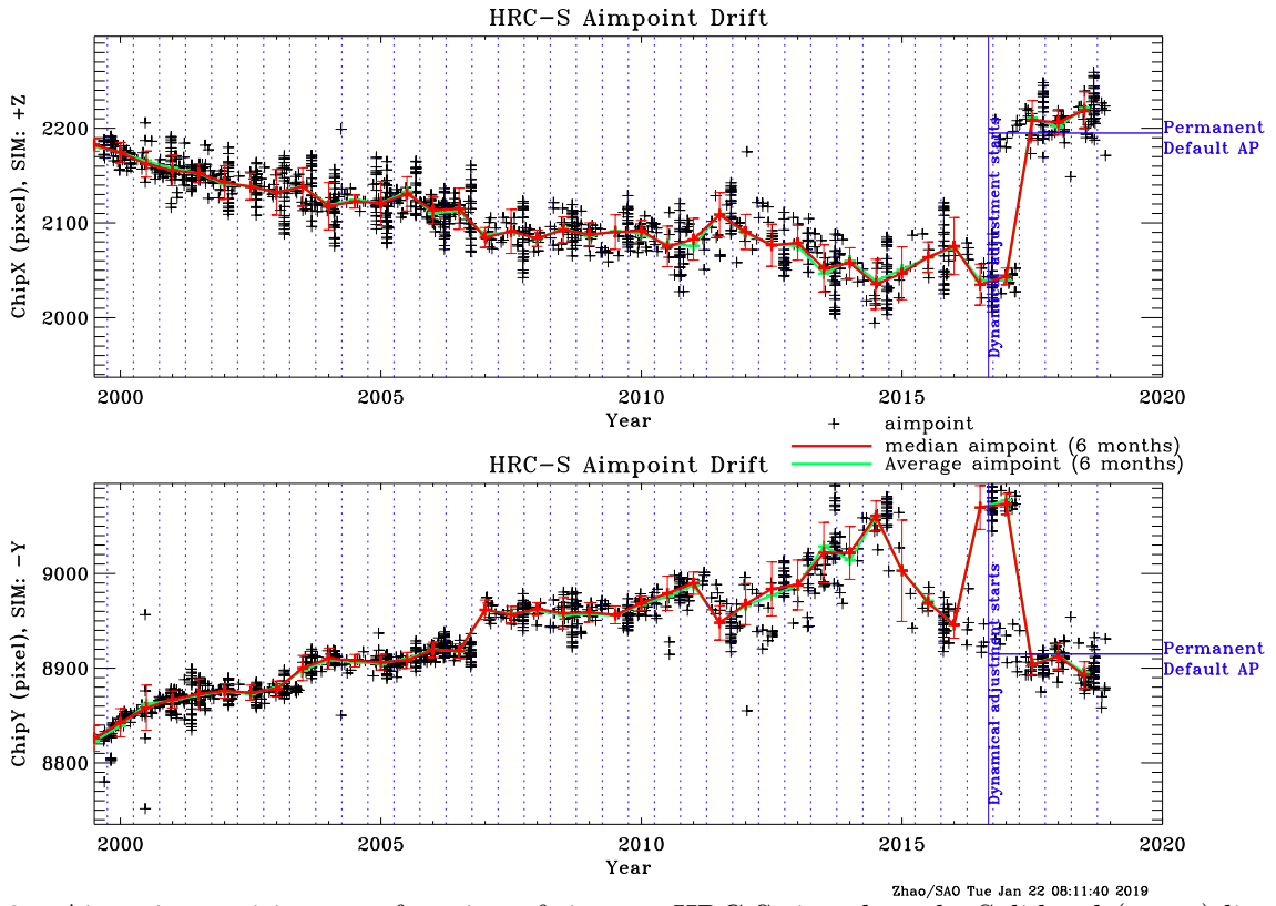
Figure 8: Aimpoint position as a function of time on HRC-S since launch. Solid red (green) lines show the median (average) aimpoint drift in 6 month bins, separated by vertical dotted blue lines. The vertical solid blue line indicates the start of the dynamical aimpoint adjustment.
