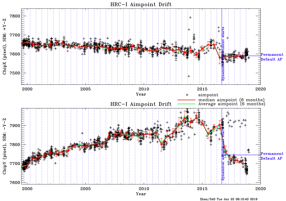
Figure 6: Aimpoint position as a function of time on HRC-I since launch. Solid red (green) lines show the median (average) aimpoint drift in 6 month bins, separated by vertical dotted blue lines. The vertical solid blue line indicates the start of the dynamical aimpoint adjustment.
