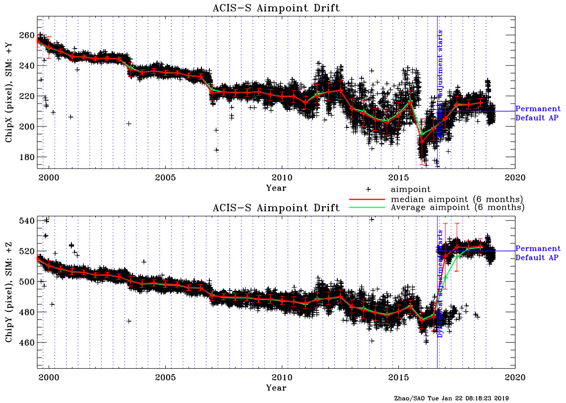
Figure 12: Aimpoint position as a function of time on ACIS-S since launch. Solid red (green) lines show the median (average) aimpoint drift in 6 month bins, separated by vertical dotted blue lines. The vertical solid blue line indicates the start of the dynamical aimpoint adjustment.
