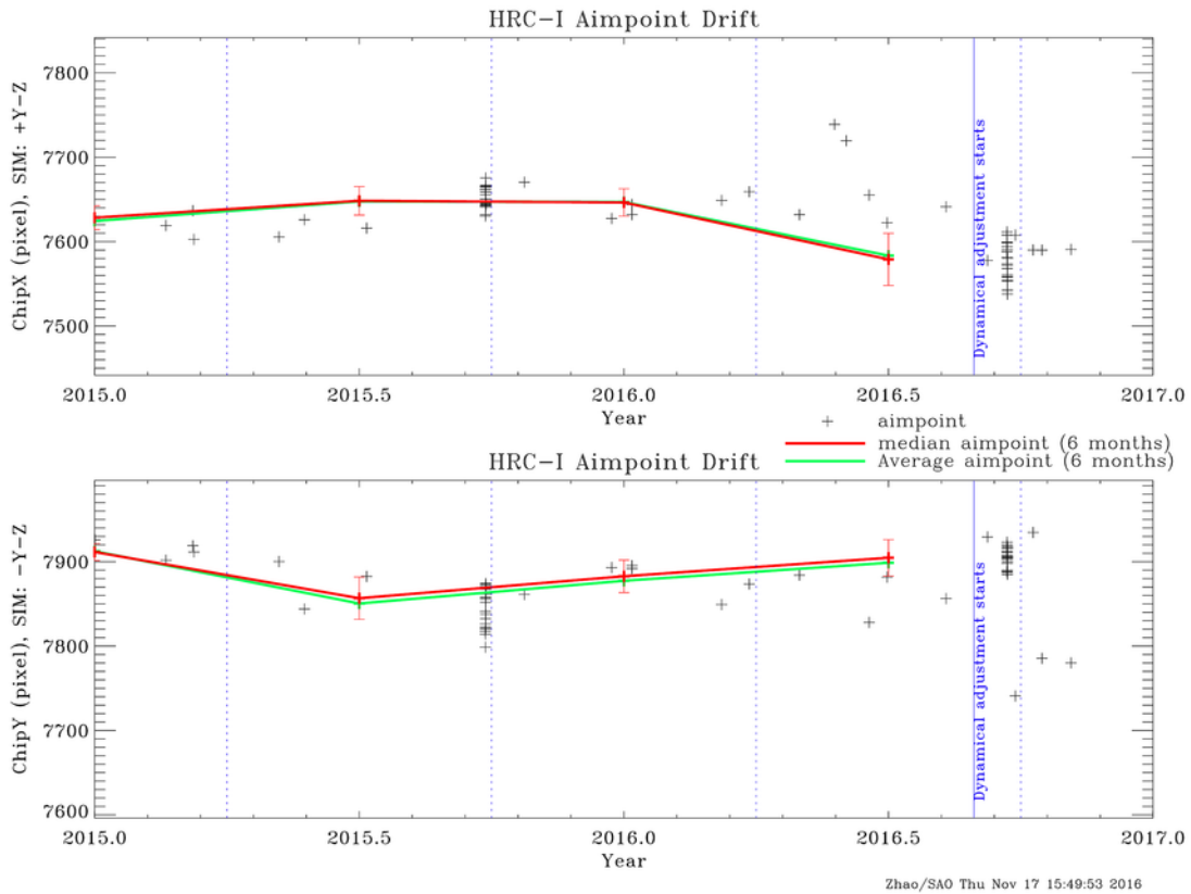
Figure 7: Aimpoint position as a function of time on HRC-I in the past two years. The vertical solid blue line indicates the start of the dynamical aimpoint adjustment.
