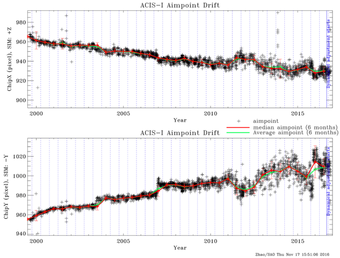
Figure 10: Aimpoint position as a function of time on ACIS-I since launch. Solid red (green) lines show the median (average) aimpoint drift in 6 months bins, separated by vertical dotted blue lines.
