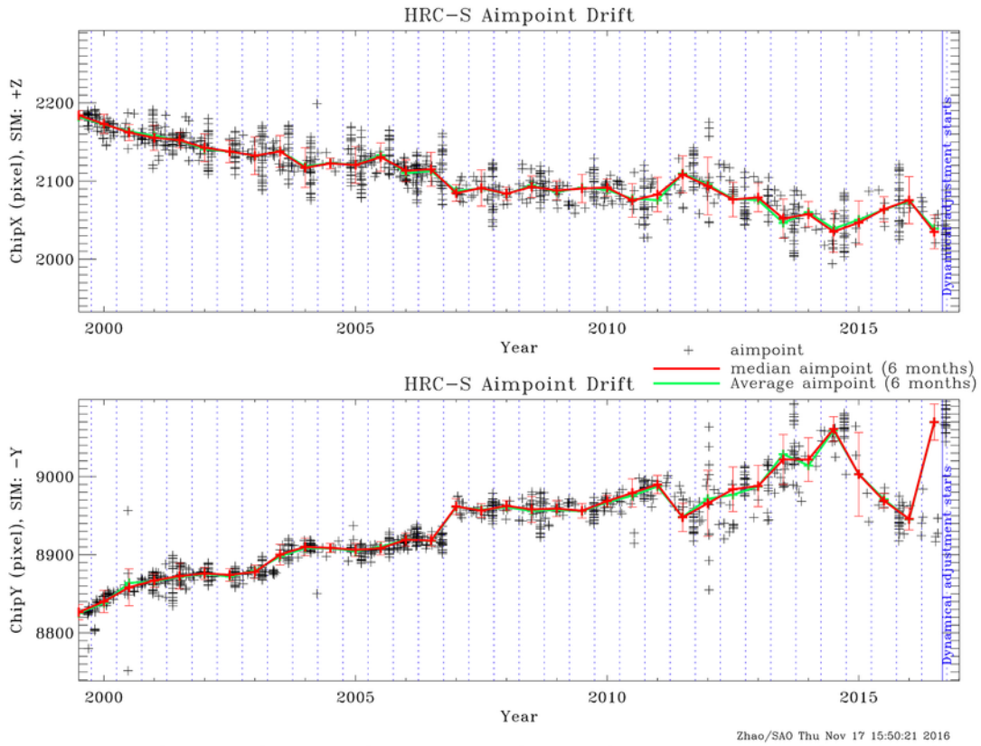
Figure 8: Aimpoint position as a function of time on HRC-S since launch. Solid red (green) lines show the median (average) aimpoint drift in 6 months bins, separated by vertical dotted blue lines.
