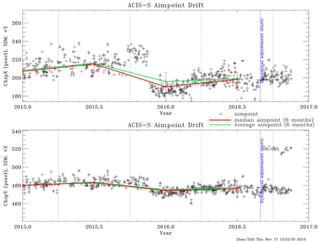
Figure 13: Aimpoint position as a function of time on ACIS-S in the past two years. The vertical solid blue line indicates the start of the dynamical aimpoint adjustment.
