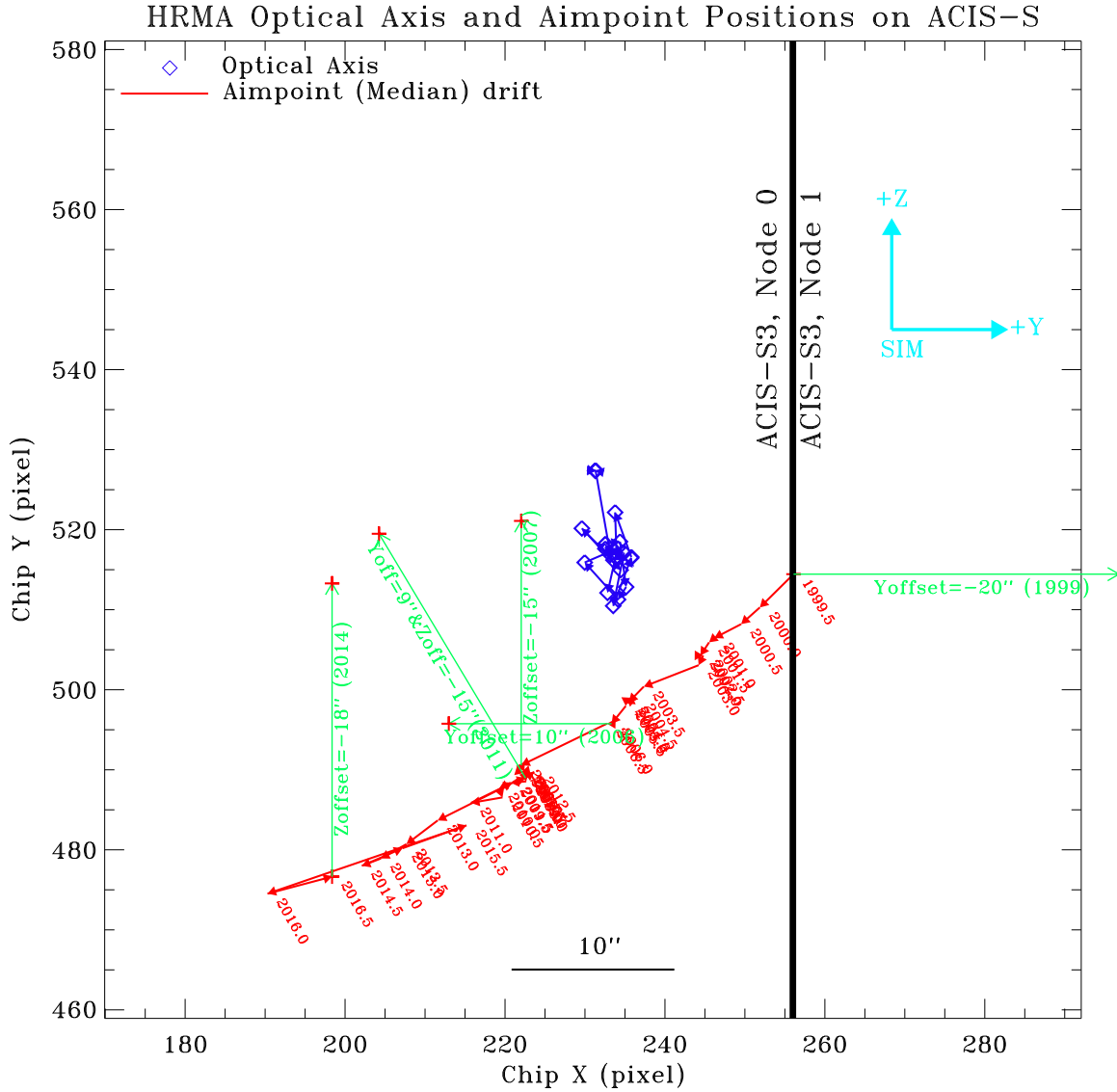
Figure 17: Chandra optical axis (blue) and median aimpoint (red, see Fig. 12) positions in half year bins on ACIS-S. Each aimpoint position is labeled by the year. The cyan colored arrows show the SIM coordinates. The green arrows show the default offsets implemented over the years (see Section 6 for more details). The last default offset was Y-offset = 0" and Z-offset = -18", implemented in December 2013, until the permanent default aimpoint was implemented in Cycle 18. All the ACIS-S observations were conducted with these default offsets starting in the year labels next to the green arrows, unless the observers requested otherwise.
