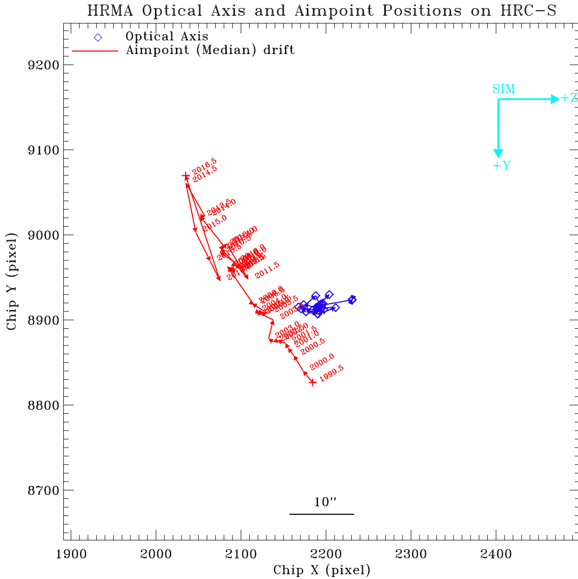
Figure 15: Chandra optical axis (blue) and median aimpoint (red, see Fig. 8) positions in half year bins on HRC-S. Each aimpoint position is labeled by the year. The cyan colored arrows show the SIM coordinates.
