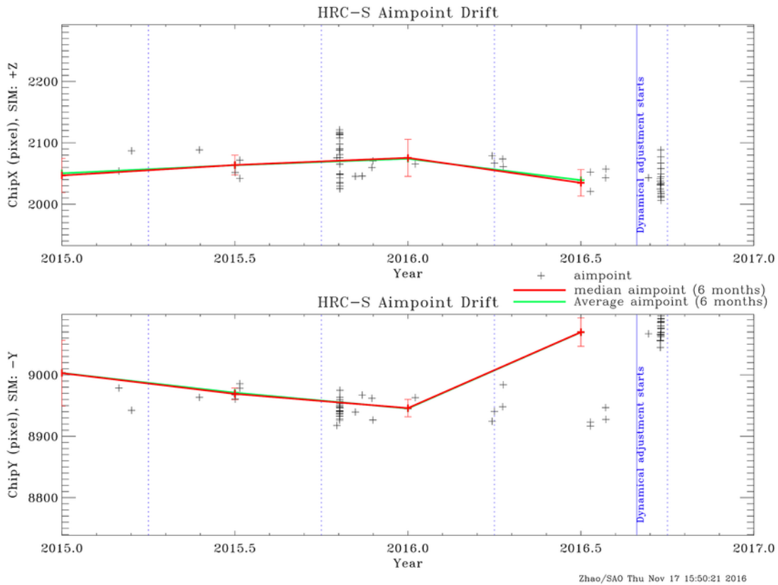
Figure 9: Aimpoint position as a function of time on HRC-S in the past two years. The vertical solid blue line indicates the start of the dynamical aimpoint adjustment.
