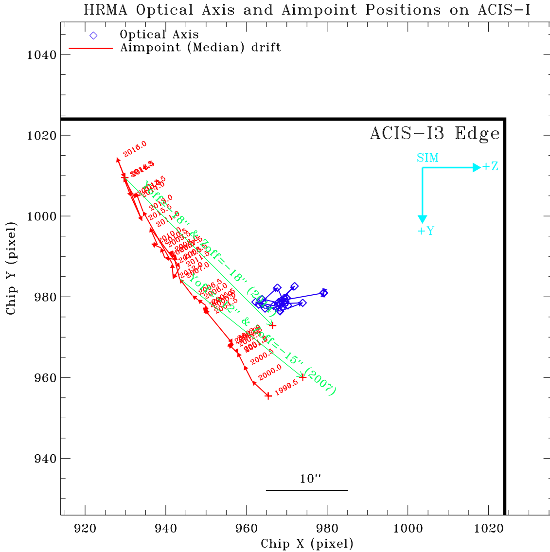
Figure 16: Chandra optical axis (blue) and median aimpoint (red, see Fig. 10) positions in half year bins on ACIS-I. Each aimpoint position is labeled by the year. The cyan colored arrows show the SIM coordinates. ACIS-I observations were conducted without default offset from the Chandra launch until the end of 2006. In December 2006, the aimpoint had a sudden shift of \sim 10'' due to the ACA primary focal plan CCD cool down from -15^\circ\text{C} to -20^\circ\text{C} . This sudden shift brought the aimpoint uncomfortably close to the ACIS-I3 chip edge. As it continue to drift towards the edge, the dither pattern ( 16'' peak-to-peak) will soon fall out of the chip. Therefore a default Y-offset = -15'' and Z-offset = -12'' was implemented to move the aimpoint away from the chip edge and also closer to the optical axis. Due to its accelerated drift since early 2012, the aimpoint was once again very close to the ACIS-I3 edge in late 2013. So since December 2013, a new default offset of Y-offset = -18'' and Z-offset = -18'' was applied, until the permanent default aimpoint was implemented in Cycle 18. The two green arrows in the figure show the magnitude and the direction of the default offsets. All the ACIS-I observations were conducted with these default offsets starting in the year labels next to the green arrows, unless the observers requested otherwise.
