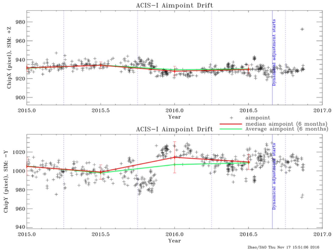
Figure 11: Aimpoint position as a function of time on ACIS-I in the past two years. The vertical solid blue line indicates the start of the dynamical aimpoint adjustment.
