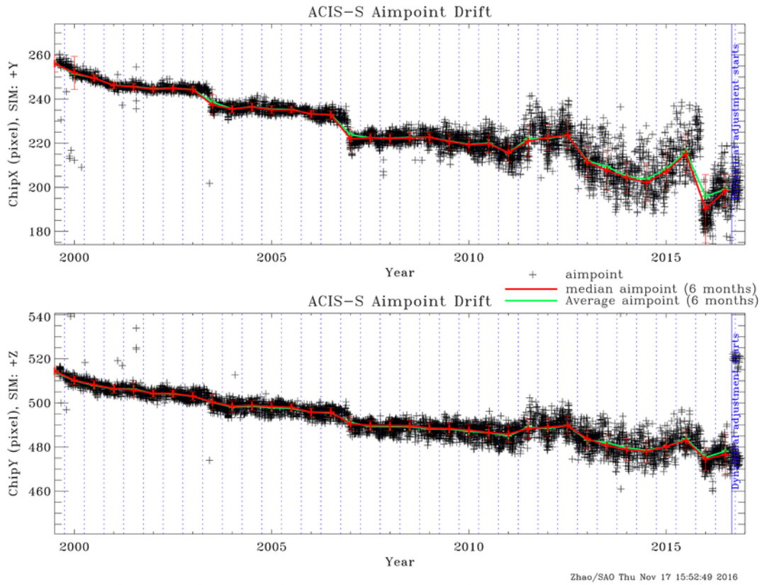
Figure 12: Aimpoint position as a function of time on ACIS-S since launch. Solid red (green) lines show the median (average) aimpoint drift in 6 months bins, separated by vertical dotted blue lines.
