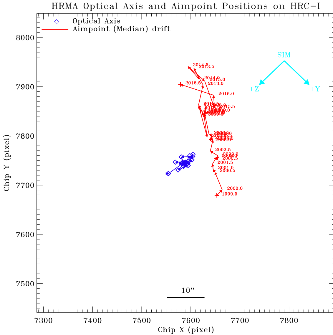
Figure 14: Chandra optical axis (blue) and median aimpoint (red, see Fig. 6) positions in half year bins on HRC-I. Each aimpoint position is labeled by the year. The cyan colored arrows show the SIM coordinates.
