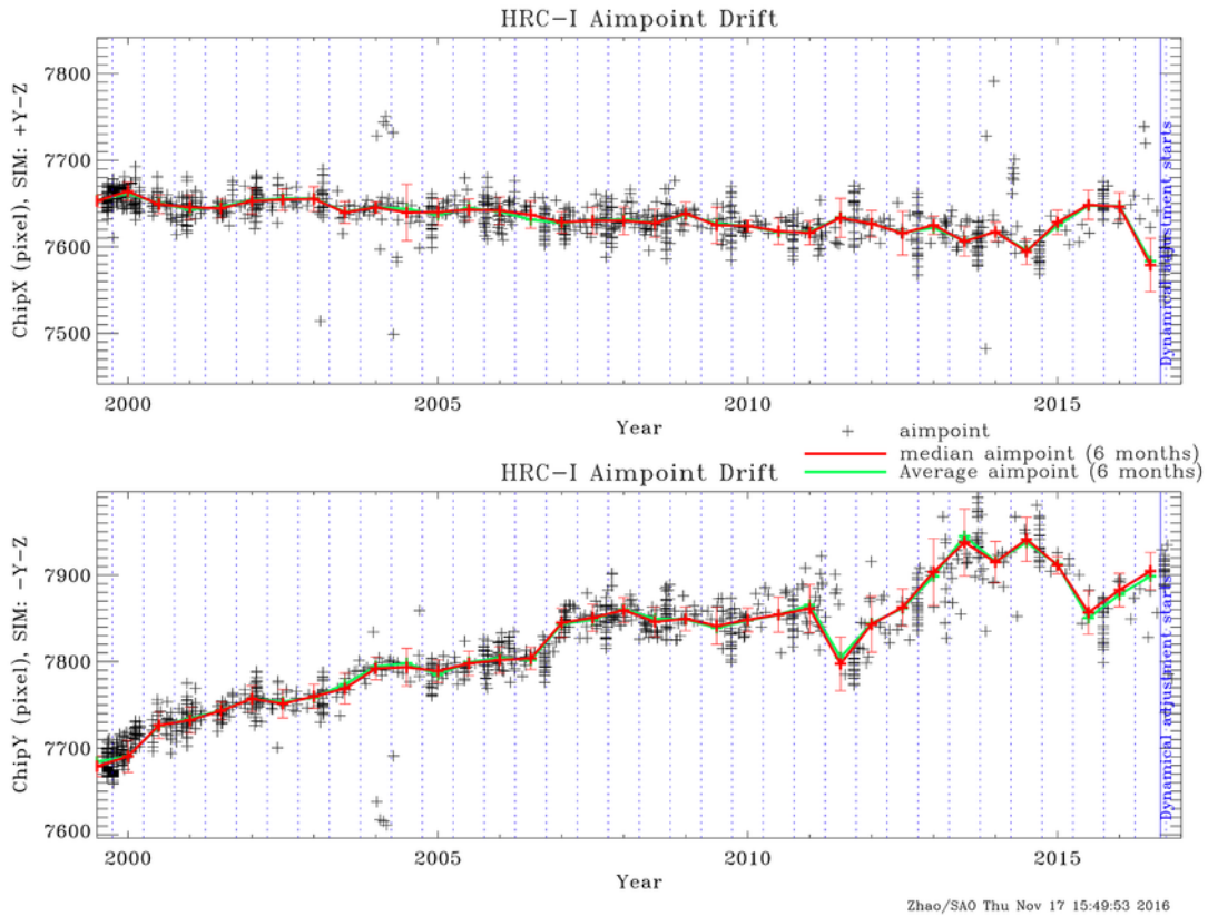
Figure 6: Aimpoint position as a function of time on HRC-I since launch. Solid red (green) lines show the median (average) aimpoint drift in 6 months bins, separated by vertical dotted blue lines.
